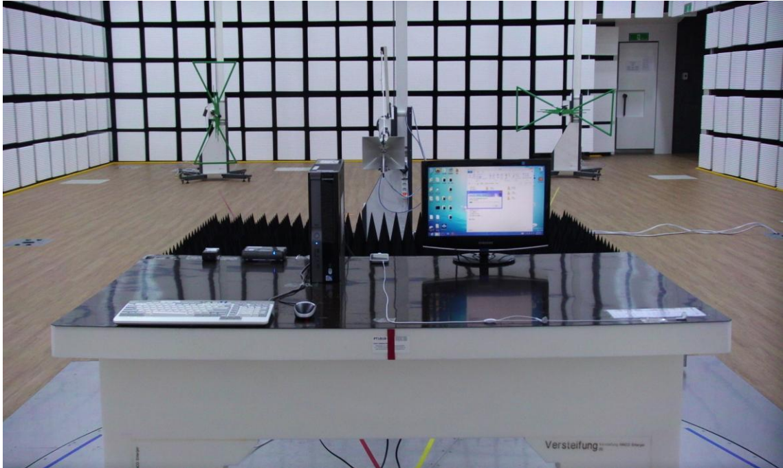
[ Radiated Disturbance for Above 1 GHz – Front ]
