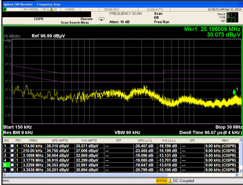
Plot 6-29. Line Conducted Plot with Bluetooth LE (N)
