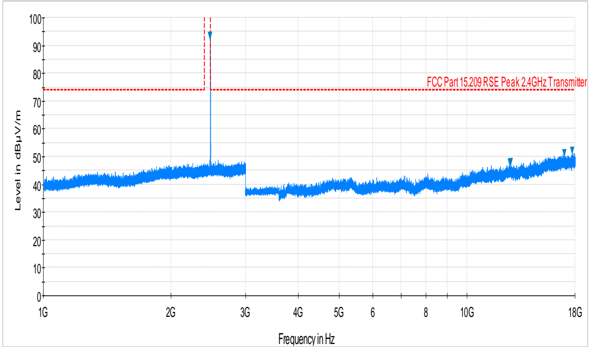
Plot 6-22. Radiated Spurious Plot above 1GHz (Bluetooth LE – Ch. 39, Ant. Pol. H)
