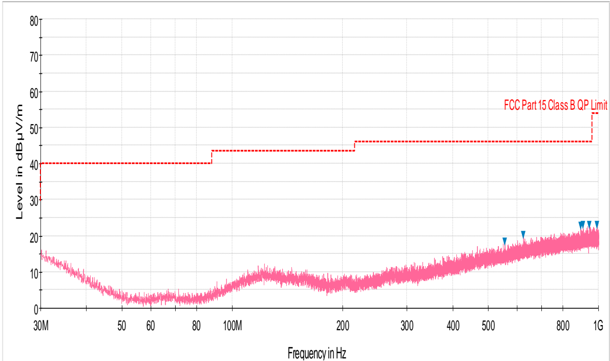
Plot 6-24. Radiated Spurious Plot below 1GHz (Pol. H)
