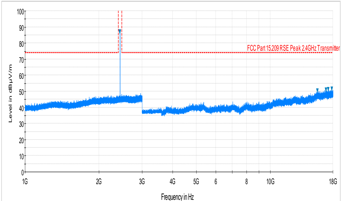
Plot 6-21. Radiated Spurious Plot above 1GHz (Bluetooth LE – Ch. 19, Ant. Pol. V)
