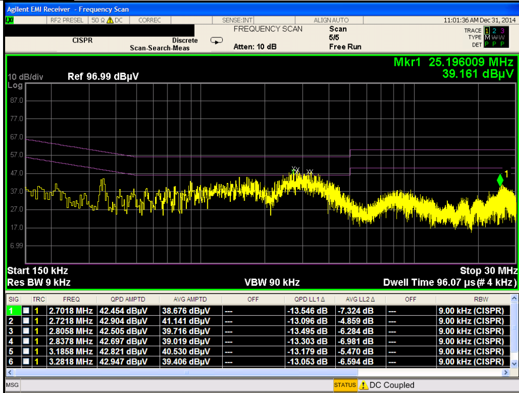
Plot 6-28. Line Conducted Plot with Bluetooth LE (L1)
