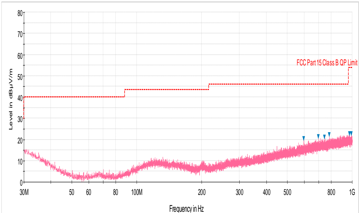
Plot 6-25. Radiated Spurious Plot below 1GHz (Pol. V)
