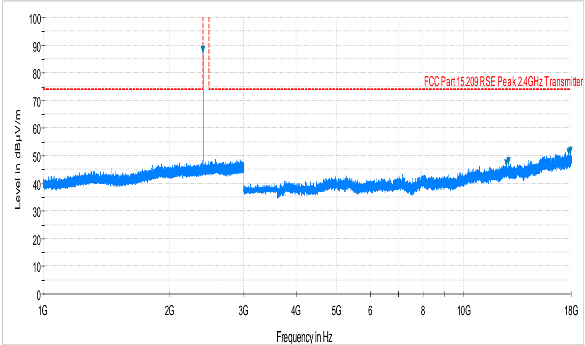
Plot 6-18. Radiated Spurious Plot above 1GHz (Bluetooth LE – Ch. 0, Ant. Pol. H)
