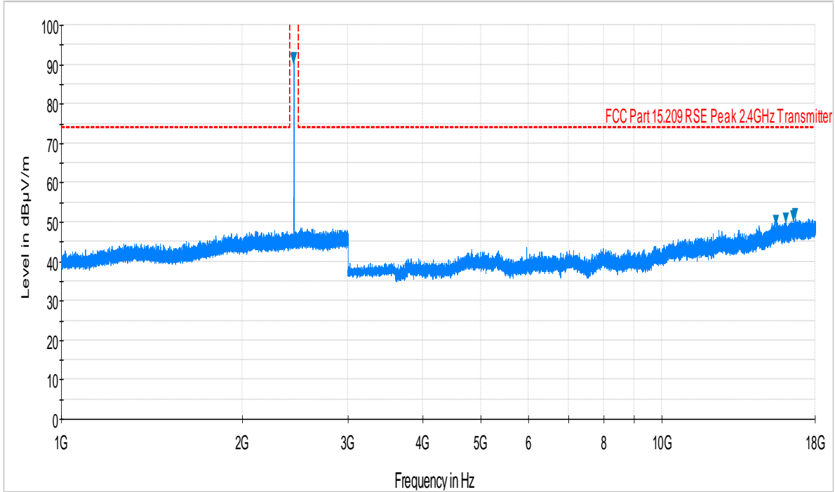
Plot 6-20. Radiated Spurious Plot above 1GHz (Bluetooth LE – Ch. 19, Ant. Pol. H)
