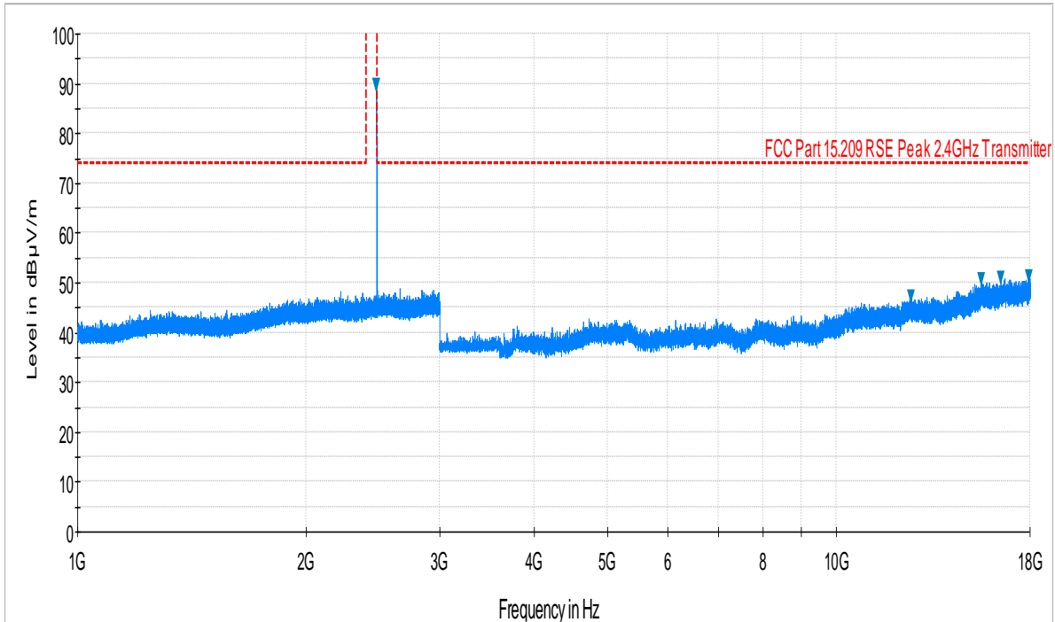
Plot 6-23. Radiated Spurious Plot above 1GHz (Bluetooth LE – Ch. 39, Ant. Pol. V)
