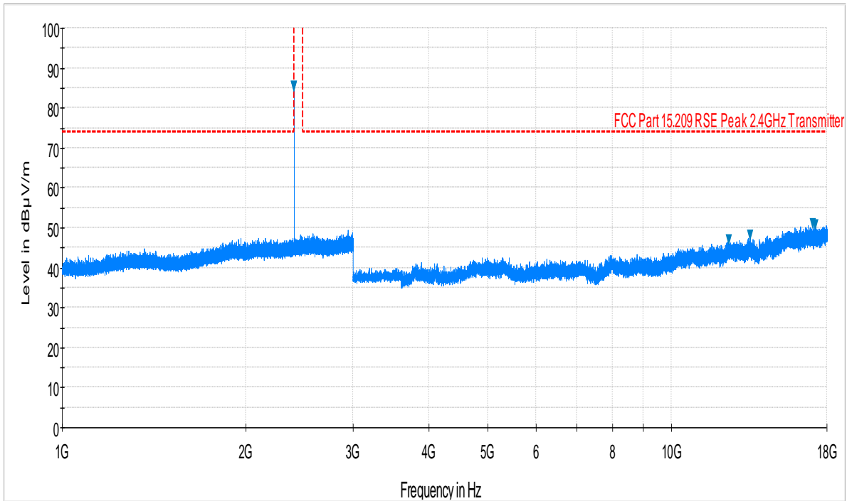
Plot 6-19. Radiated Spurious Plot above 1GHz (Bluetooth LE – Ch. 0, Ant. Pol. V)
