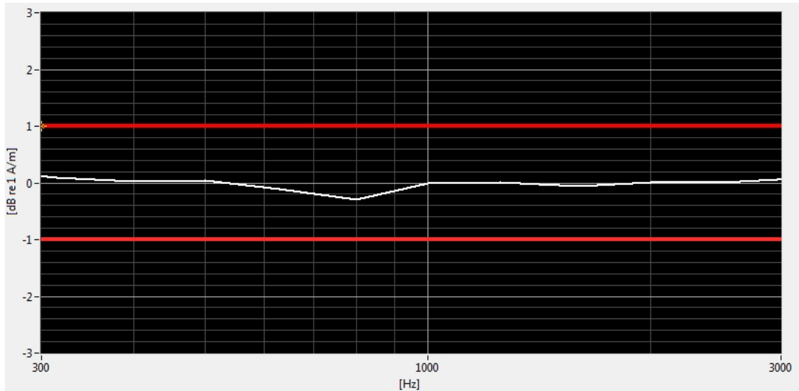
Figure 6-4 Helmholtz Coil Validation for Frequency Response
