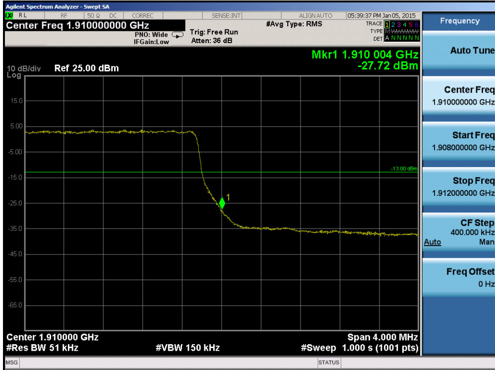
Plot 6-91. Upper Band Edge Plot (Band 2 – 5.0MHz QPSK – RB Size 25)
