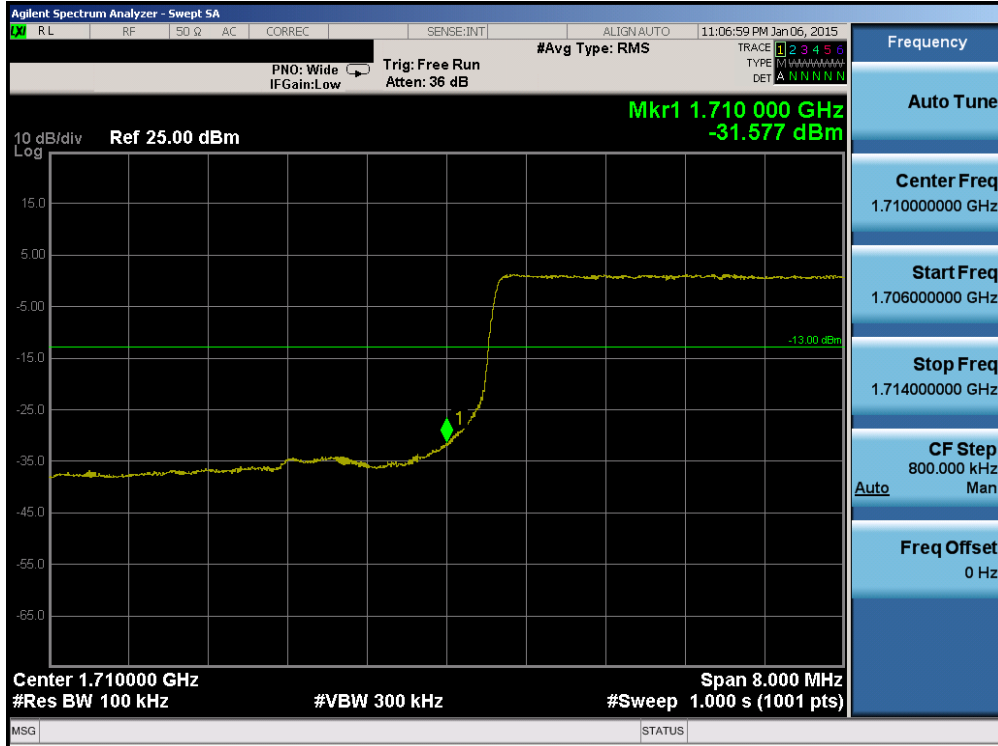
Plot 6-69. Lower Band Edge Plot (Band 4 – 10.0MHz QPSK – RB Size 50)
