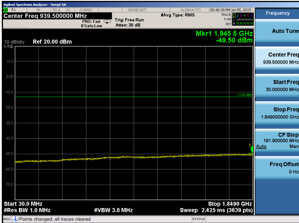
Plot 6-40. Conducted Spurious Plot (Band 2 – 10.0MHz QPSK – RB Size 1, RB Offset 0 – Mid Channel)
