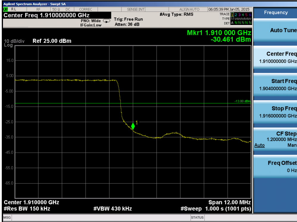
Plot 6-99. Upper Band Edge Plot (Band 2 – 15.0MHz QPSK – RB Size 75)
