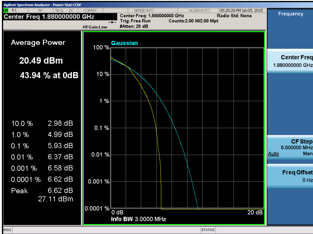
Plot 6-108. PAR Plot (Band 2 – 3.0MHz 16-QAM – RB Size 15)
