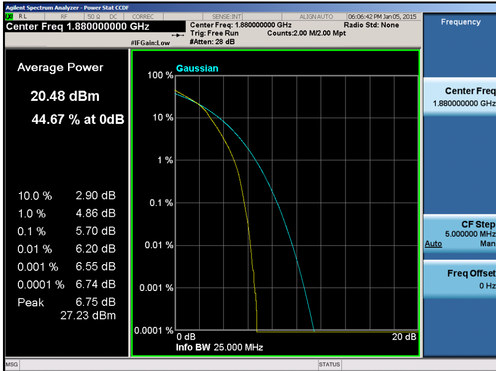
Plot 6-116. PAR Plot (Band 2 – 20.0MHz 16-QAM – RB Size 100)
