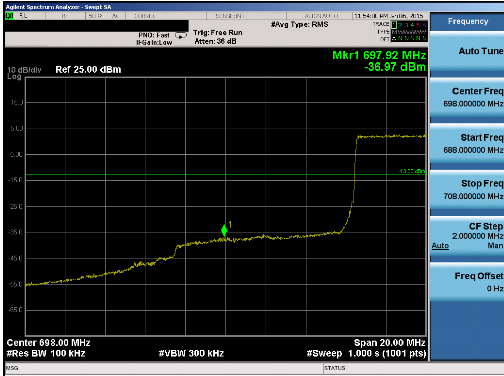
Plot 6-47. Lower Band Edge Plot (Band 17 – 10.0MHz QPSK – RB Size 50)
