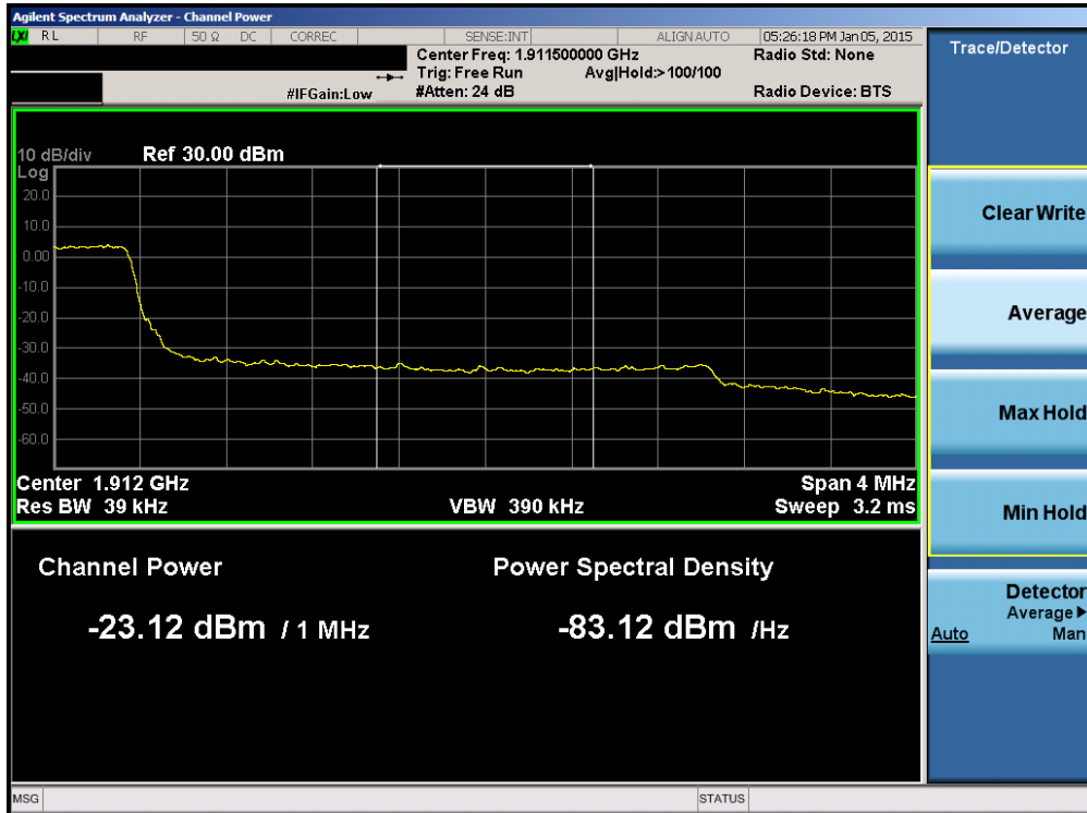
Plot 6-88. Upper Extended Band Edge Plot (Band 2 – 3.0MHz QPSK – RB Size 15)
