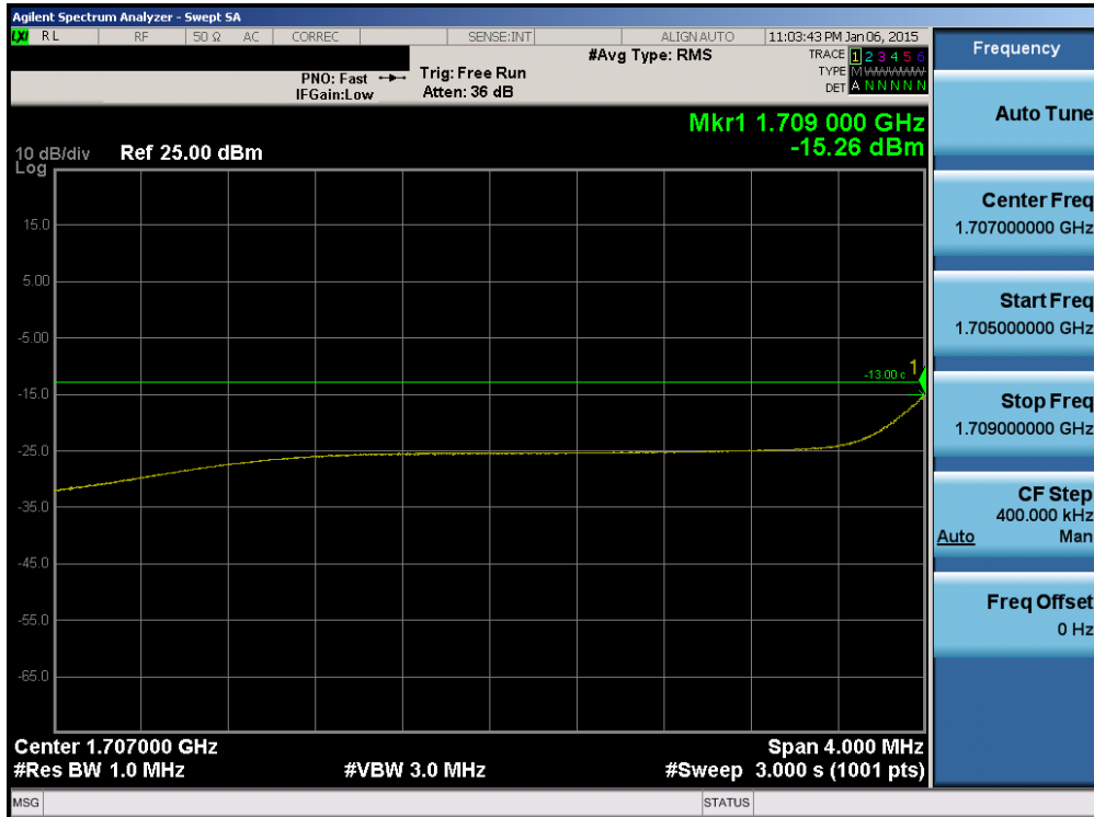
Plot 6-66. Lower Extended Band Edge Plot (Band 4 – 5.0MHz QPSK – RB Size 25)
