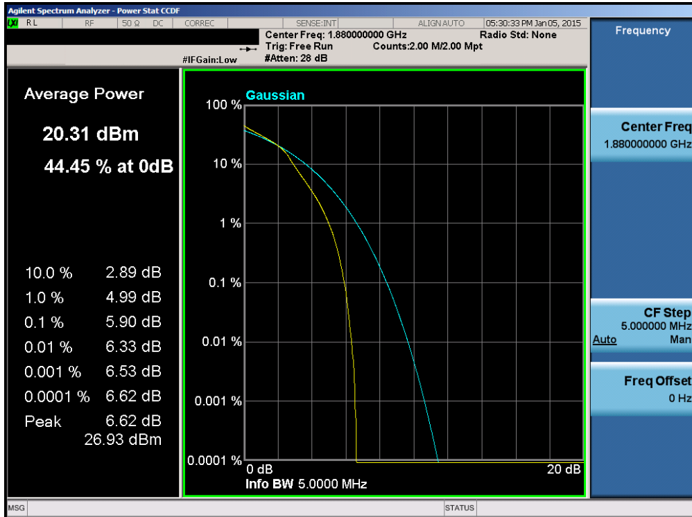
Plot 6-110. PAR Plot (Band 2 – 5.0MHz 16-QAM – RB Size 25)
