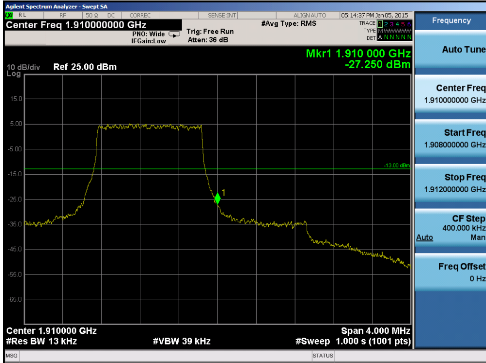
Plot 6-83. Upper Band Edge Plot (Band 2 – 1.4MHz QPSK – RB Size 6)
