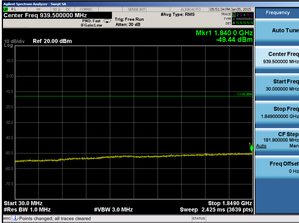
Plot 6-43. Conducted Spurious Plot (Band 2 – 10.0MHz QPSK – RB Size 1, RB Offset 0 – High Channel)
