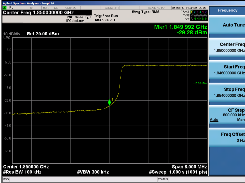
Plot 6-93. Lower Band Edge Plot (Band 2 – 10.0MHz QPSK – RB Size 50)
