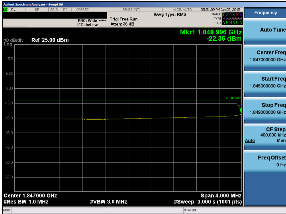
Plot 6-94. Lower Extended Band Edge Plot (Band 2 – 10.0MHz QPSK – RB Size 50)
