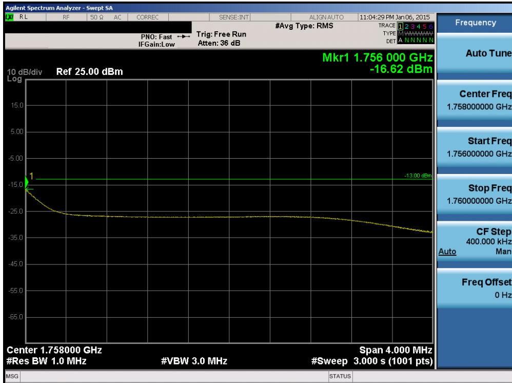
Plot 6-68. Upper Extended Band Edge Plot (Band 4 – 5.0MHz QPSK – RB Size 25)
