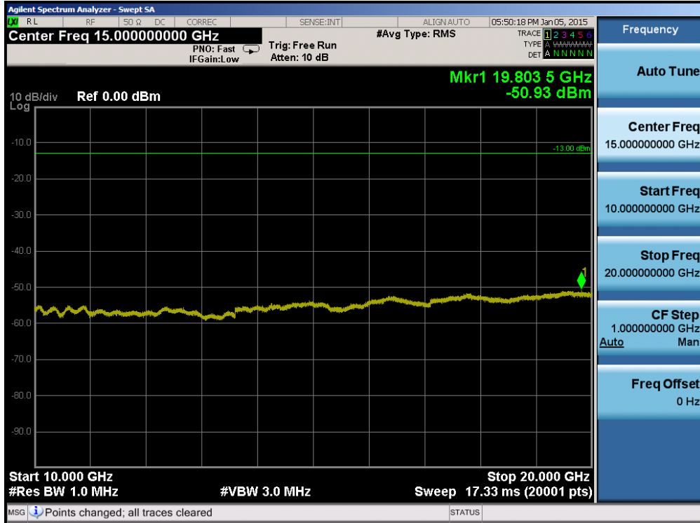
Plot 6-39. Conducted Spurious Plot (Band 2 – 10.0MHz QPSK – RB Size 1, RB Offset 0 – Low Channel)
