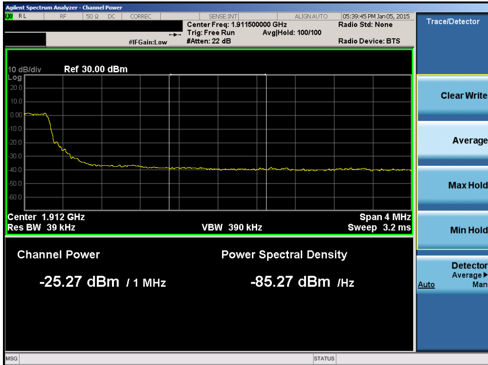
Plot 6-92. Upper Extended Band Edge Plot (Band 2 – 5.0MHz QPSK – RB Size 25)
