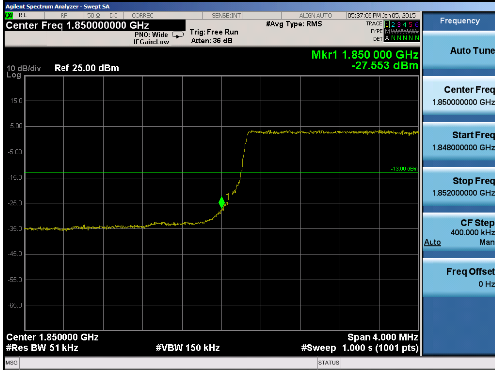
Plot 6-89. Lower Band Edge Plot (Band 2 – 5.0MHz QPSK – RB Size 25)
