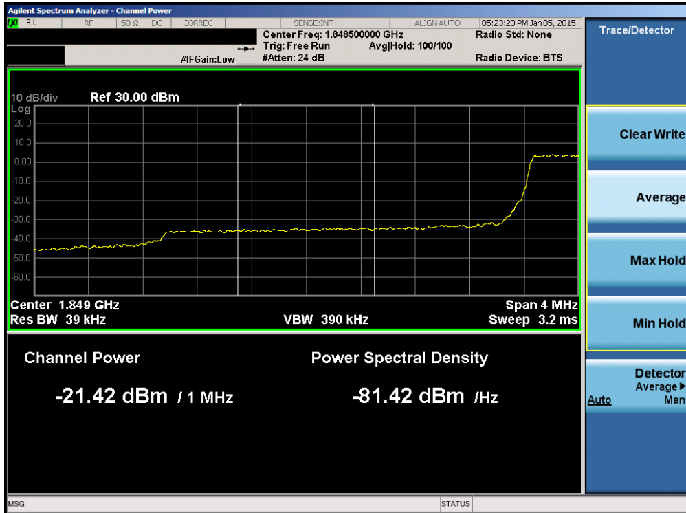
Plot 6-86. Lower Extended Band Edge Plot (Band 2 – 3.0MHz QPSK – RB Size 15)
