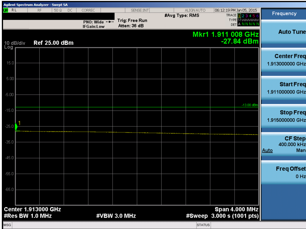
Plot 6-104. Upper Extended Band Edge Plot (Band 2 – 20.0MHz QPSK – RB Size 100)
