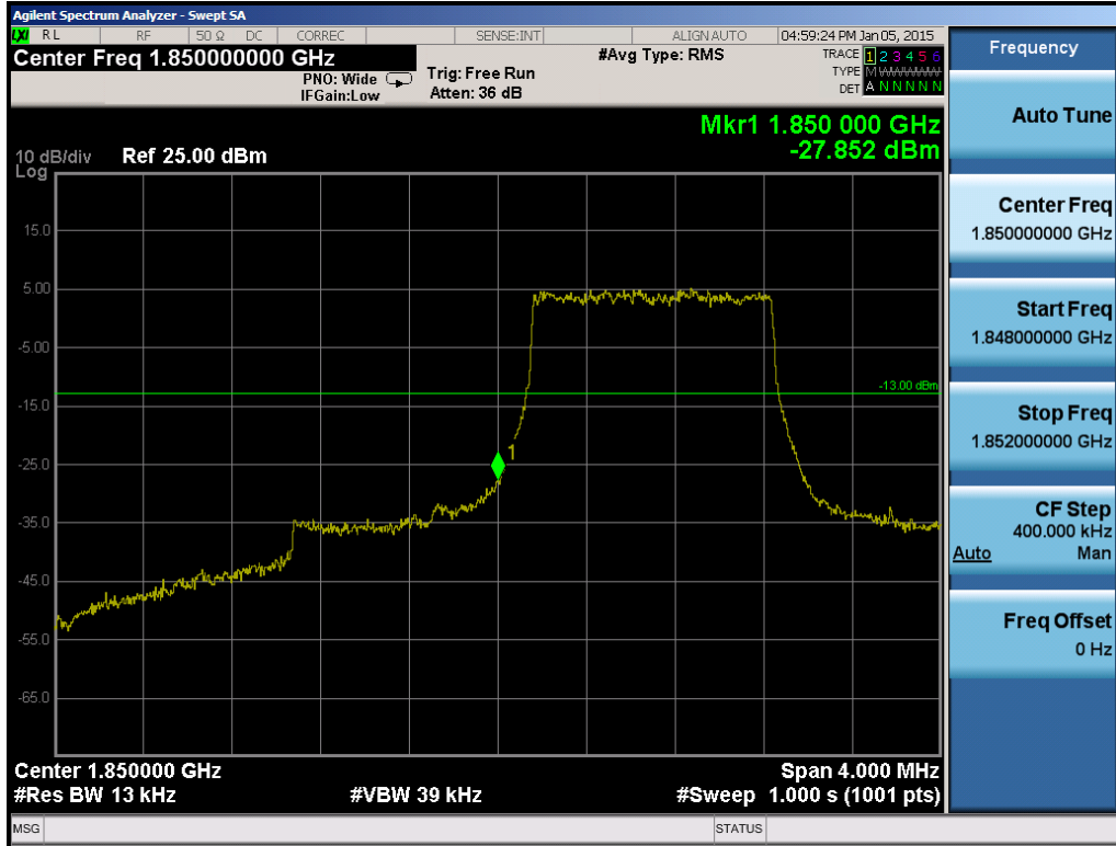
Plot 6-81. Lower Band Edge Plot (Band 2 – 1.4MHz QPSK – RB Size 6)
