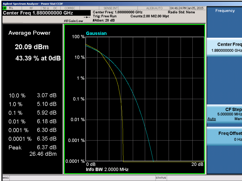
Plot 6-106. PAR Plot (Band 2 – 1.4MHz 16-QAM – RB Size 6)
