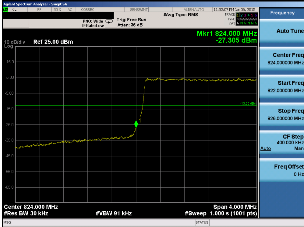
Plot 6-51. Lower Band Edge Plot (Band 5 – 3.0MHz QPSK – RB Size 15)
