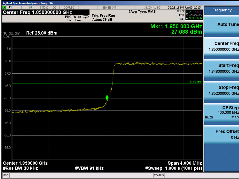
Plot 6-85. Lower Band Edge Plot (Band 2 – 3.0MHz QPSK – RB Size 15)
