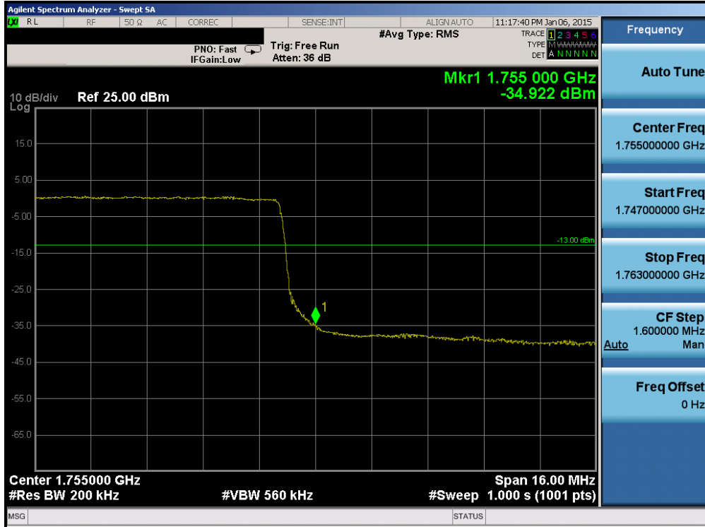
Plot 6-79. Upper Band Edge Plot (Band 4 – 20.0MHz QPSK – RB Size 100)
