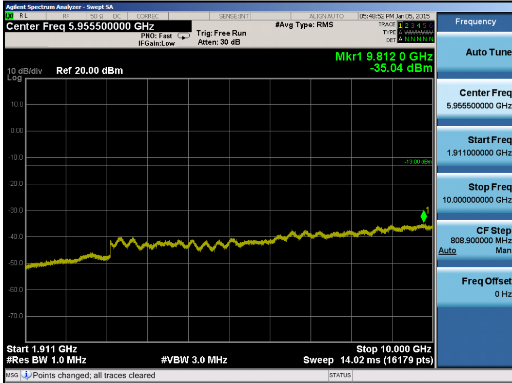
Plot 6-41. Conducted Spurious Plot (Band 2 – 10.0MHz QPSK – RB Size 1, RB Offset 0 – Mid Channel)
