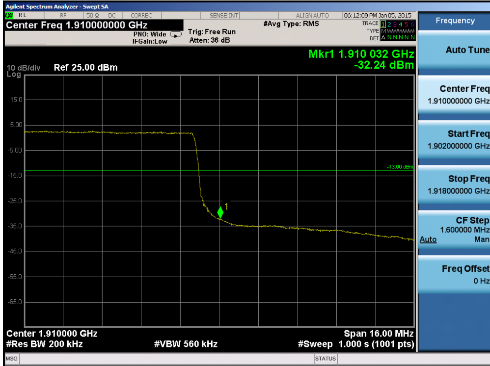
Plot 6-103. Upper Band Edge Plot (Band 2 – 20.0MHz QPSK – RB Size 100)
