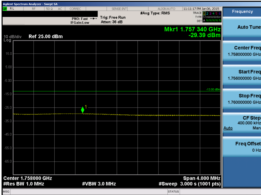
Plot 6-76. Upper Extended Band Edge Plot (Band 4 – 15.0MHz QPSK – RB Size 75)
