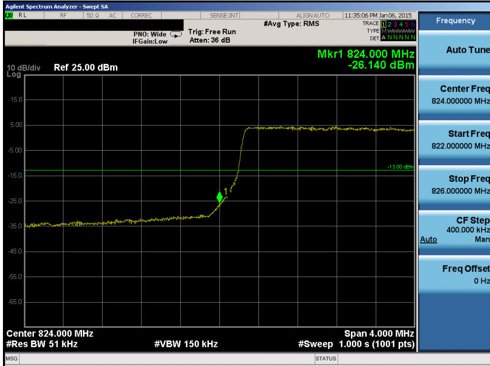
Plot 6-53. Lower Band Edge Plot (Band 5 – 5.0MHz QPSK – RB Size 25)
