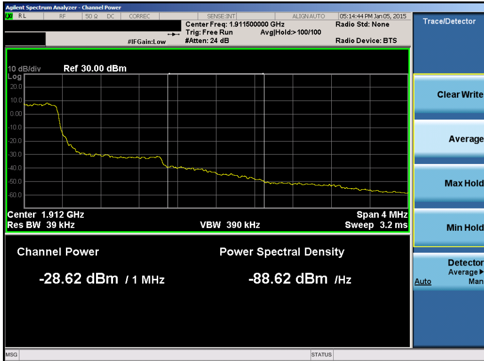
Plot 6-84. Upper Extended Band Edge Plot (Band 2 – 1.4MHz QPSK – RB Size 6)
