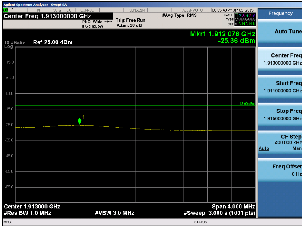
Plot 6-100. Upper Extended Band Edge Plot (Band 2 – 15.0MHz QPSK – RB Size 75)
