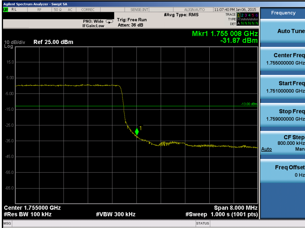
Plot 6-71. Upper Band Edge Plot (Band 4 – 10.0MHz QPSK – RB Size 50)
