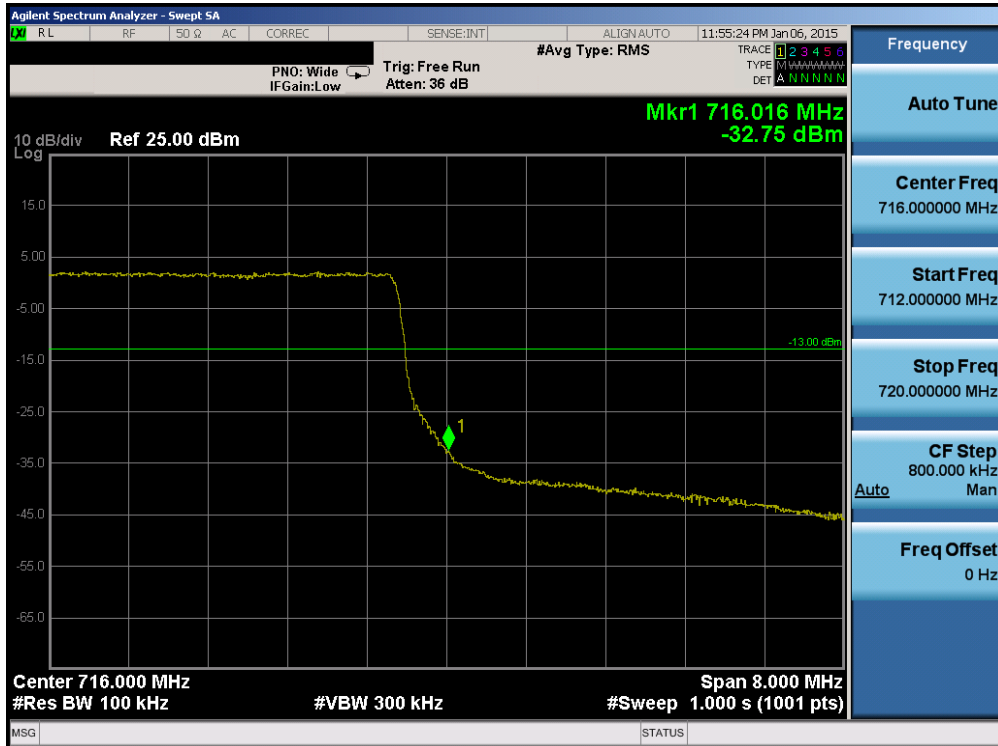
Plot 6-48. Upper Band Edge Plot (Band 17 – 10.0MHz QPSK – RB Size 50)
