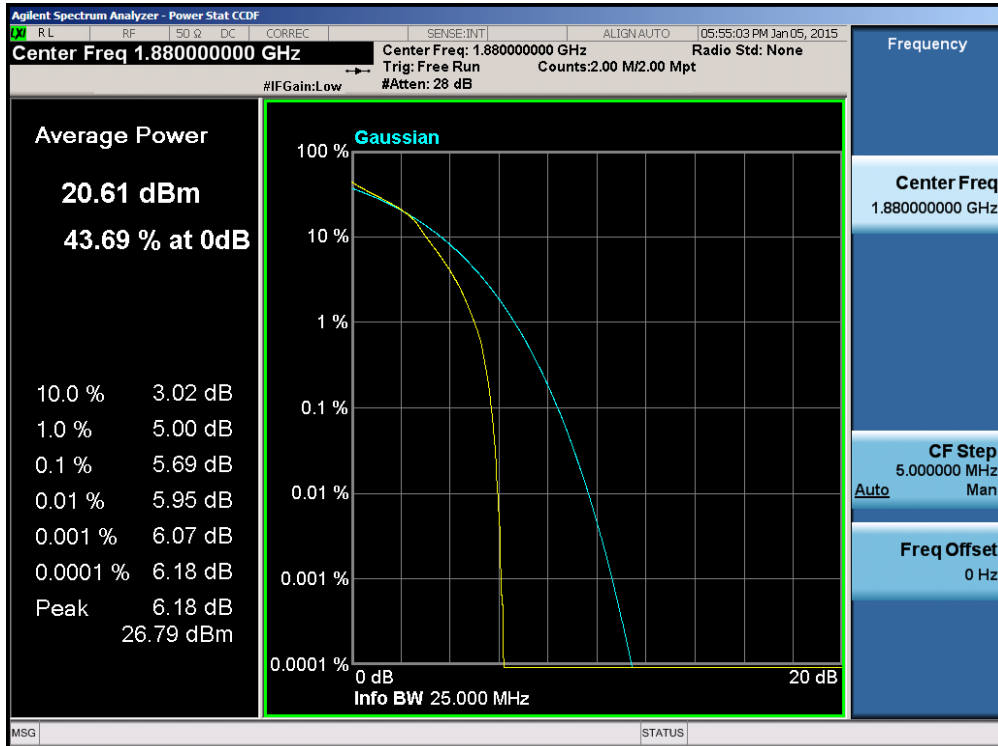
Plot 6-114. PAR Plot (Band 2 – 15.0MHz 16-QAM – RB Size 75)
