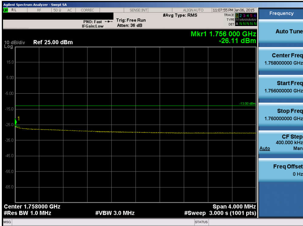
Plot 6-72. Upper Extended Band Edge Plot (Band 4 – 10.0MHz QPSK – RB Size 50)
