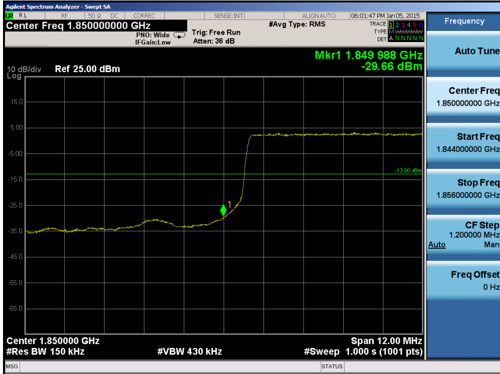
Plot 6-97. Lower Band Edge Plot (Band 2 – 15.0MHz QPSK – RB Size 75)
