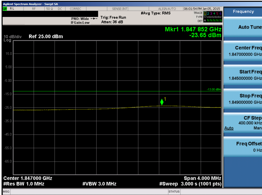
Plot 6-98. Lower Extended Band Edge Plot (Band 2 – 15.0MHz QPSK – RB Size 75)
