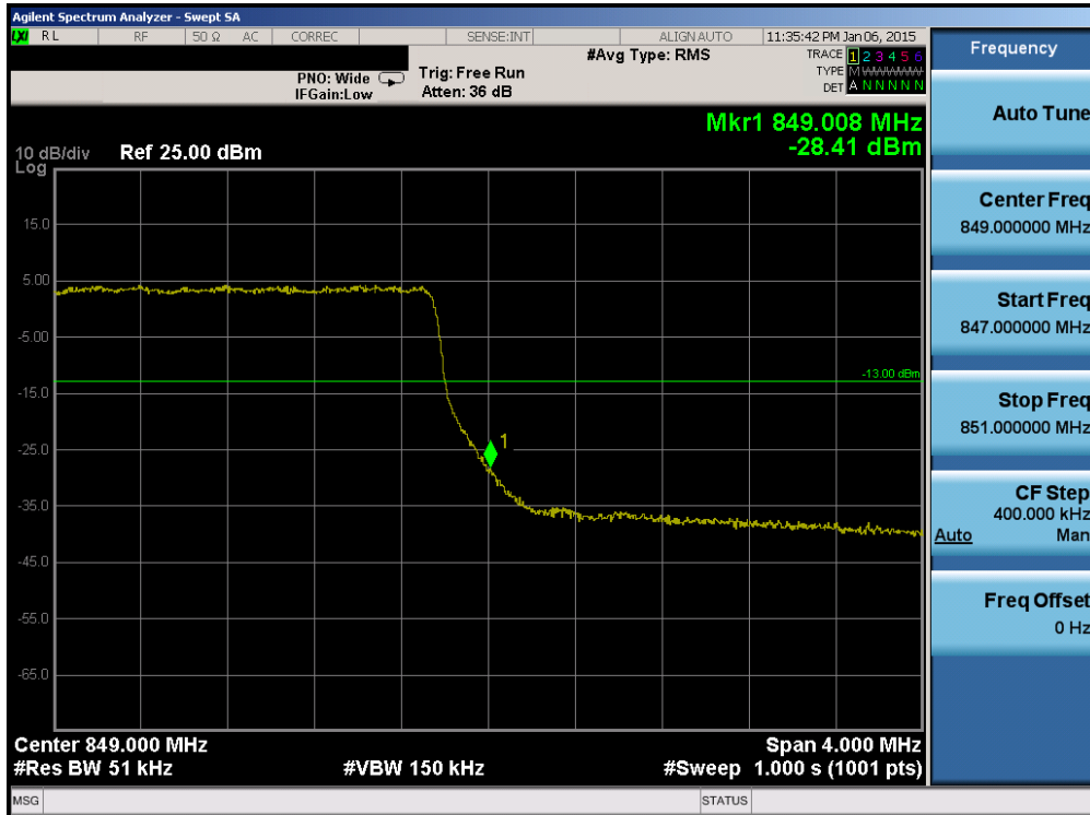
Plot 6-54. Upper Band Edge Plot (Band 5 – 5.0MHz QPSK – RB Size 25)
