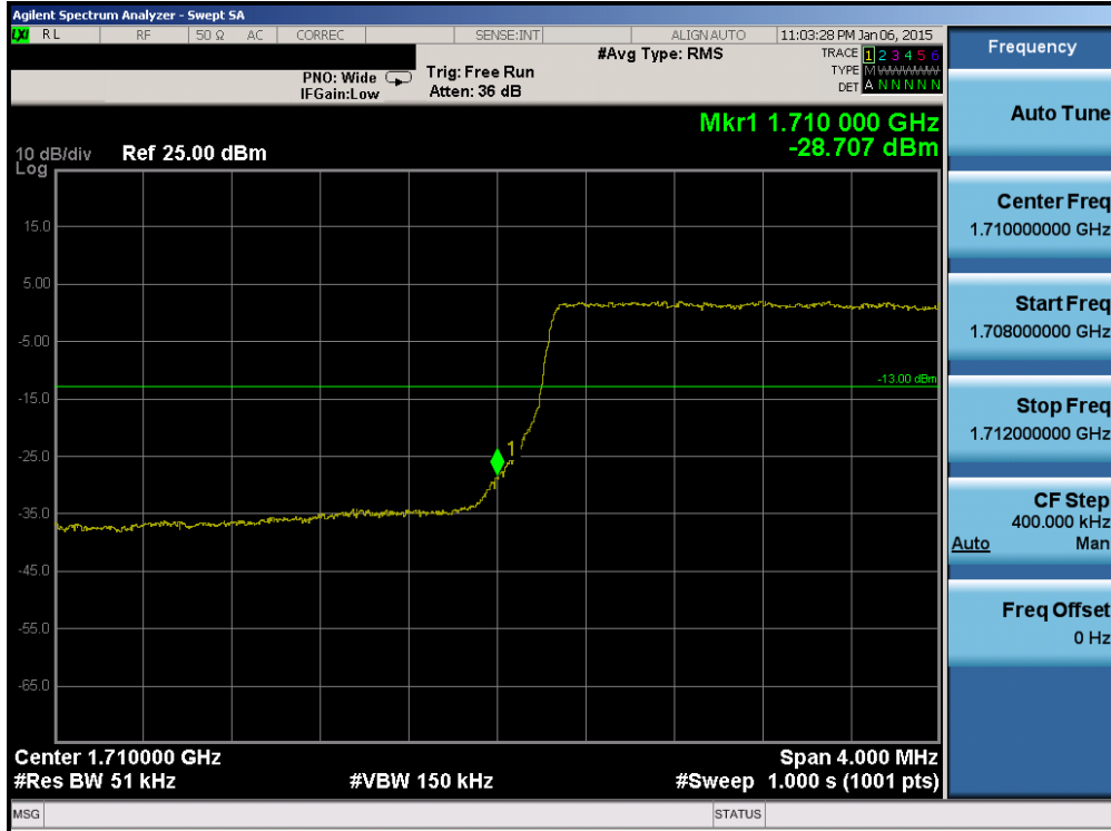
Plot 6-65. Lower Band Edge Plot (Band 4 – 5.0MHz QPSK – RB Size 25)
