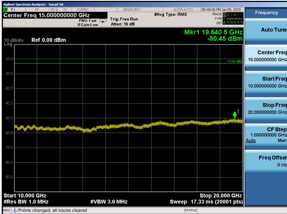
Plot 6-42. Conducted Spurious Plot (Band 2 – 10.0MHz QPSK – RB Size 1, RB Offset 0 – Mid Channel)
