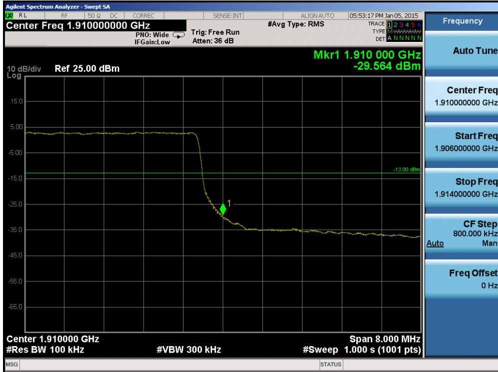
Plot 6-95. Upper Band Edge Plot (Band 2 – 10.0MHz QPSK – RB Size 50)
