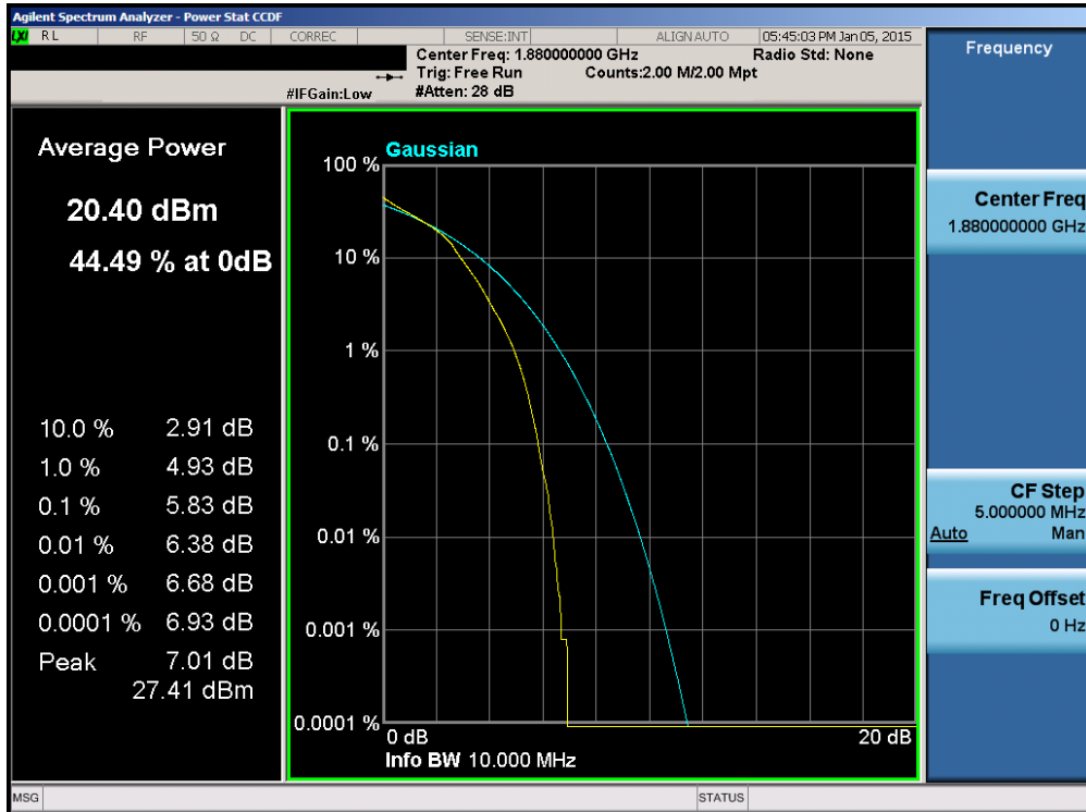
Plot 6-112. PAR Plot (Band 2 – 10.0MHz 16-QAM – RB Size 50)
