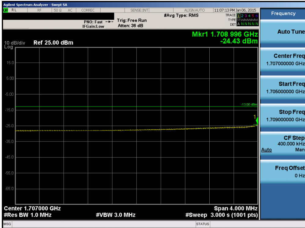
Plot 6-70. Lower Extended Band Edge Plot (Band 4 – 10.0MHz QPSK – RB Size 50)
