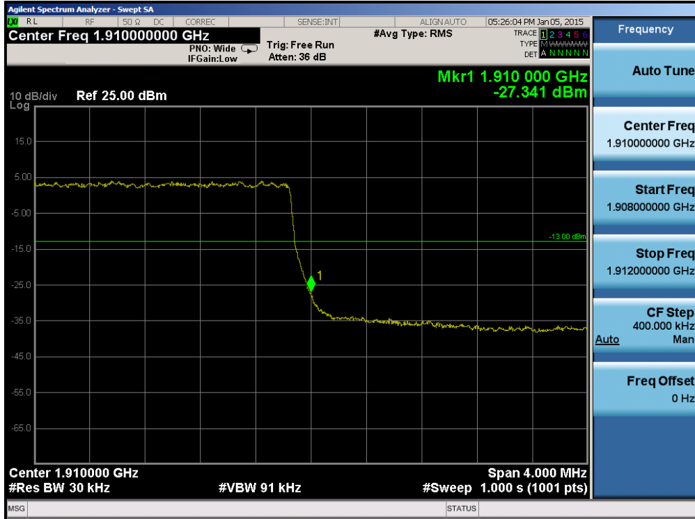
Plot 6-87. Upper Band Edge Plot (Band 2 – 3.0MHz QPSK – RB Size 15)
