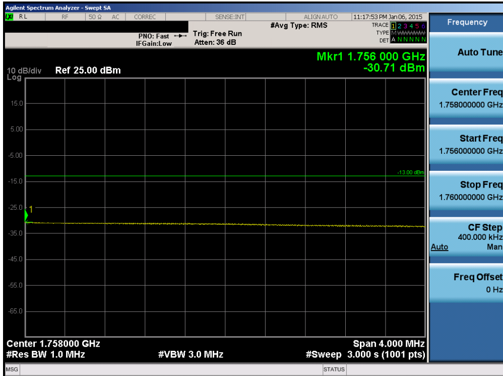
Plot 6-80. Upper Extended Band Edge Plot (Band 4 – 20.0MHz QPSK – RB Size 100)
