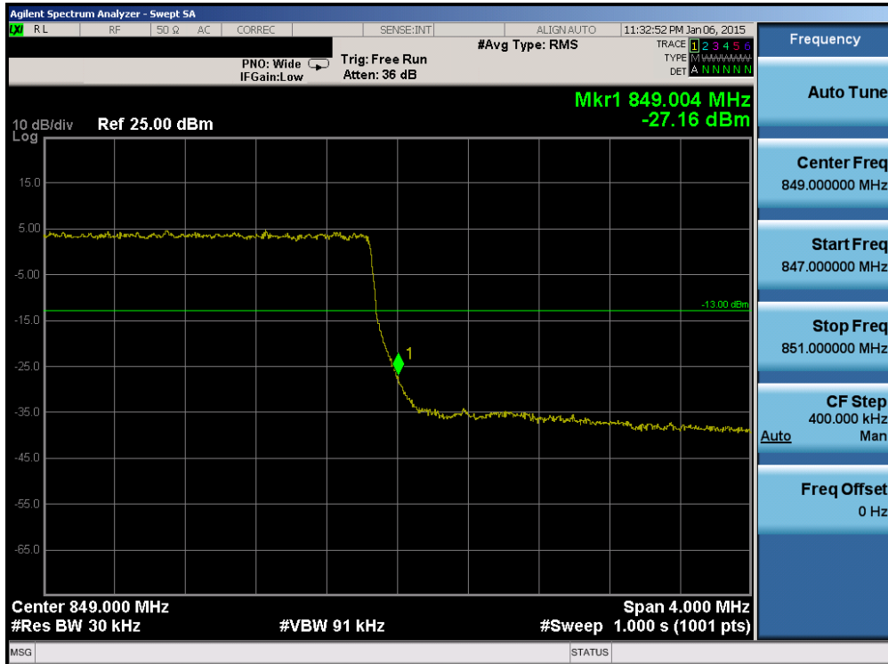
Plot 6-52. Upper Band Edge Plot (Band 5 – 3.0MHz QPSK – RB Size 15)
