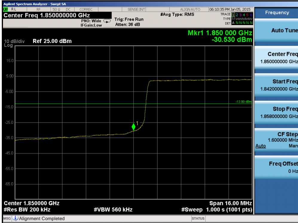
Plot 6-101. Lower Band Edge Plot (Band 2 – 20.0MHz QPSK – RB Size 100)
