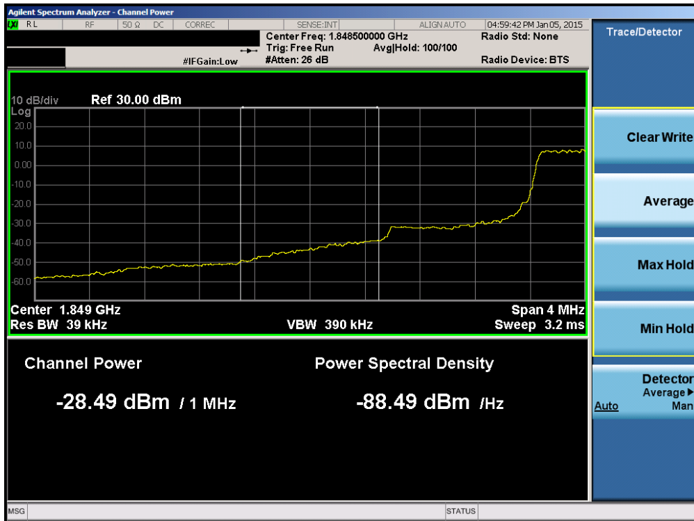
Plot 6-82. Lower Extended Band Edge Plot (Band 2 – 1.4MHz QPSK – RB Size 6)
