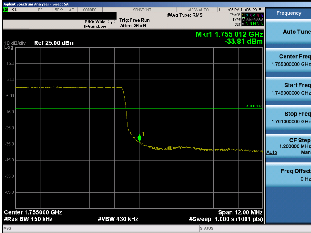
Plot 6-75. Upper Band Edge Plot (Band 4 – 15.0MHz QPSK – RB Size 75)
