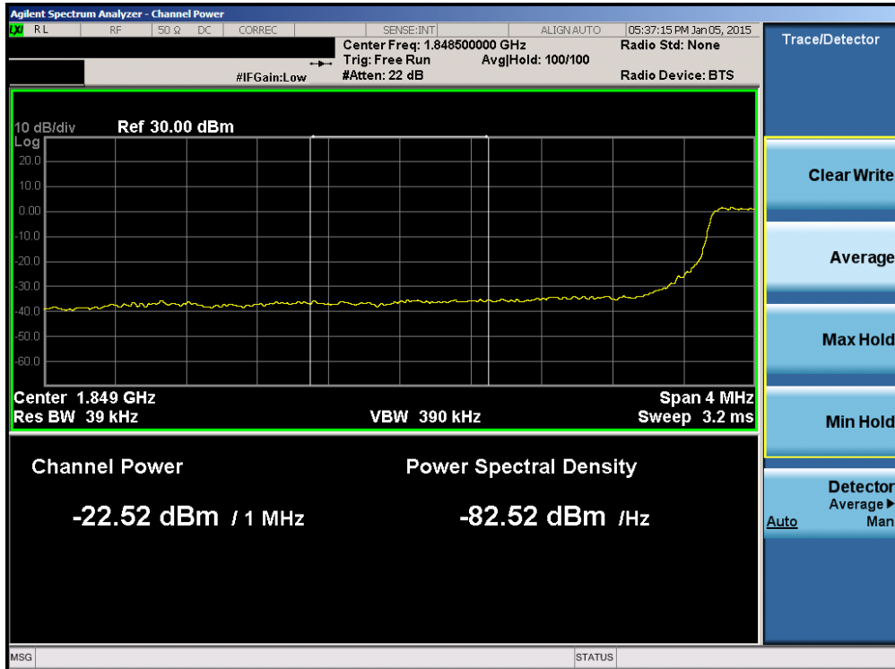
Plot 6-90. Lower Extended Band Edge Plot (Band 2 – 5.0MHz QPSK – RB Size 25)
