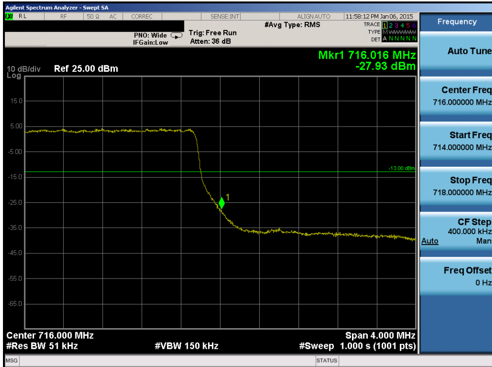
Plot 6-46. Upper Band Edge Plot (Band 17 – 5.0MHz QPSK – RB Size 25)
