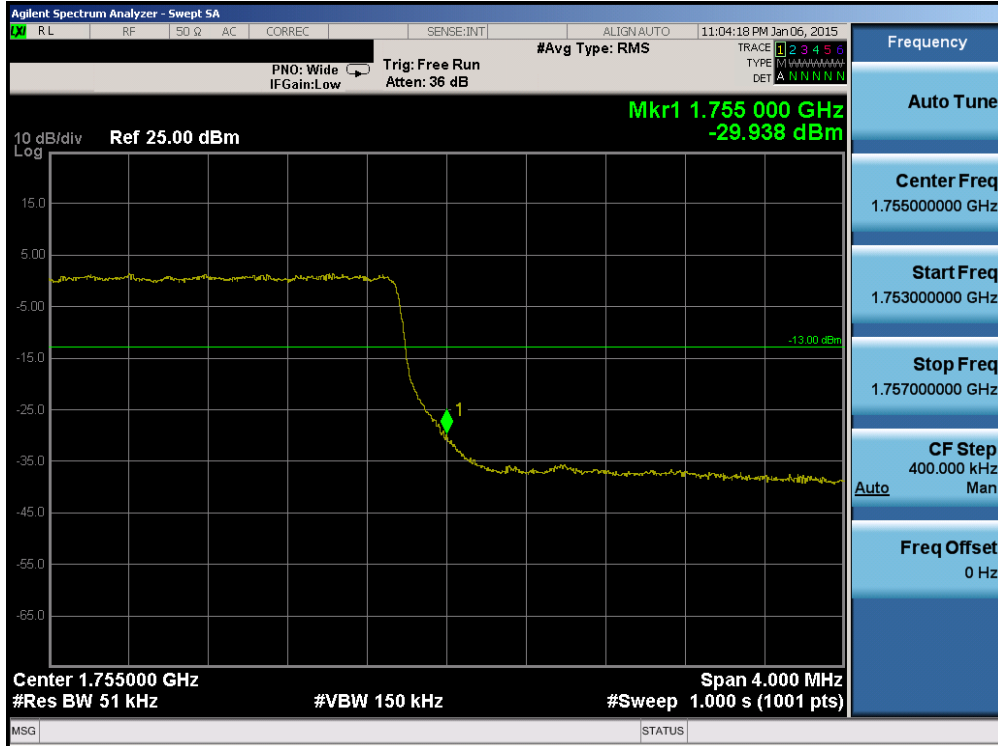
Plot 6-67. Upper Band Edge Plot (Band 4 – 5.0MHz QPSK – RB Size 25)
