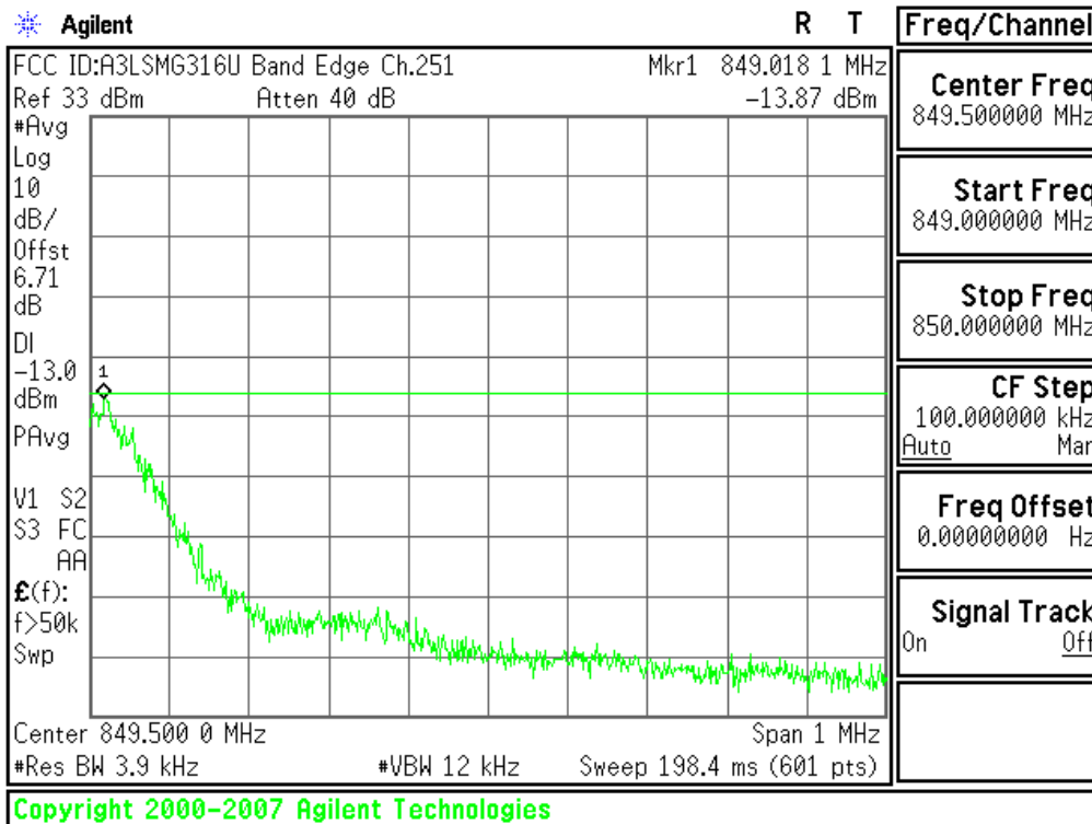
Plot 6-46. Upper Band Edge Plot (Cellular GSM Mode – Ch.251)
