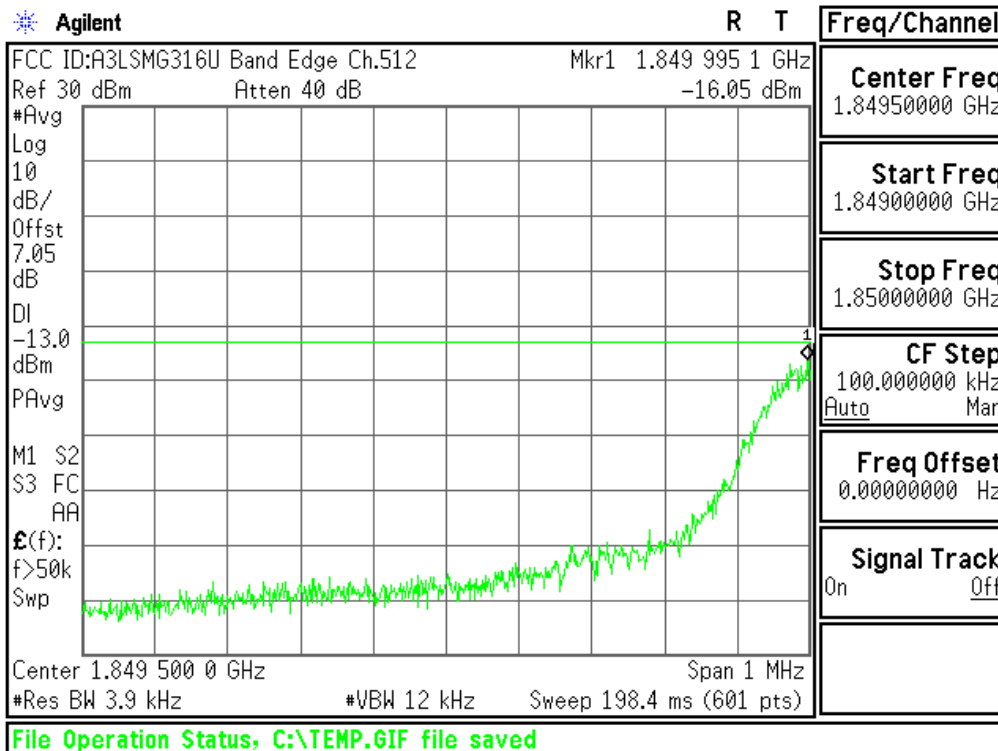
Plot 6-48. Lower Band Edge Plot (PCS GSM Mode – Ch.512)
