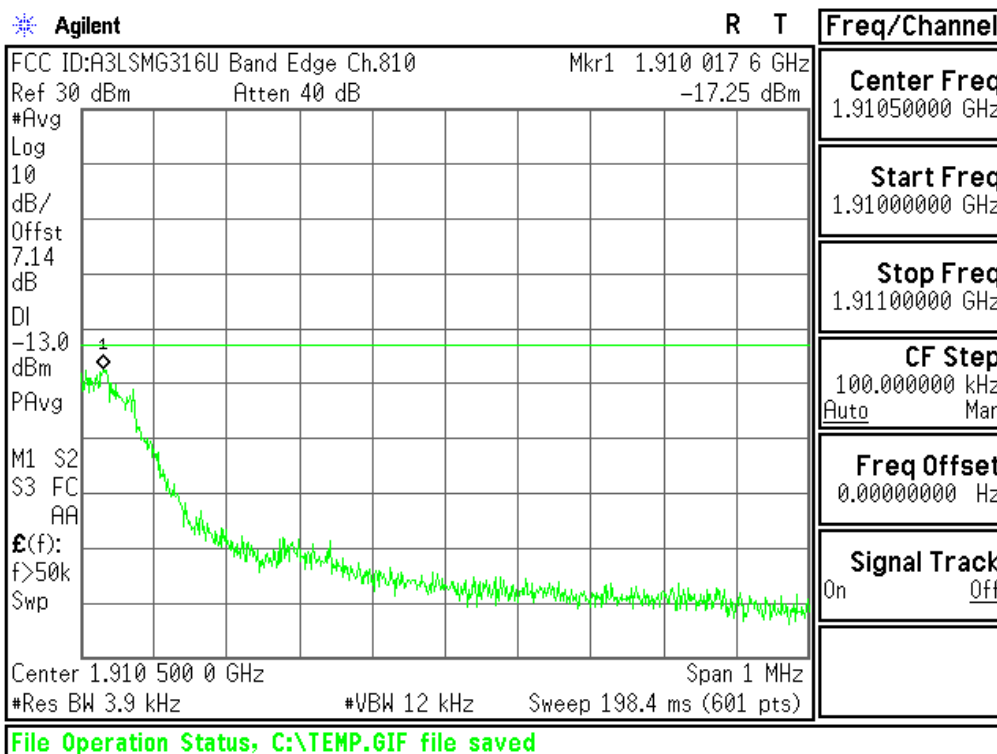
Plot 6-50. Upper Band Edge Plot (PCS GSM Mode – Ch.810)
