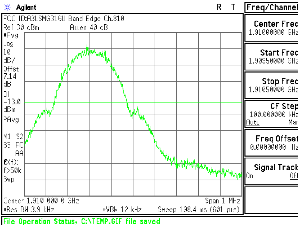
Plot 6-49. Upper Band Edge Plot (PCS GSM Mode – Ch.810)
