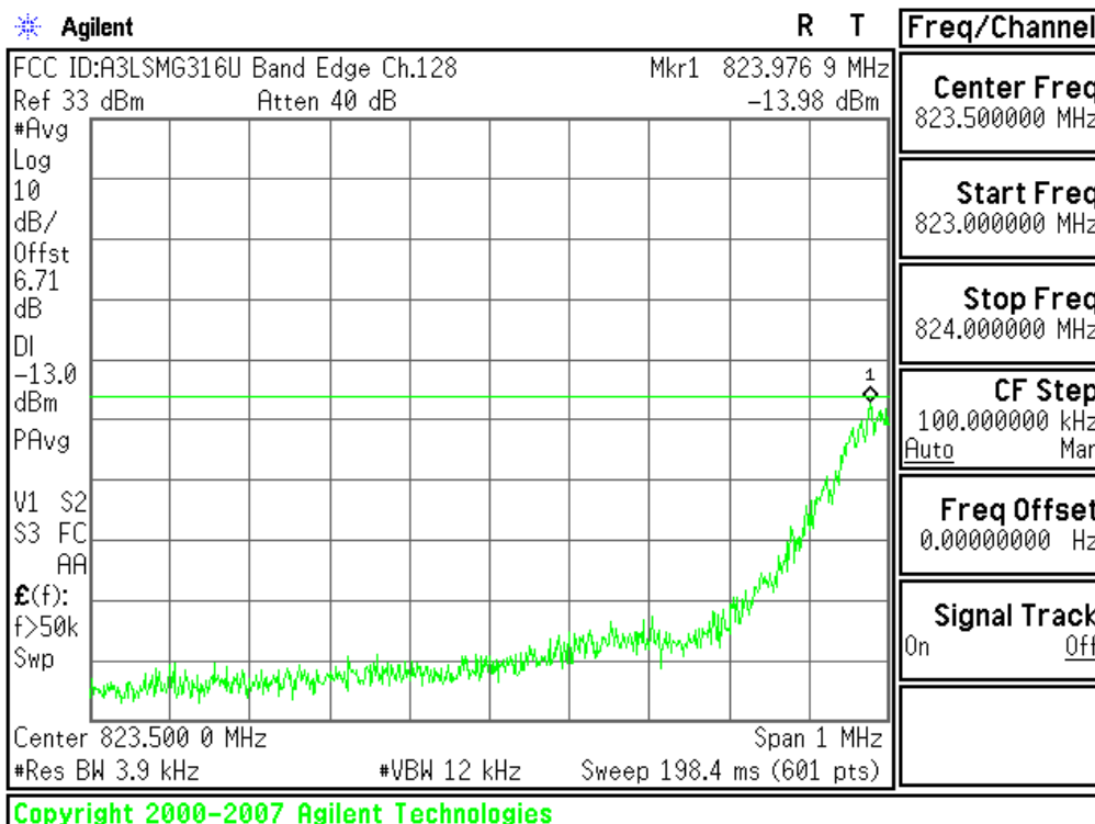
Plot 6-44. Lower Band Edge Plot (Cellular GSM Mode – Ch.128)
