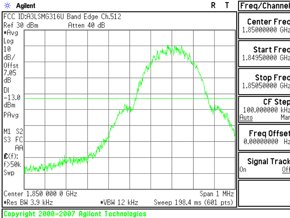
Plot 6-47. Lower Band Edge Plot (PCS GSM Mode – Ch.512)
