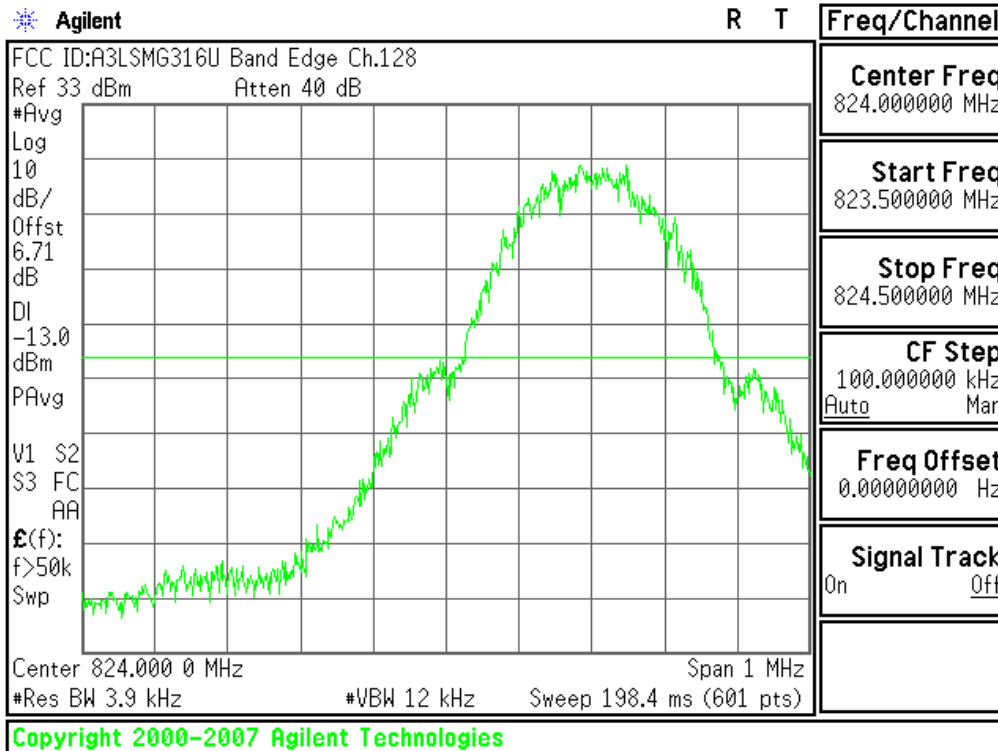
Plot 6-43. Lower Band Edge Plot (Cellular GSM Mode – Ch.128)
