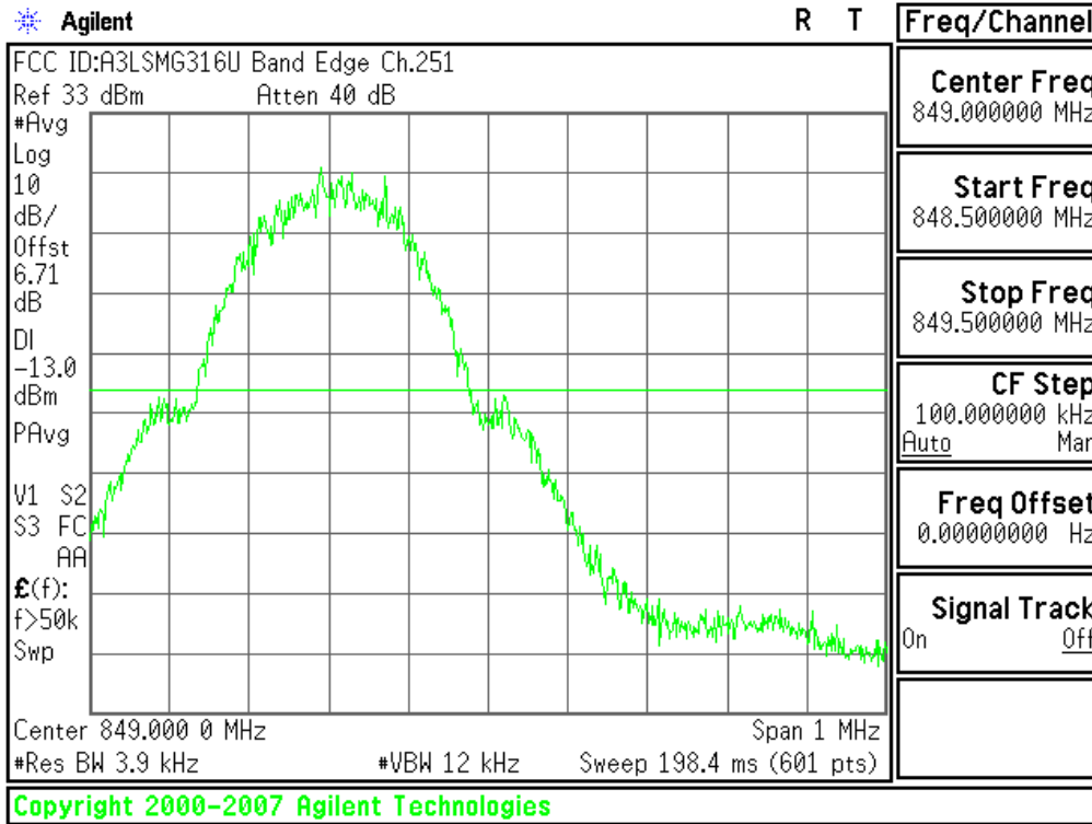
Plot 6-45. Upper Band Edge Plot (Cellular GSM Mode – Ch.251)
