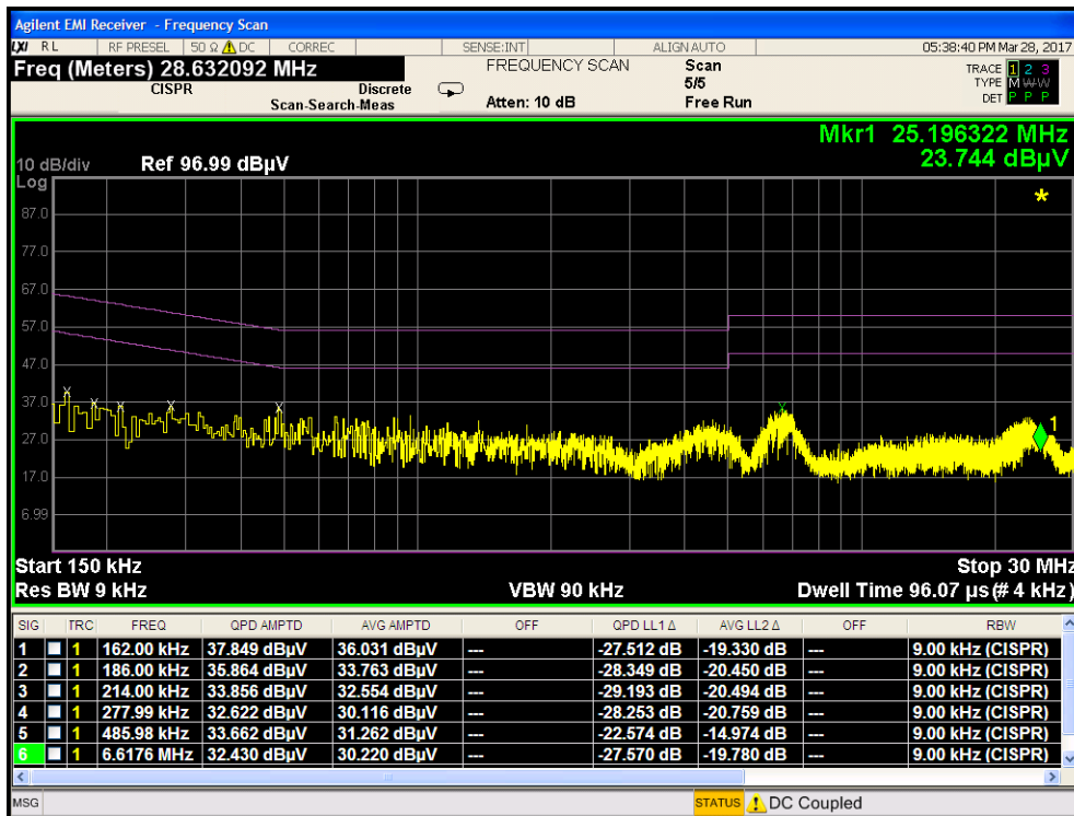
Plot 7-98. Line Conducted Plot with 802.11a UNII Band 3 (N)
