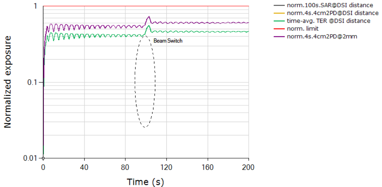
Total Normalized Time-averaged RF Exposure Tech: LTE, Band 66 / Tech: NR5G MMW, Band 261
