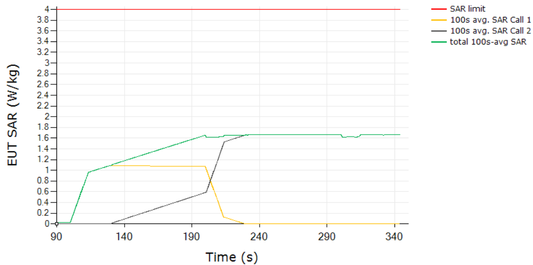
SAR Call Drop Tech: LTE, Band 41
