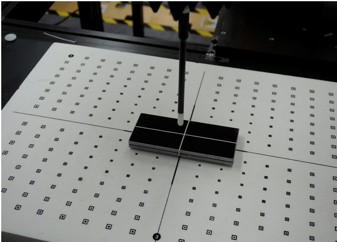
Front View of the DUT
