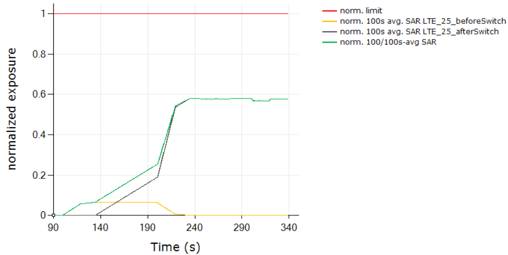
Total Normalized Time-averaged RF Exposure Tech: LTE, Band 25
