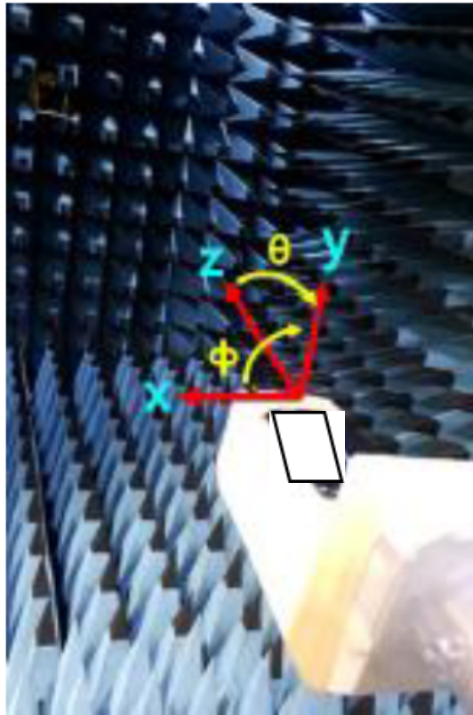
Figure 1: Geometry for Q5 for Radiation patterns
