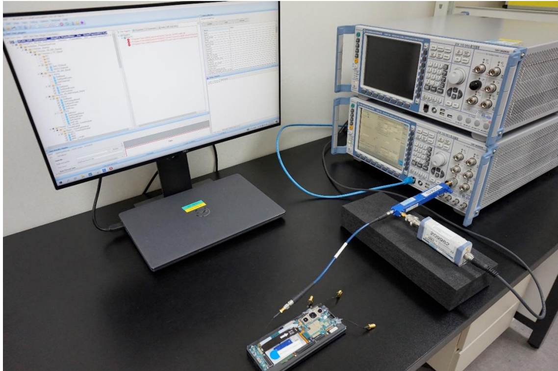
A.1 : Conducted test in CMW500 callbox
