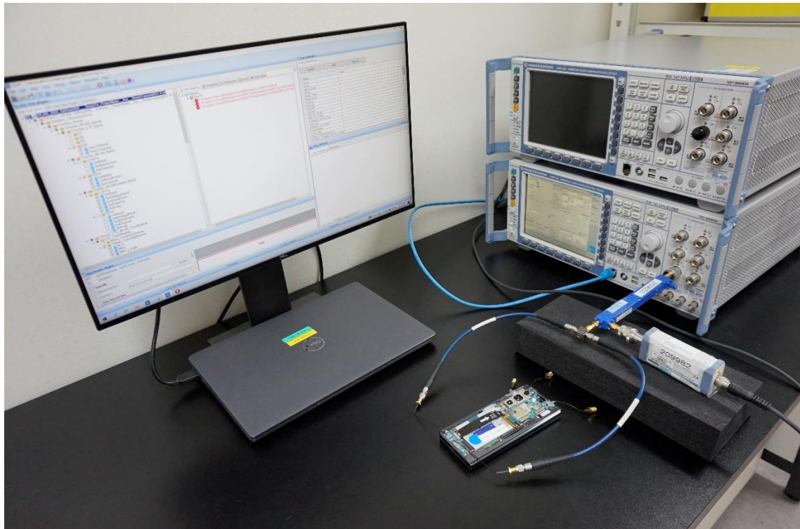
A.2 : Conducted test in CMW500 callbox
