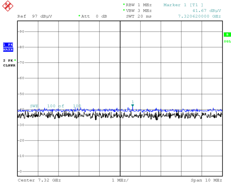
Radiated Spurious Emissions plot – Peak Result (Ch. 19 3rd Harmonic, X-H)
