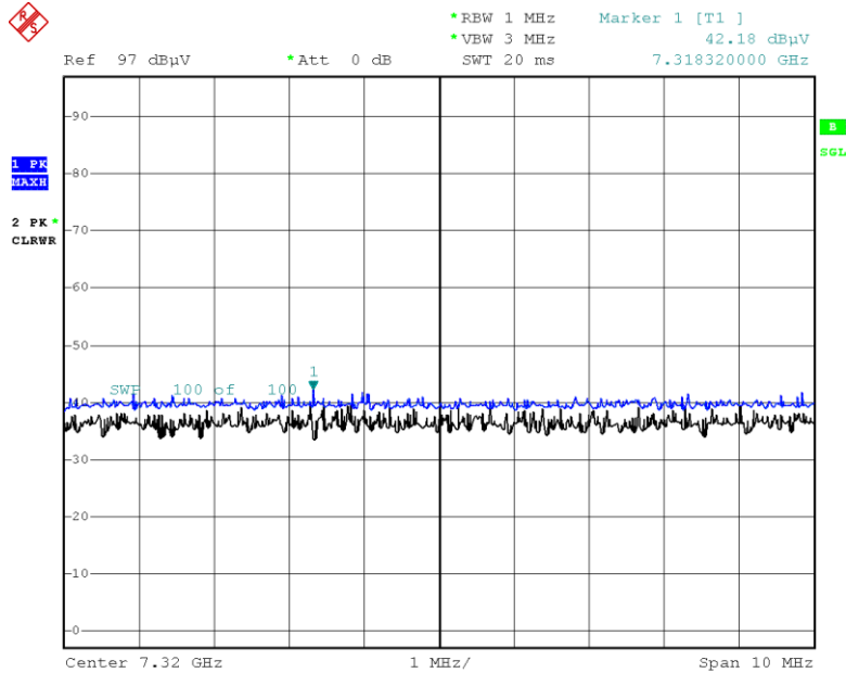
Radiated Spurious Emissions plot – Peak Result (Ch. 19 3rd Harmonic, Y-H)
