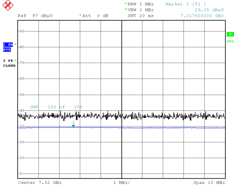
Radiated Spurious Emissions plot – Average Result (Ch. 19 3rd Harmonic, X-V)
