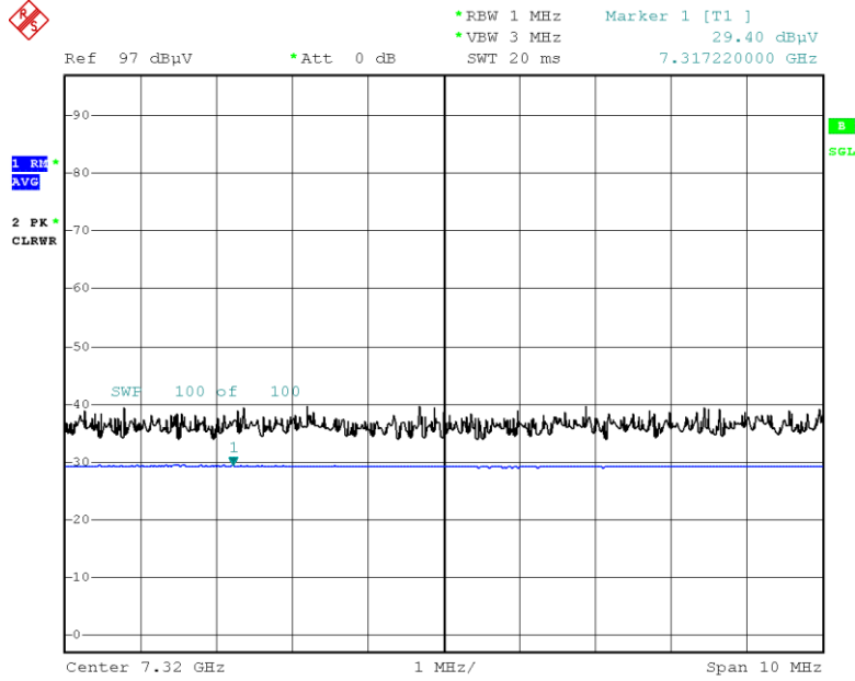
Radiated Spurious Emissions plot – Average Result (Ch. 19 3rd Harmonic, Z-H)
