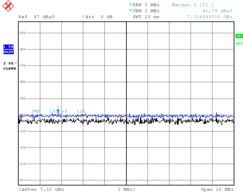
Radiated Spurious Emissions plot – Peak Result (Ch. 19 3rd Harmonic, X-V)
