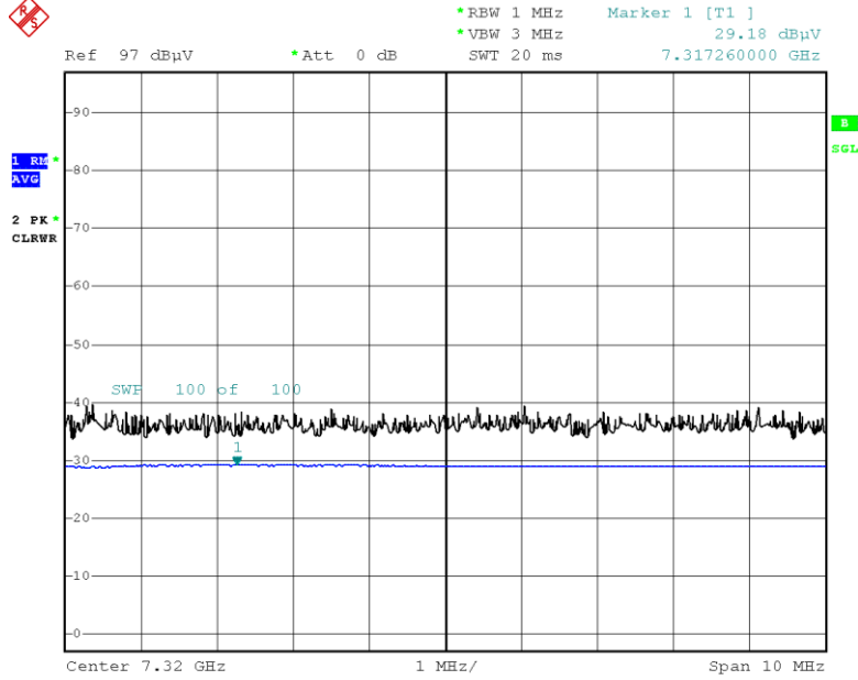
Radiated Spurious Emissions plot – Average Result (Ch. 19 3rd Harmonic, X-H)
