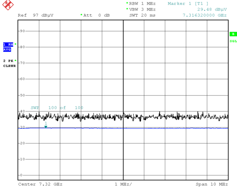
Radiated Spurious Emissions plot – Average Result (Ch. 19 3rd Harmonic, Y-H)
