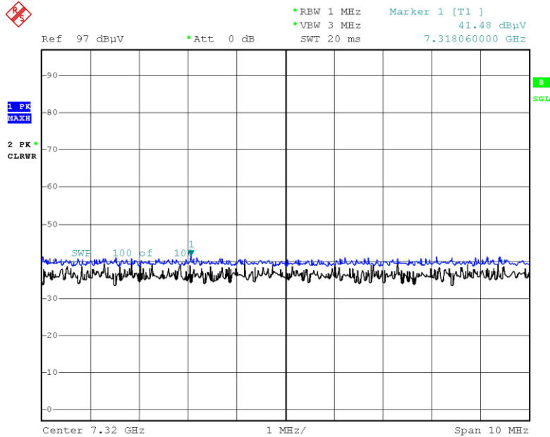
Radiated Spurious Emissions plot – Peak Result (Ch. 19 3rd Harmonic, Z-H)
