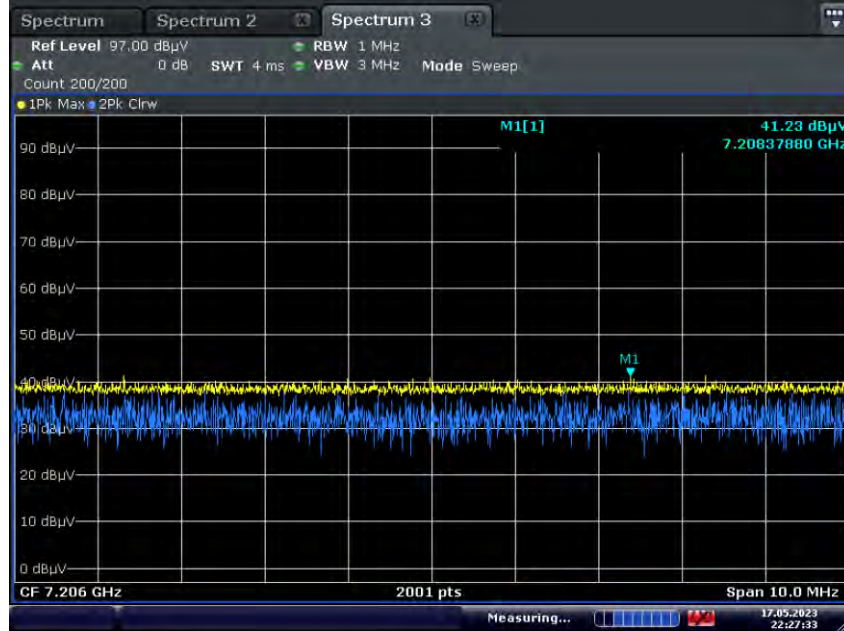
Radiated Spurious Emissions plot – Peak & Average Result (3rd Harmonic, X-H)
