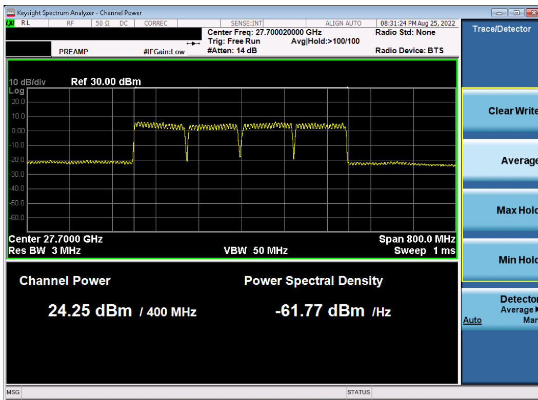
Plot 7-76. Ant2 EIRP Plot (Band n261 – 100MHz-4CC – \pi/2 -BPSK – Low Channel)
