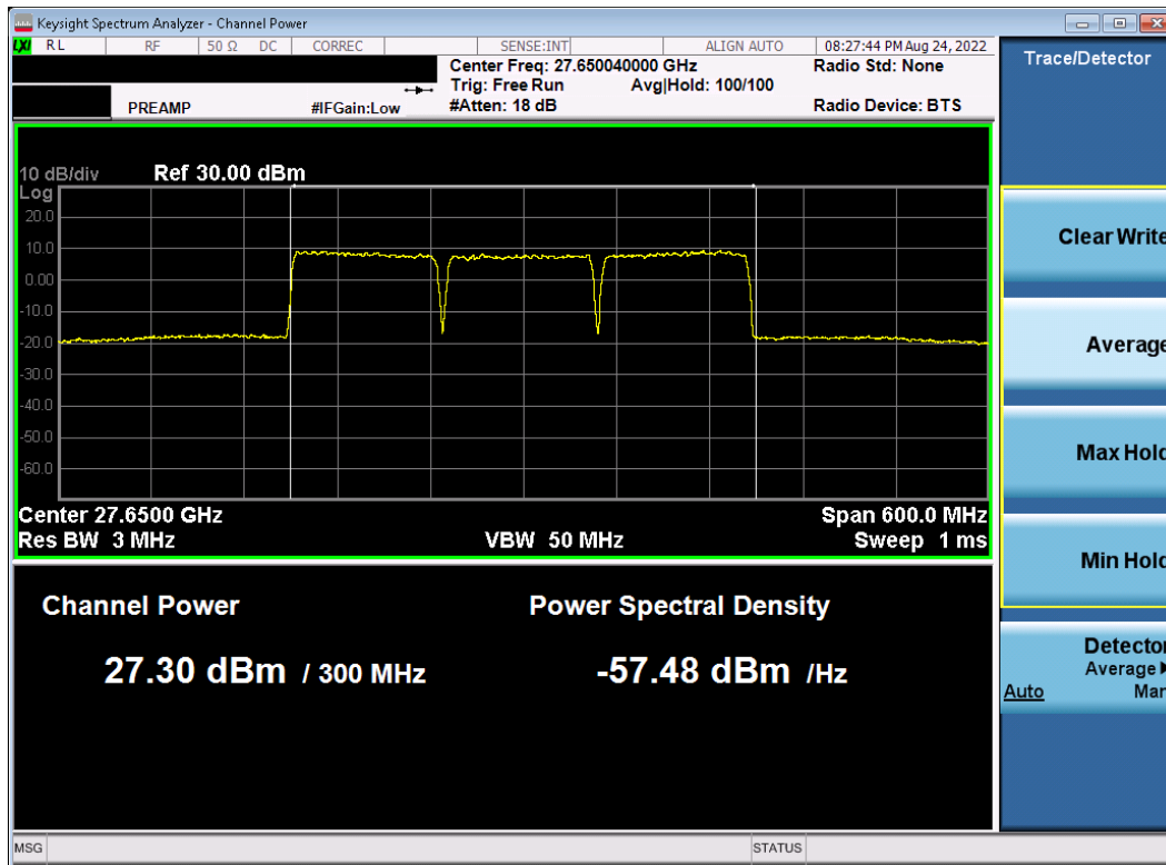
Plot 7-71. Ant1 EIRP Plot (Band n261 – 100MHz-3CC – \pi/2 BPSK – Low Channel)
