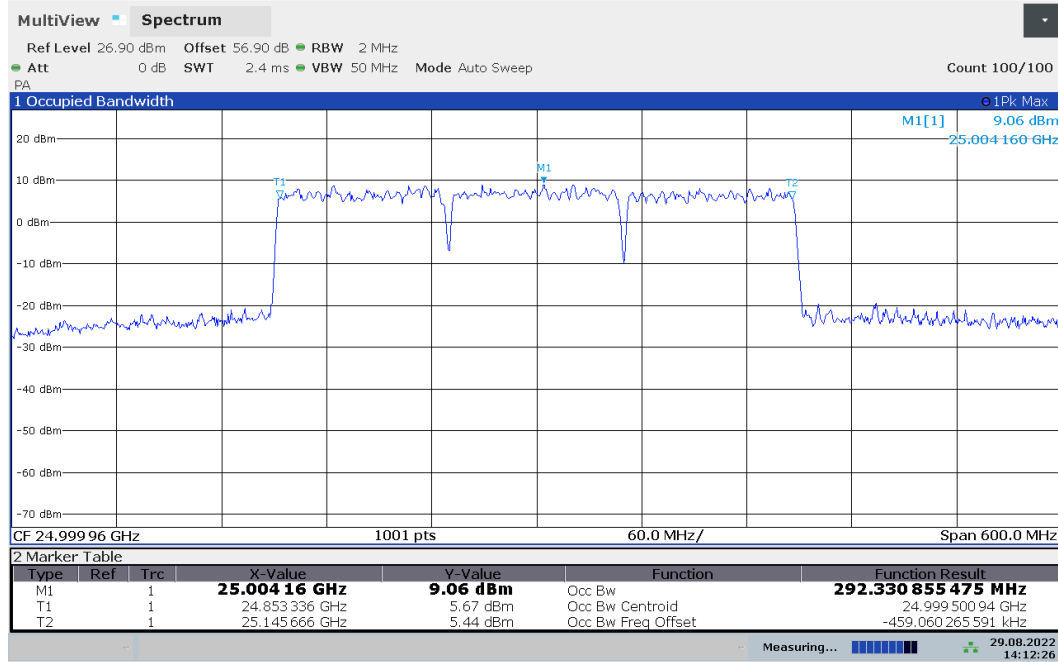
Plot 7-19. Occupied Bandwidth Plot (100MHz-3CC – 16QAM – Mid Channel)
