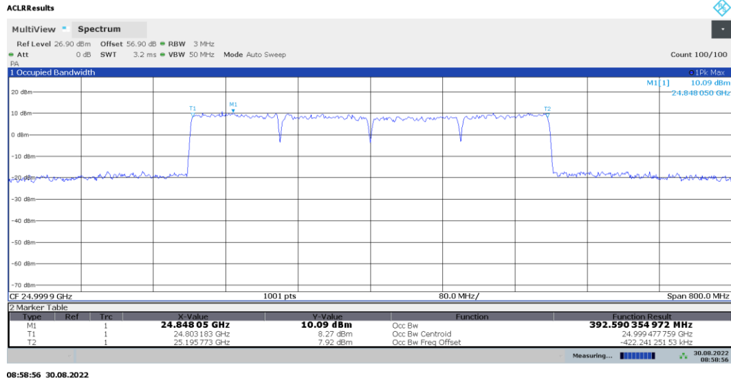
Plot 7-21. Occupied Bandwidth Plot (100MHz-4CC – QPSK – Mid Channel)
