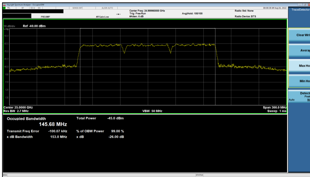
Plot 7-10. Occupied Bandwidth Plot (50MHz-3CC – \pi/2 -BPSK – Mid Channel)
