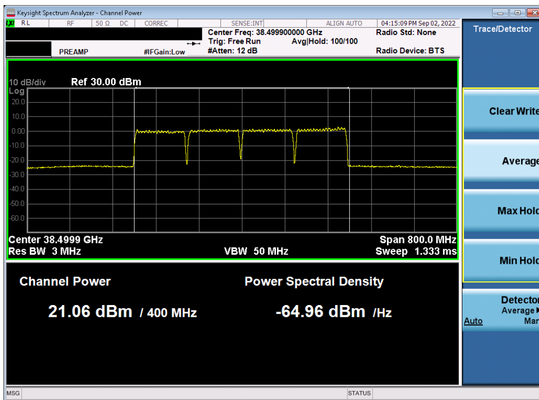
Plot 7-84. Ant2 EIRP Plot (Band n260 – 100MHz-4CC – \pi/2 -BPSK – Mid Channel)
