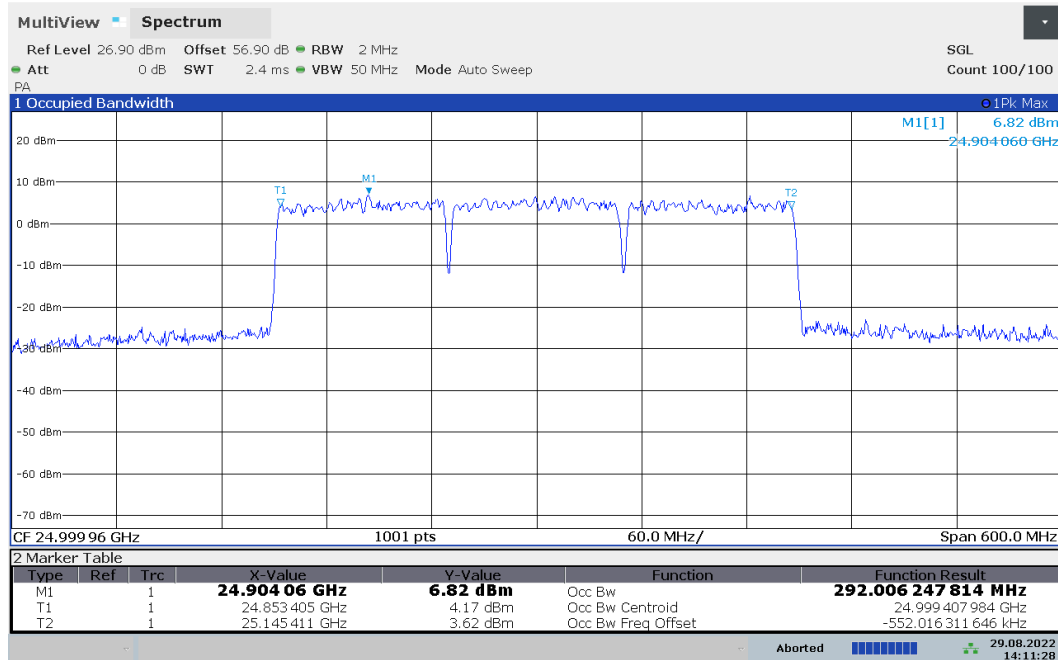
Plot 7-20. Occupied Bandwidth Plot (100MHz-3CC – 64QAM – Mid Channel)
