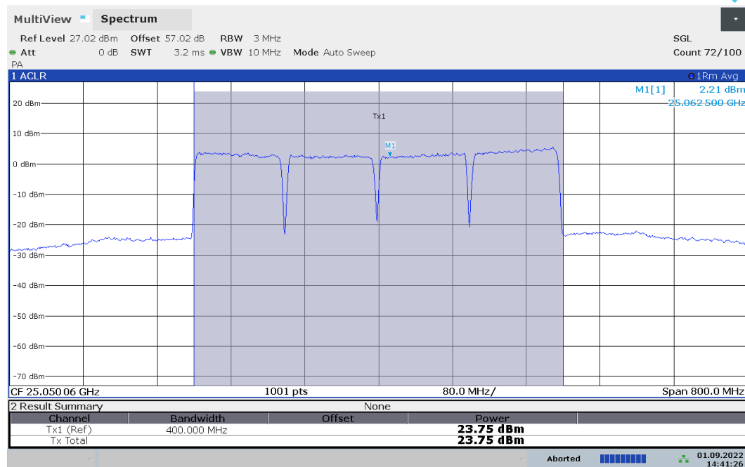
Plot 7-68. Ant2 EIRP Plot (Band n258-R2 – 100MHz-4CC – \pi/2 -BPSK – High Channel)
