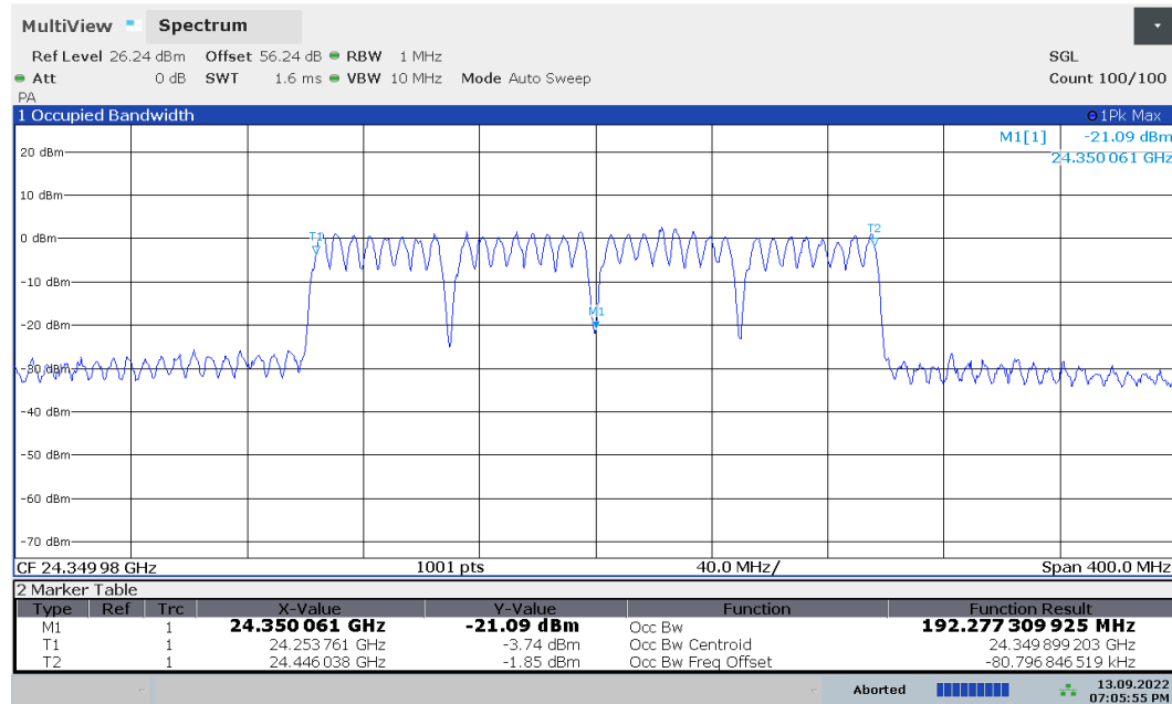
Plot 7-5. Occupied Bandwidth Plot (50MHz-4CC – QPSK – Mid Channel)
