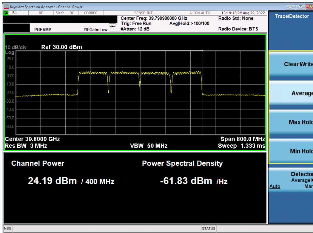
Plot 7-80. Ant1 EIRP Plot (Band n260 - 100MHz-4CC - \pi/2 -BPSK - High Channel)
