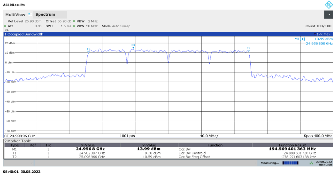
Plot 7-14. Occupied Bandwidth Plot (50MHz-4CC – \pi/2 -BPSK – Mid Channel)
