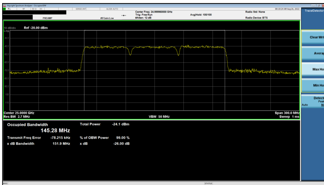
Plot 7-12. Occupied Bandwidth Plot (50MHz-3CC – 64QAM – Mid Channel)
