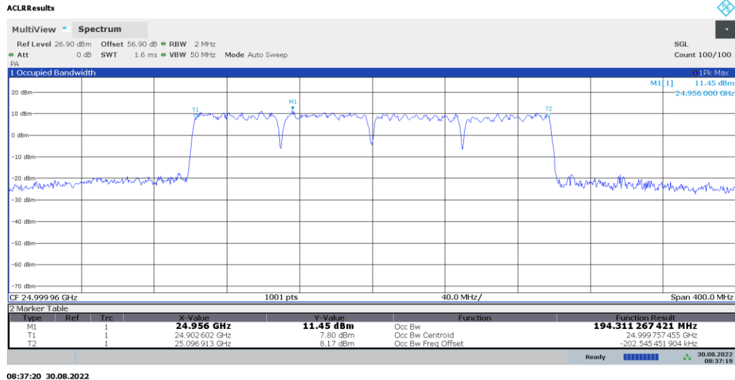
Plot 7-15. Occupied Bandwidth Plot (50MHz-4CC – 16QAM – Mid Channel)
