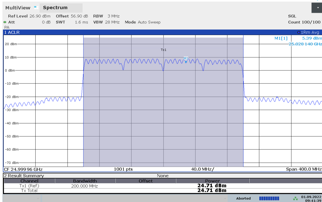
Plot 7-66. Ant2 EIRP Plot (Band n258-R2 - 50MHz-4CC - \pi/2 -BPSK - Mid Channel)
