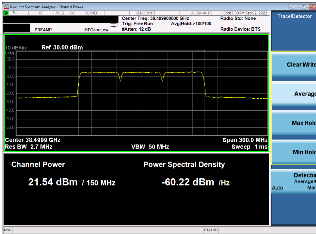
Plot 7-81. Ant2 EIRP Plot (Band n260 – 50MHz-3CC – QPSK – Mid Channel)
