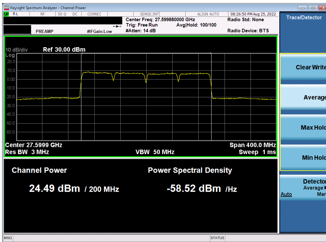
Plot 7-74. Ant2 EIRP Plot (Band n261 – 50MHz-4CC – \pi/2 -BPSK – Low Channel)
