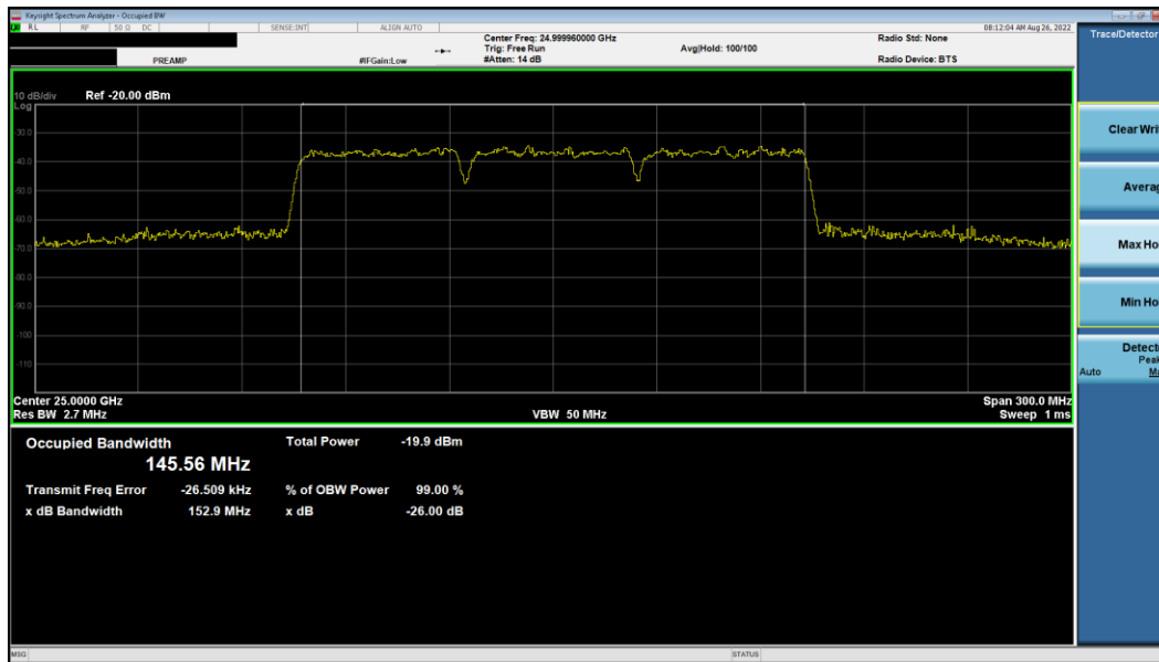
Plot 7-9. Occupied Bandwidth Plot (50MHz-3CC – QPSK – Mid Channel)
