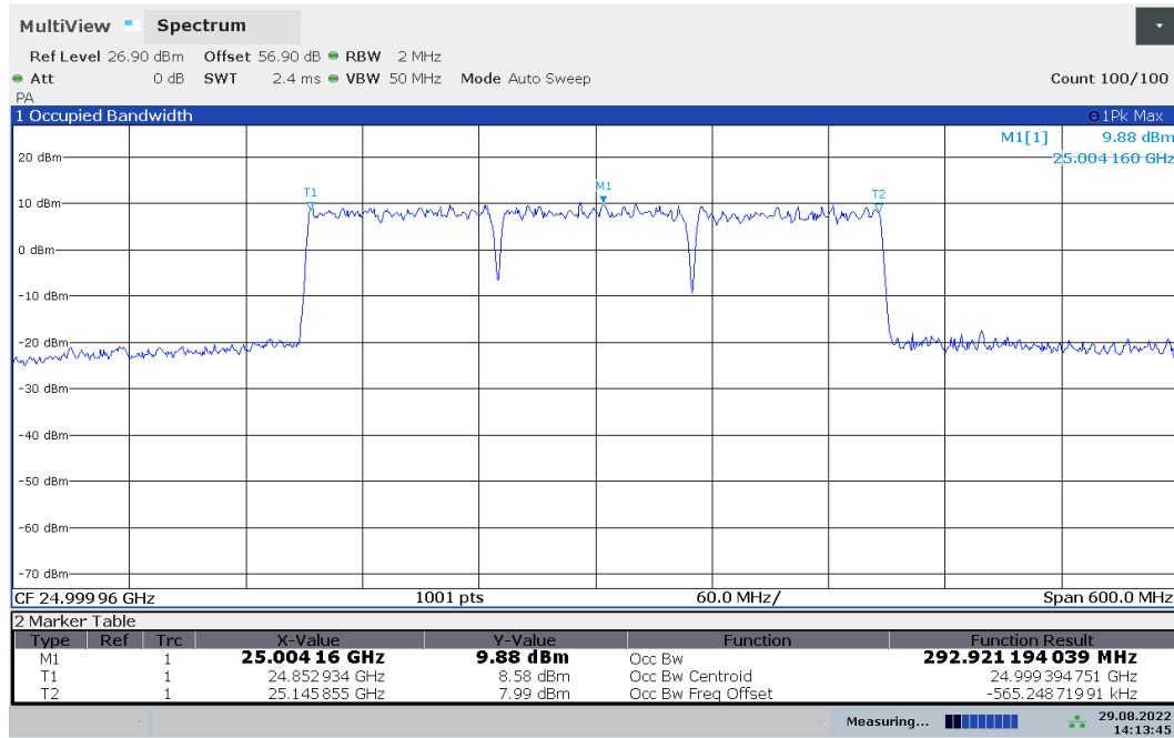
Plot 7-17. Occupied Bandwidth Plot (100MHz-3CC – QPSK – Mid Channel)
