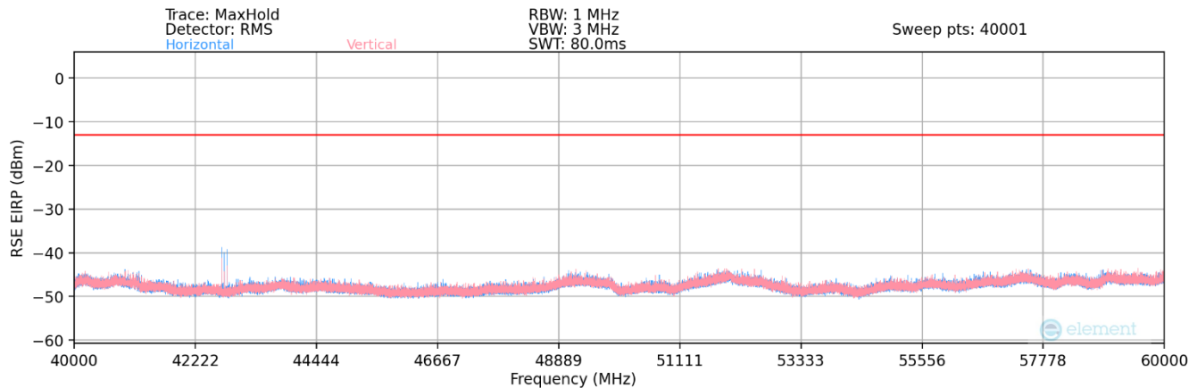
Plot 7-91. Ant 1-n260 Radiated Spurious Plot (3CC QPSK Mid Channel 2Tx)
