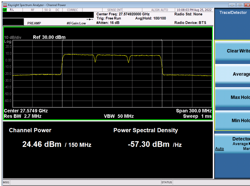
Plot 7-73. Ant2 EIRP Plot (Band n261 – 50MHz-3CC – QPSK – Low Channel)
