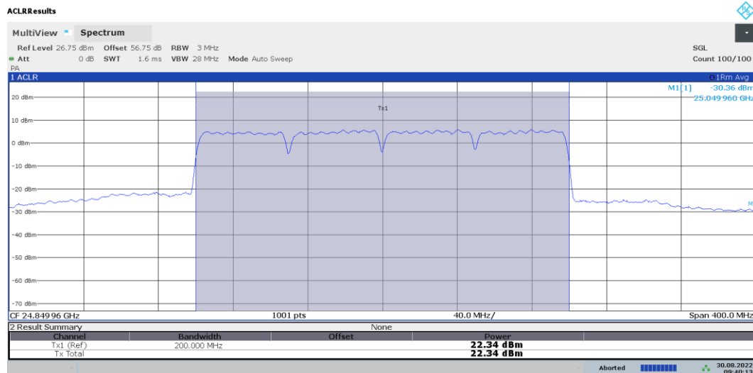
Plot 7-62. Ant1 EIRP Plot (Band n258-R2 – 50MHz-4CC – QPSK – Low Channel)
