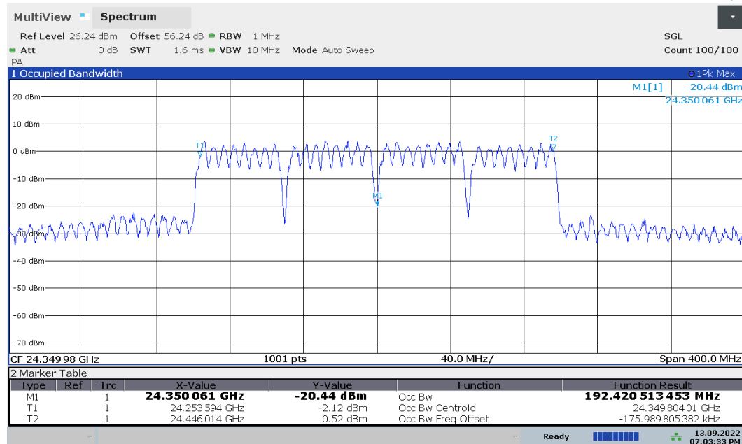
Plot 7-6. Occupied Bandwidth Plot (50MHz-4CC – \pi/2 -BPSK – Mid Channel)
