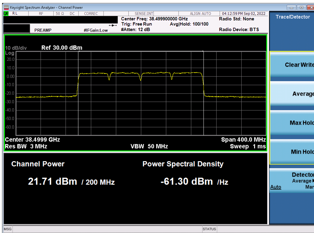
Plot 7-82. Ant2 EIRP Plot (Band n260 – 50MHz-4CC – \pi/2 -BPSK – Mid Channel)
