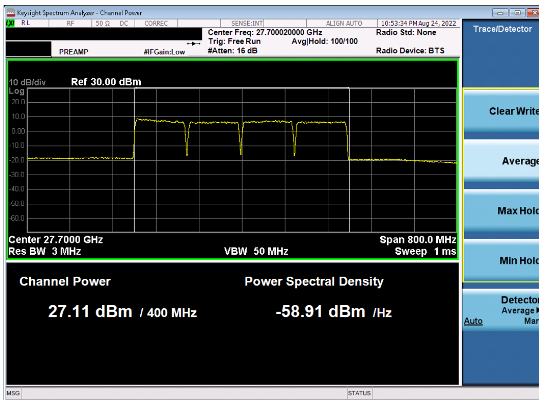
Plot 7-72. Ant1 EIRP Plot (Band n261 – 100MHz-4CC – QPSK – Low Channel)
