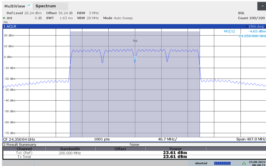
Plot 7-58. Ant1 EIRP Plot (Band n258-R1 – 50MHz-4CC – QPSK – Mid Channel)
