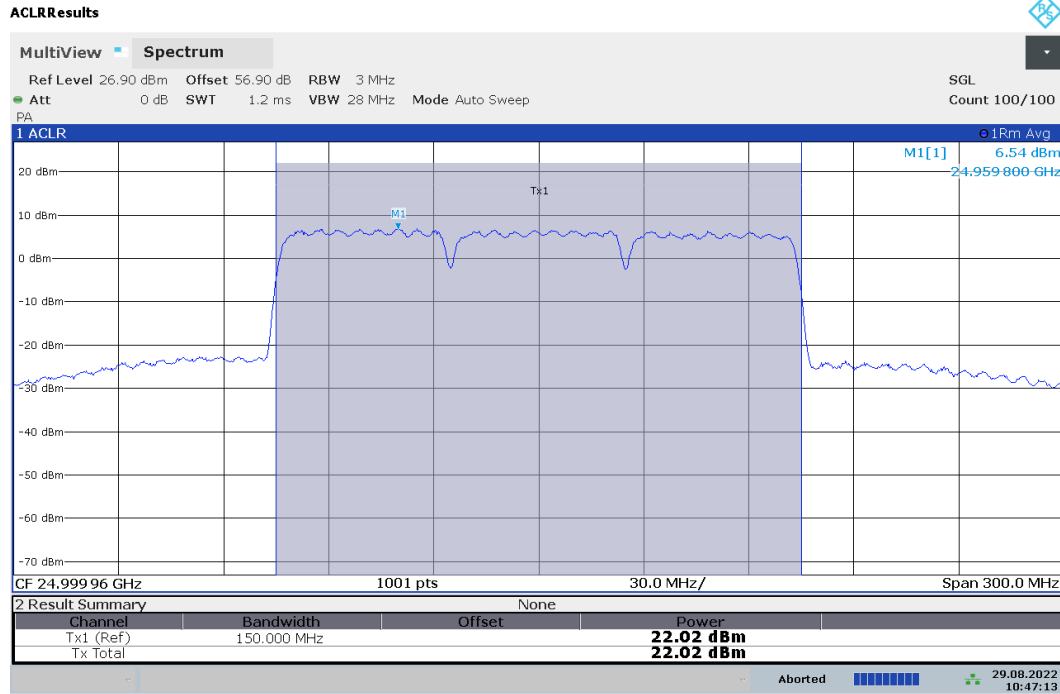
Plot 7-61. Ant1 EIRP Plot (Band n258-R2 – 50MHz-3CC – \pi/2 -BPSK – Mid Channel)
