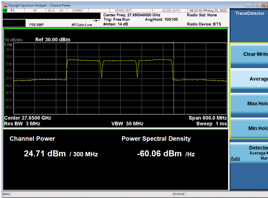
Plot 7-75. Ant2 EIRP Plot (Band n261 – 100MHz-3CC – \pi/2 -BPSK – Low Channel)
