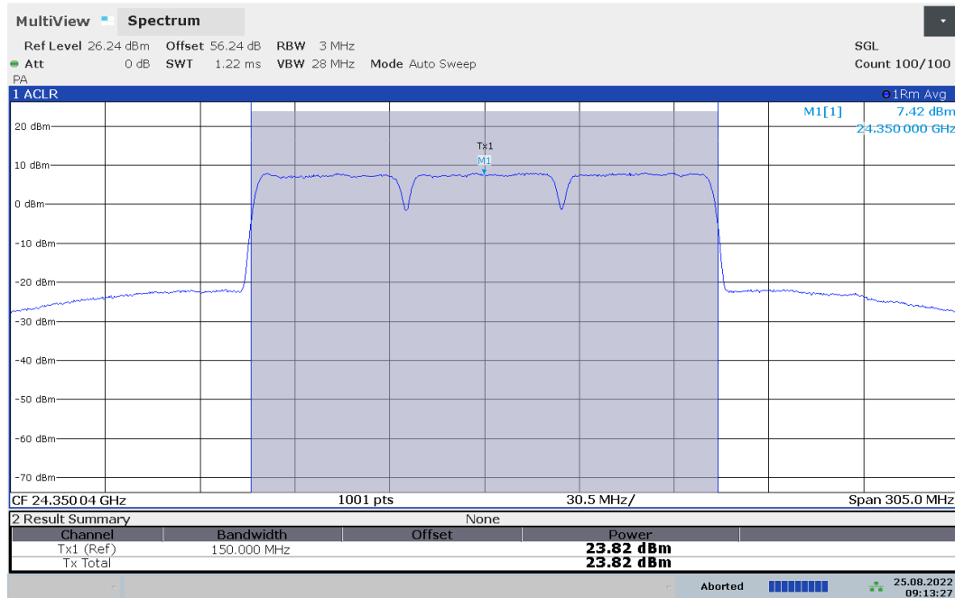
Plot 7-57. Ant1 EIRP Plot (Band n258-R1 – 50MHz-3CC – QPSK – Mid Channel)
