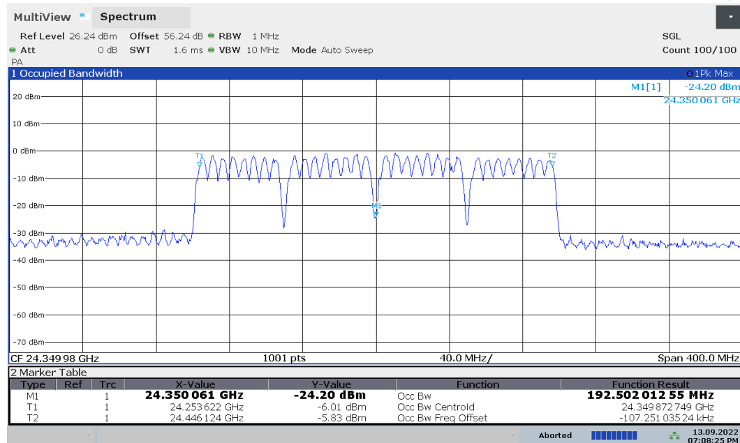
Plot 7-8. Occupied Bandwidth Plot (50MHz-4CC – 64QAM – Mid Channel)
