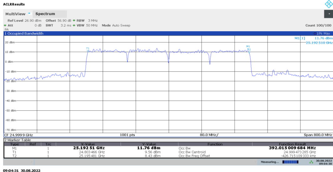
Plot 7-22. Occupied Bandwidth Plot (100MHz-4CC – \pi/2 -BPSK – Mid Channel)
