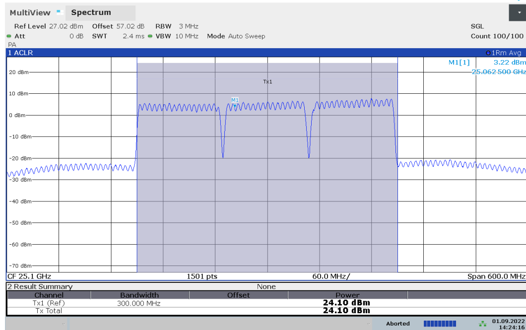
Plot 7-67. Ant2 EIRP Plot (Band n258-R2 – 100MHz-3CC – QPSK – High Channel)
