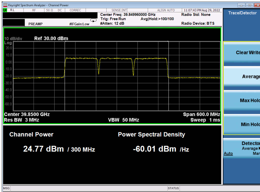
Plot 7-79. Ant1 EIRP Plot (Band n260 - 100MHz-3CC - \pi/2 -BPSK - High Channel)
