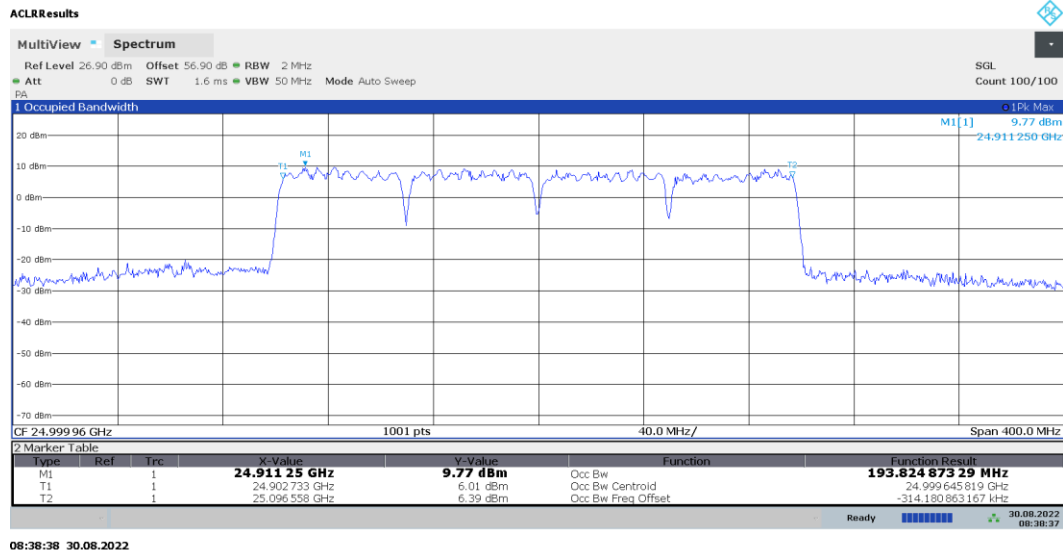
Plot 7-16. Occupied Bandwidth Plot (50MHz-4CC – 64QAM – Mid Channel)
