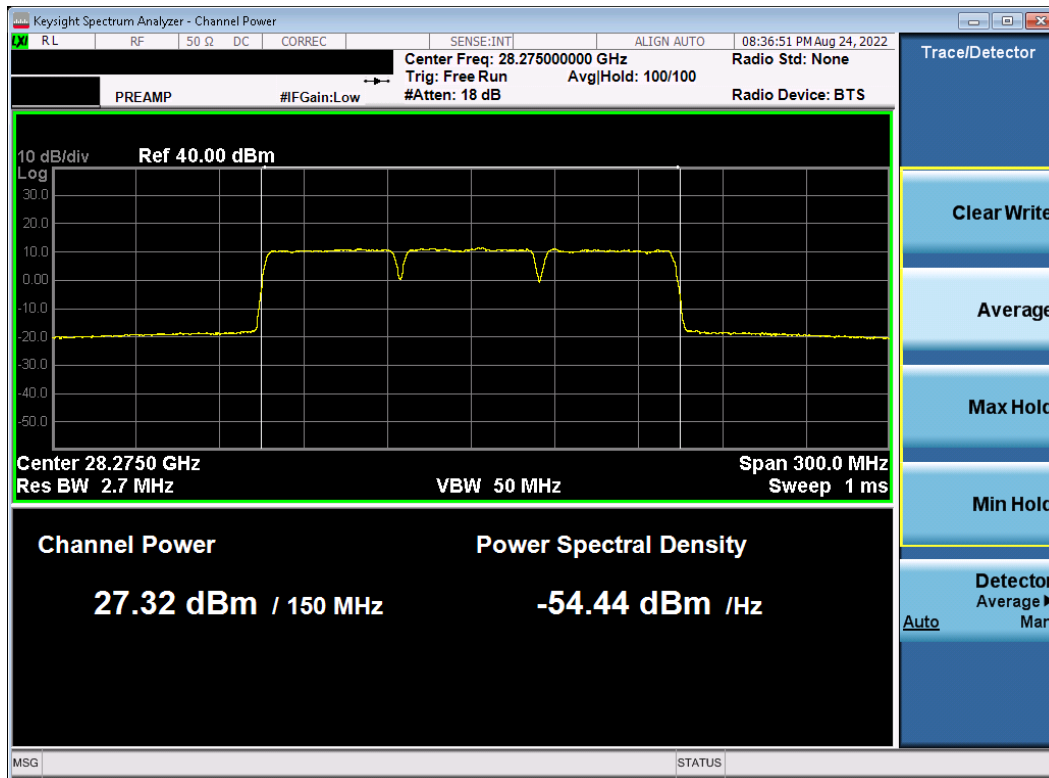
Plot 7-69. Ant1 EIRP Plot (Band n261 – 50MHz-3CC – QPSK – High Channel)
