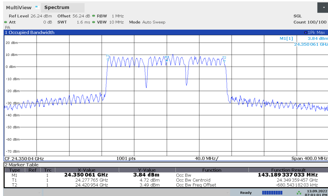
Plot 7-4. Occupied Bandwidth Plot (50MHz-3CC – 64QAM – Mid Channel)
