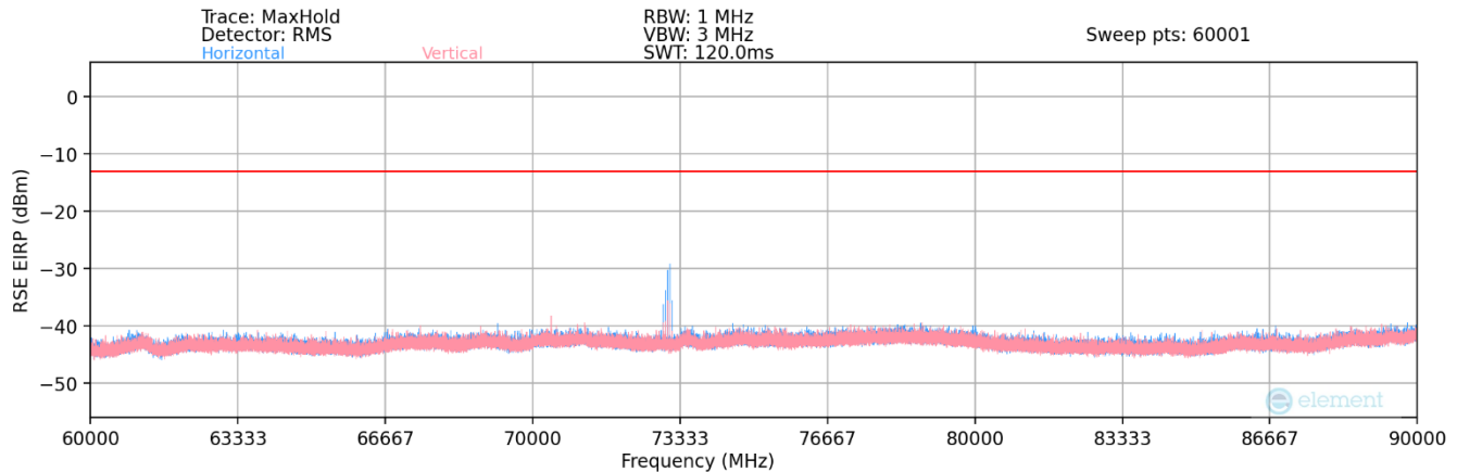
Plot 7-85. Ant 1-n258-R1 Radiated Spurious Plot (3CC QPSK Mid Channel 2Tx)
