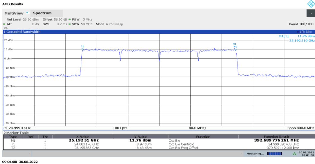
Plot 7-24. Occupied Bandwidth Plot (100MHz-4CC – 64QAM – Mid Channel)
