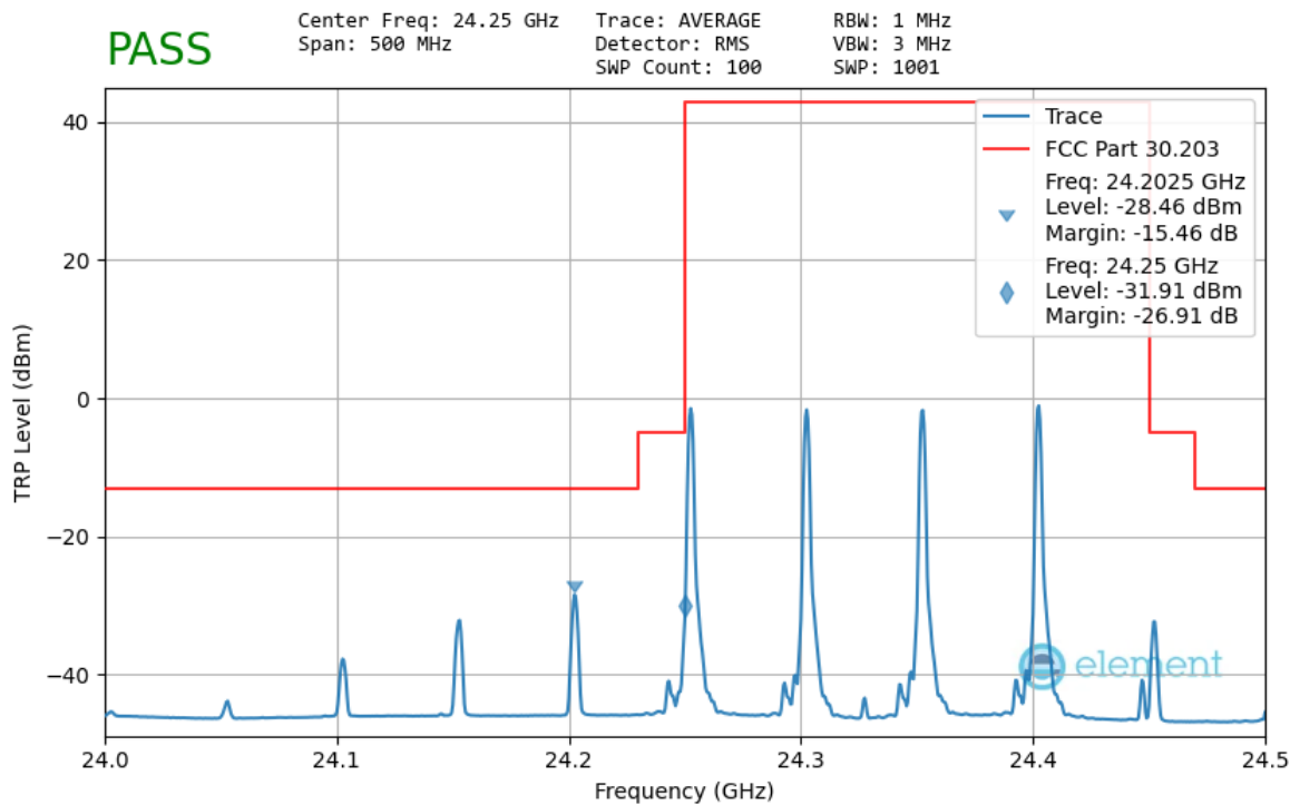
Plot 7-94. Ant 1 Lower Band Edge – TRP (50MHz-4CC – \pi/2 -BPSK 1 RB)
