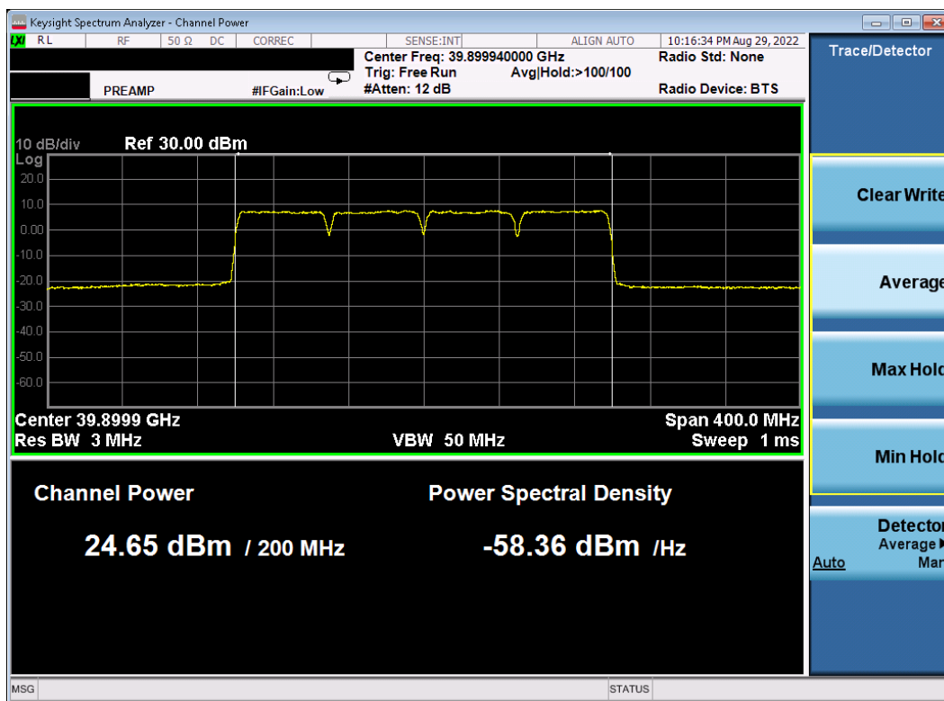
Plot 7-78. Ant1 EIRP Plot (Band n260 – 50MHz-4CC – \pi/2 -BPSK – High Channel)
