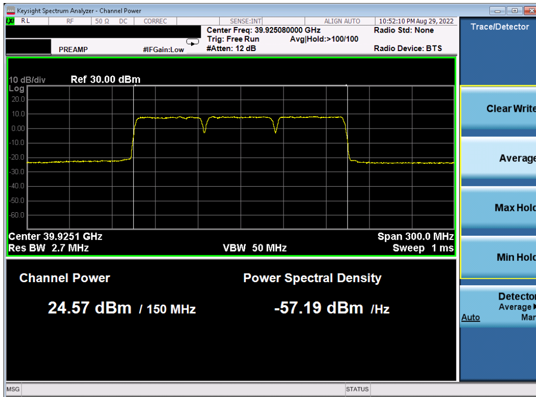
Plot 7-77. Ant1 EIRP Plot (Band n260 – 50MHz-3CC – \pi/2 -BPSK – High Channel)
