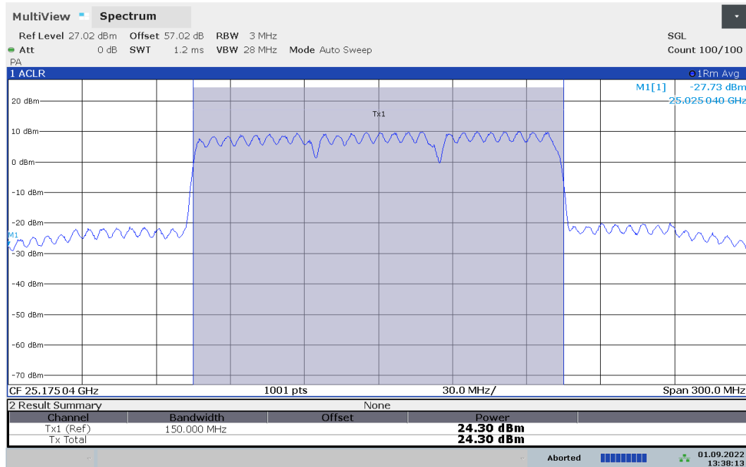
Plot 7-65. Ant2 EIRP Plot (Band n258-R2 - 50MHz-3CC - \pi/2 -BPSK - High Channel)
