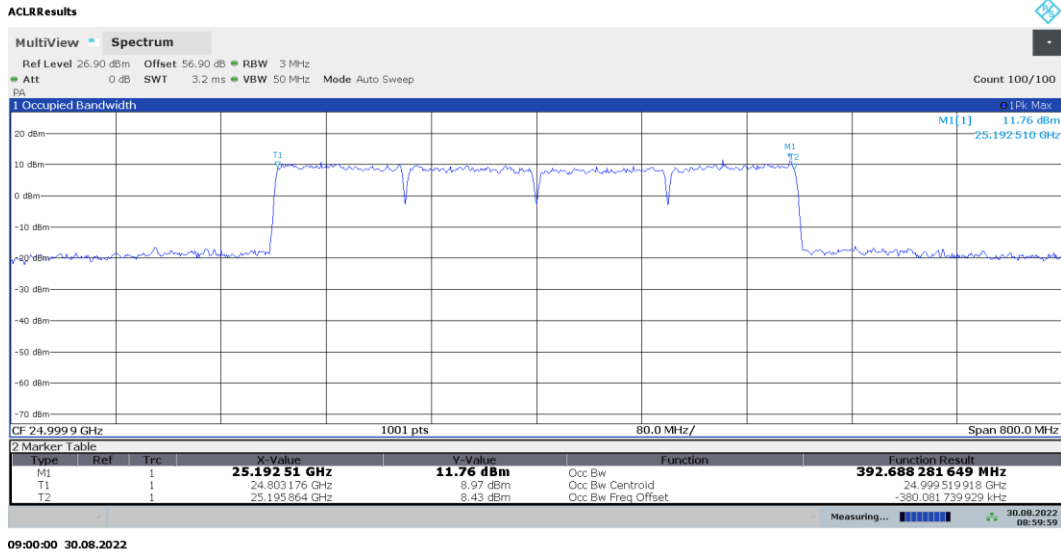
Plot 7-23. Occupied Bandwidth Plot (100MHz-4CC – 16QAM – Mid Channel)
