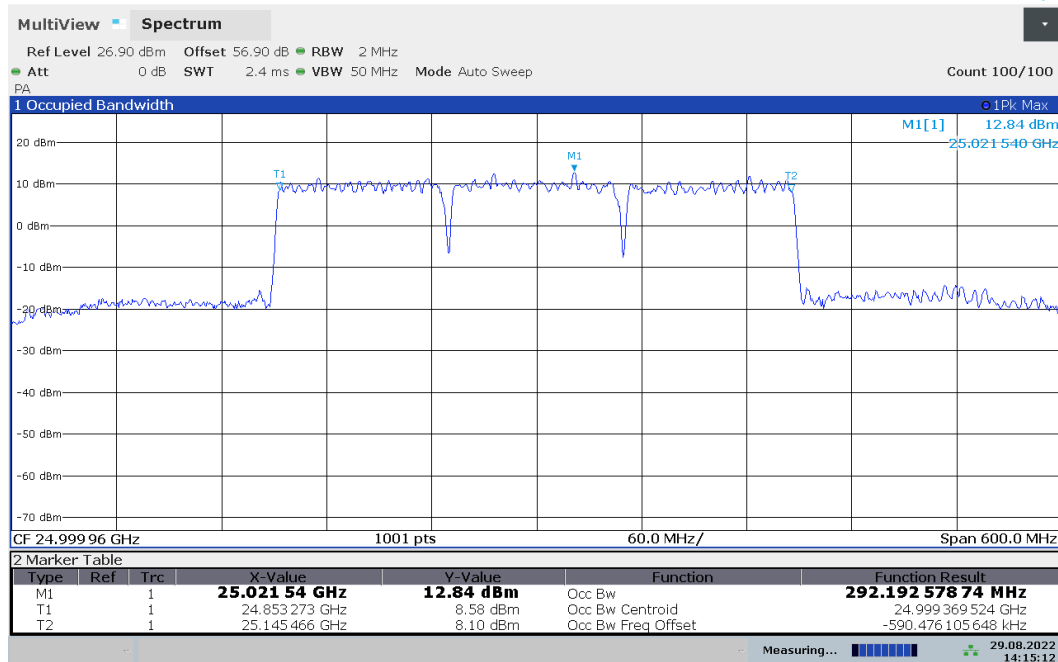
Plot 7-18. Occupied Bandwidth Plot (100MHz-3CC – \pi/2 -BPSK – Mid Channel)
