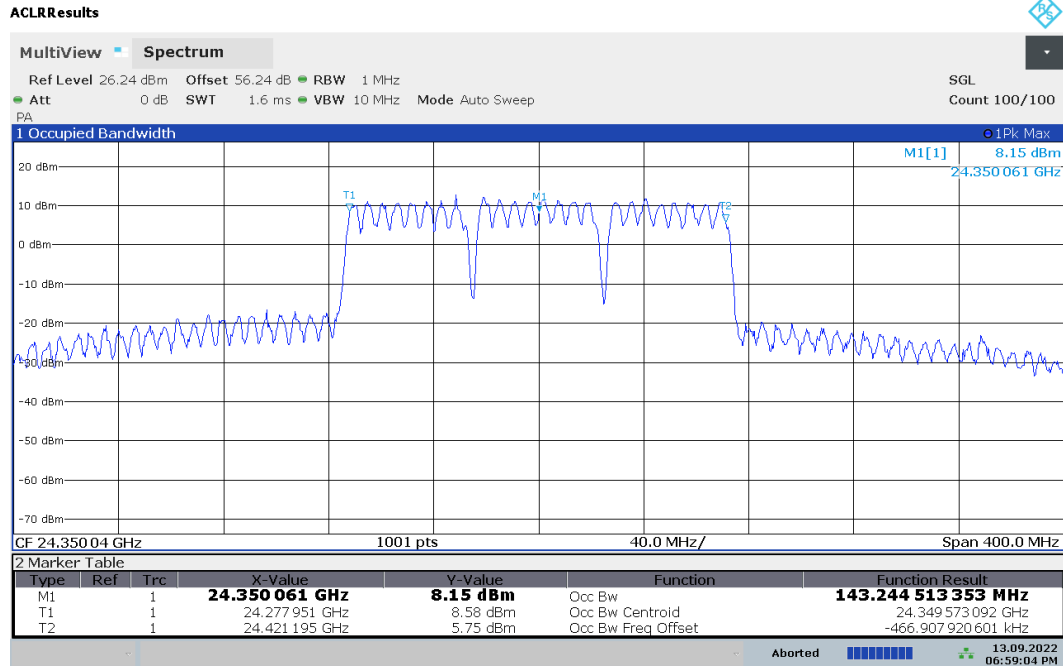
Plot 7-1. Occupied Bandwidth Plot (50MHz-3CC – QPSK – Mid Channel)
