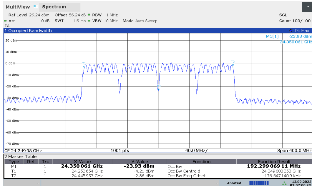
Plot 7-7. Occupied Bandwidth Plot (50MHz-4CC – 16QAM – Mid Channel)
