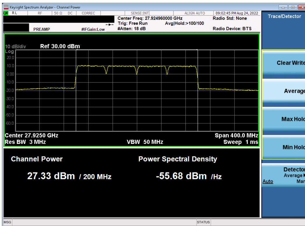
Plot 7-70. Ant1 EIRP Plot (Band n261 – 50MHz-4CC – QPSK – Mid Channel)
