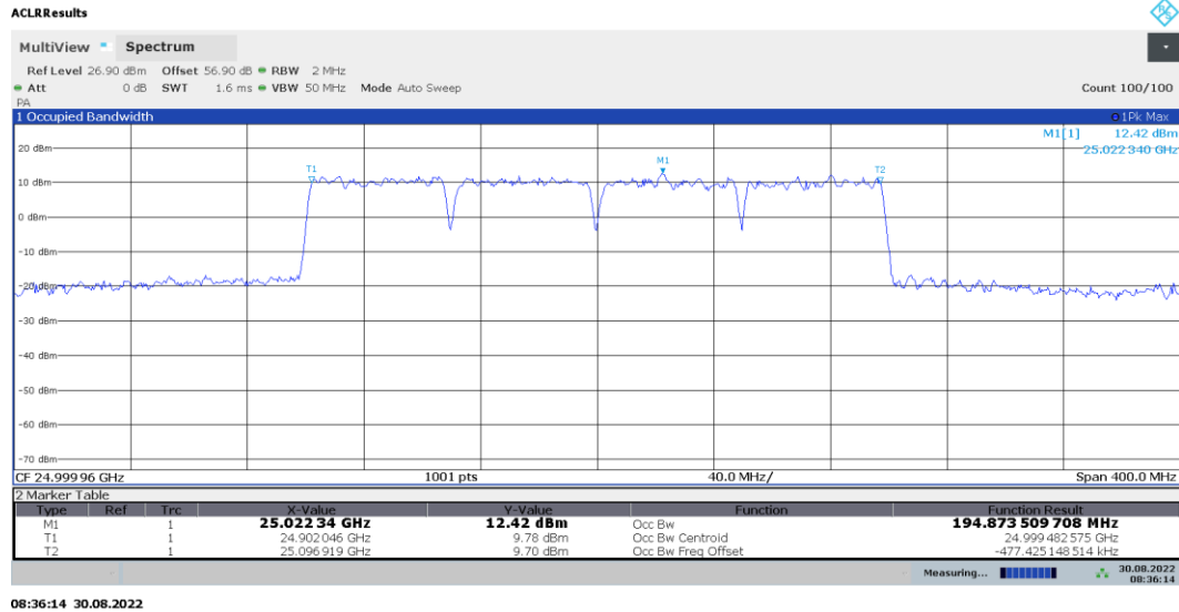
Plot 7-13. Occupied Bandwidth Plot (50MHz-4CC – QPSK – Mid Channel)
