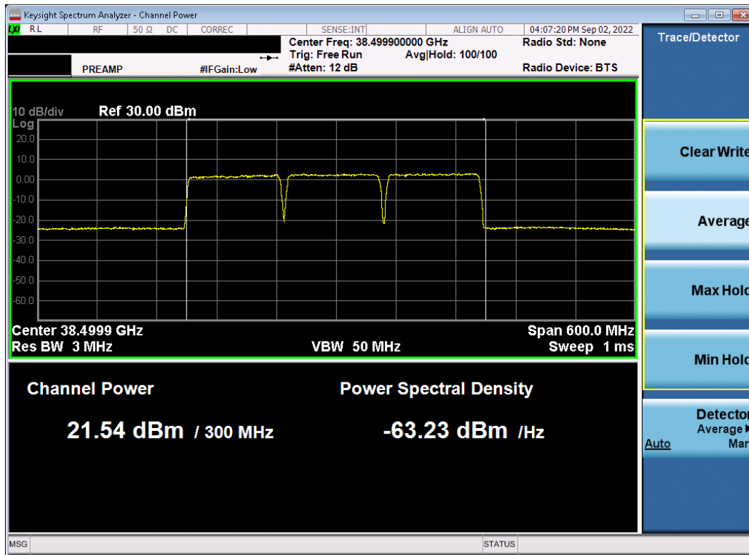
Plot 7-83. Ant2 EIRP Plot (Band n260 – 100MHz-3CC – QPSK – Mid Channel)
