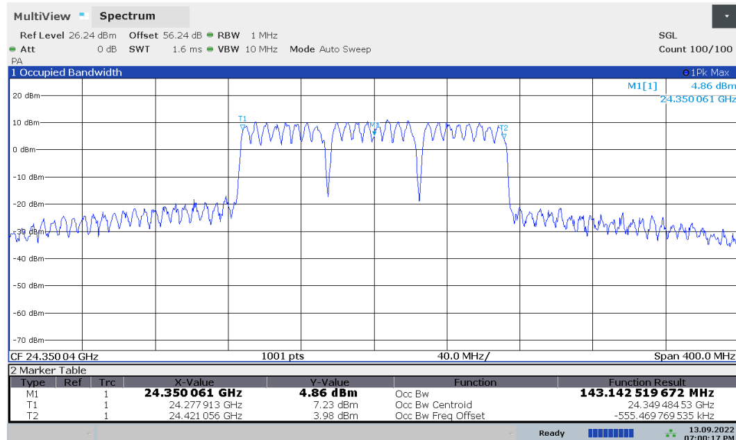
Plot 7-3. Occupied Bandwidth Plot (50MHz-3CC – 16QAM – Mid Channel)
