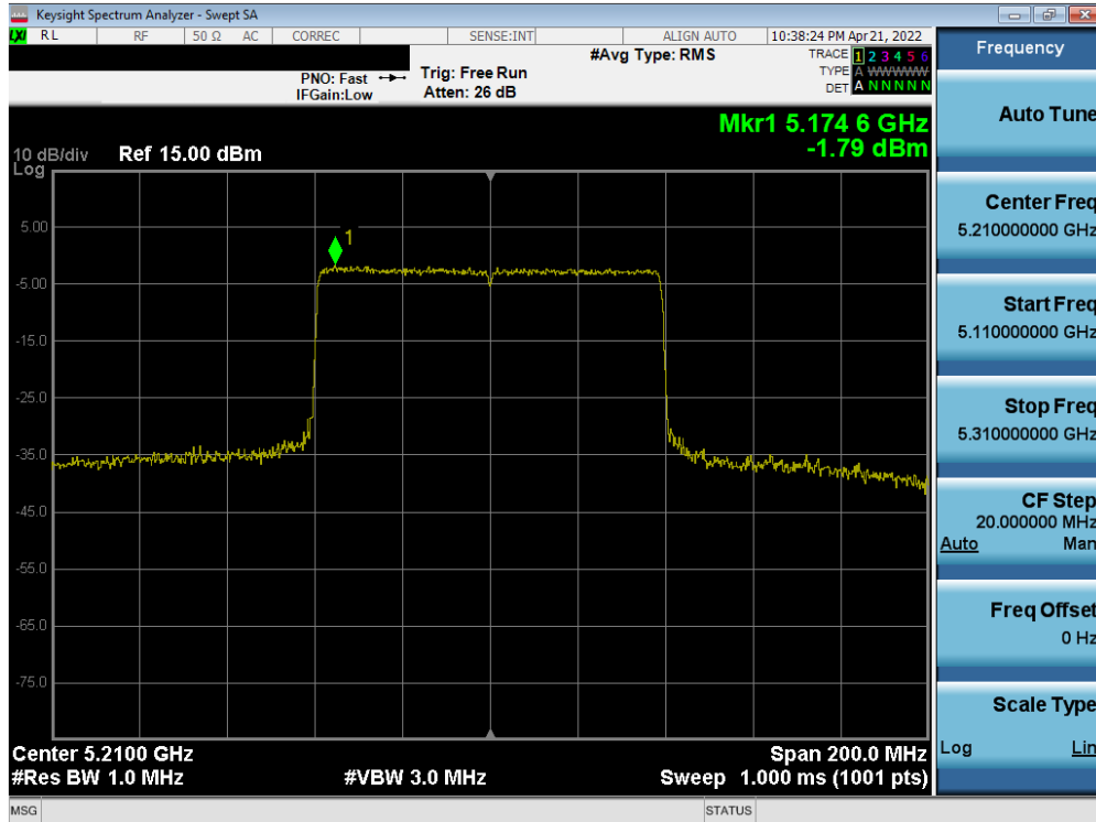
Plot 7-271. Power Spectral Density Plot MIMO ANT2 (80MHz BW 802.11ax – Full Tones (UNII Band 1) – Ch. 42)
