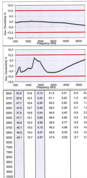
Figure B-19-2 600 – 5800 MHz Body Tissue Equivalent Matter
