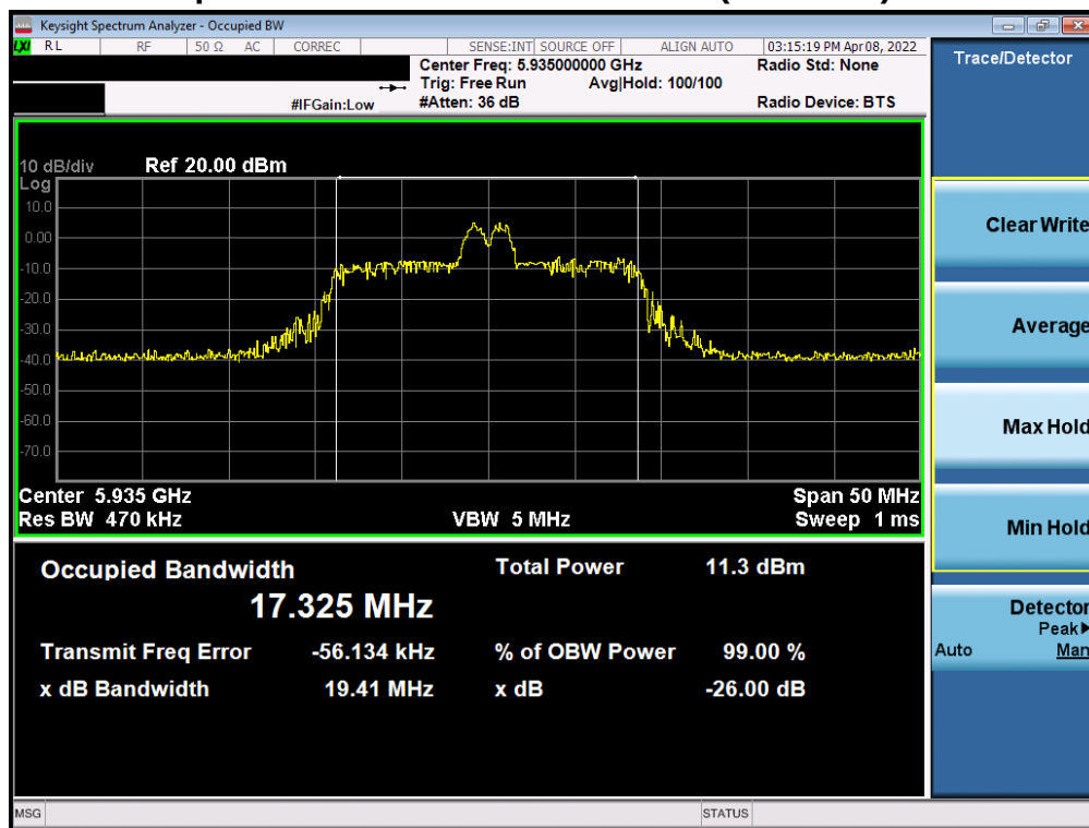
Plot 7-1. Occupied Bandwidth Plot MIMO ANT1 (20MHz BW 802.11ax (26 Tones) UNII Band 5) – Ch. 2
