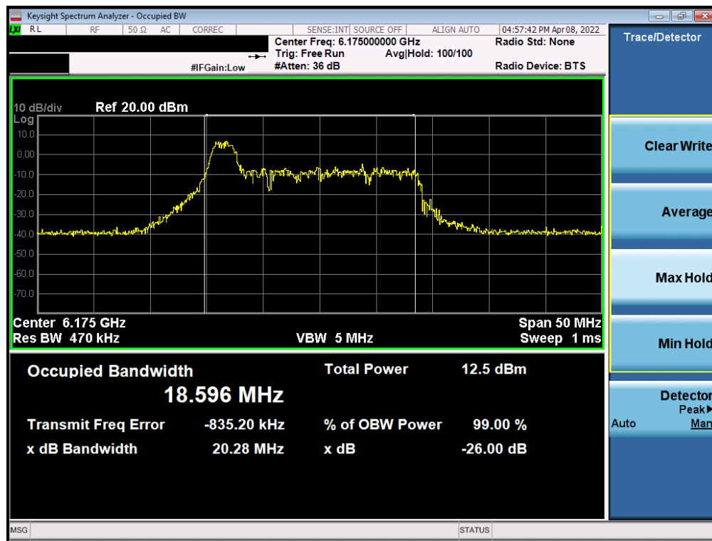
Plot 7-76. Occupied Bandwidth Plot MIMO ANT2 (20MHz BW 802.11ax (26 Tones) (UNII Band 5) – Ch. 45)
