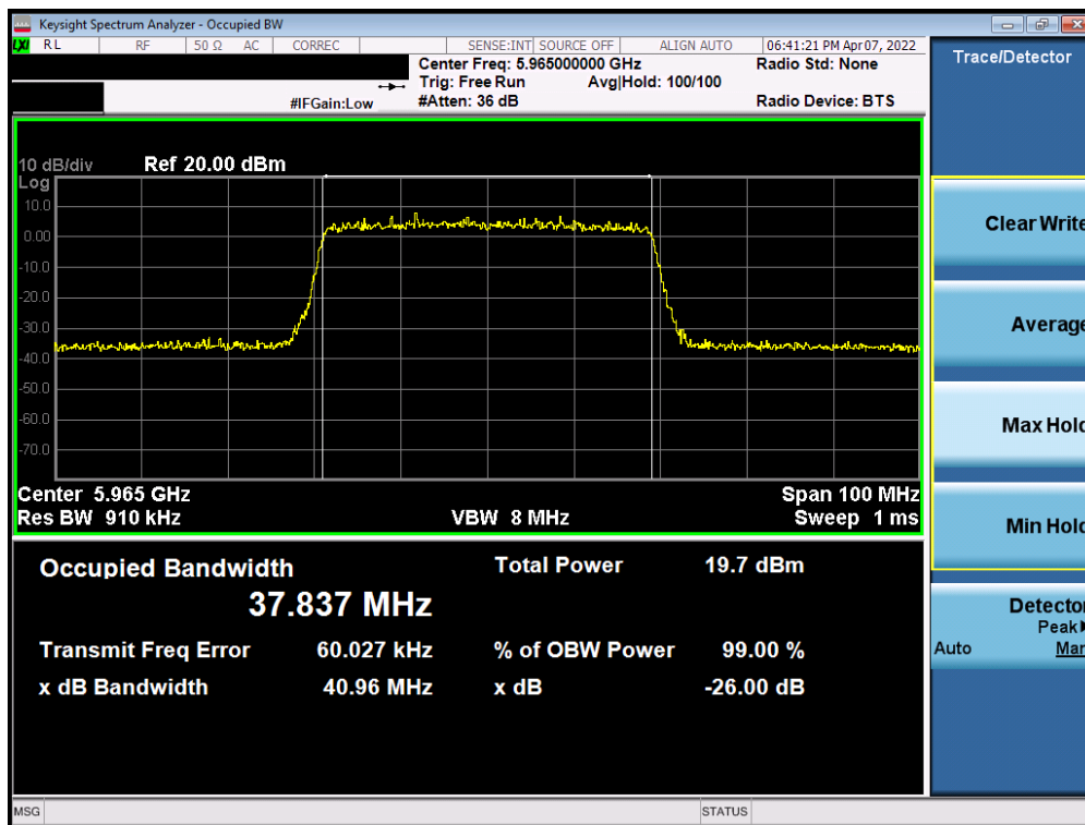
Plot 7-59. 26dB Bandwidth Plot MIMO ANT2 (40MHz 802.11ax (UNII Band 5) – Ch. 3)
