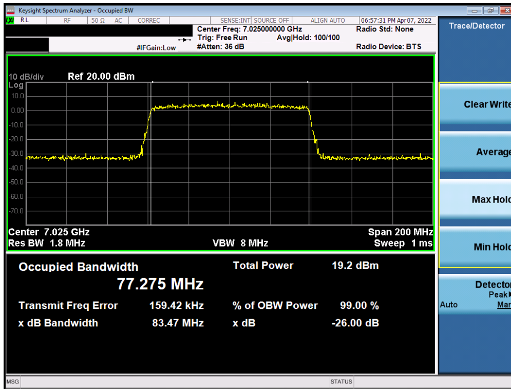
Plot 7-103. 26dB Bandwidth Plot MIMO ANT2 (80MHz 802.11ax (UNII Band 8) – Ch. 215)
