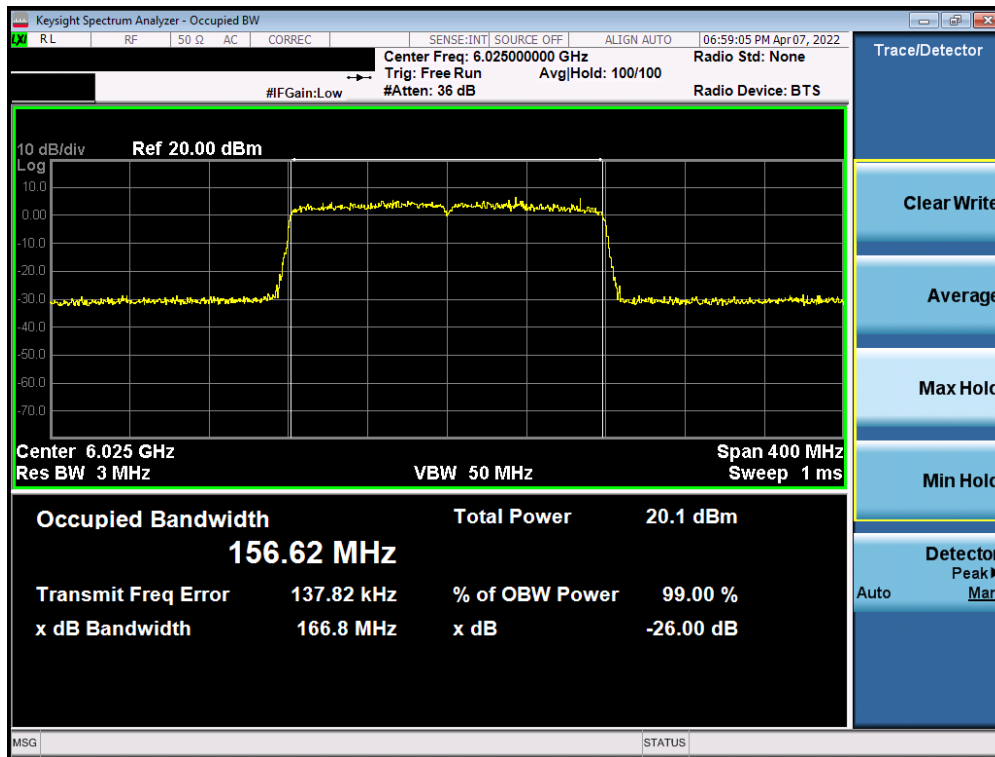
Plot 7-65. 26dB Bandwidth Plot MIMO ANT2 (160MHz 802.11ax (UNII Band 5) – Ch. 15)
