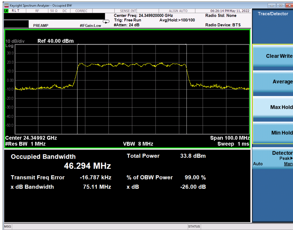
Plot 7-1. Occupied Bandwidth Plot (50MHz-1CC – QPSK – Mid Channel)
