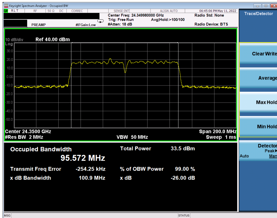
Plot 7-6. Occupied Bandwidth Plot (50MHz-2CC – pi/2-BPSK – Mid Channel)
