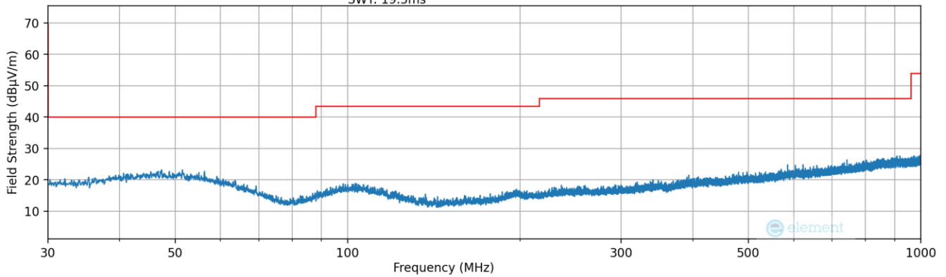
Plot 7-10. Radiated Spurious Plot 30MHz – 1GHz (Pol. V) – Closed
