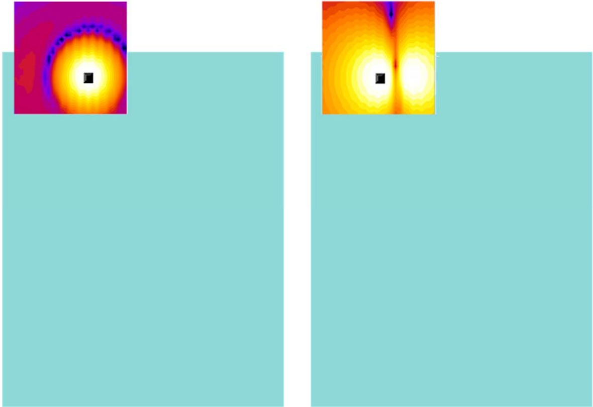
Figure 10-2 T-Coil Scan Overlay Magnetic Field Distributions (OPEN – FRONT)
