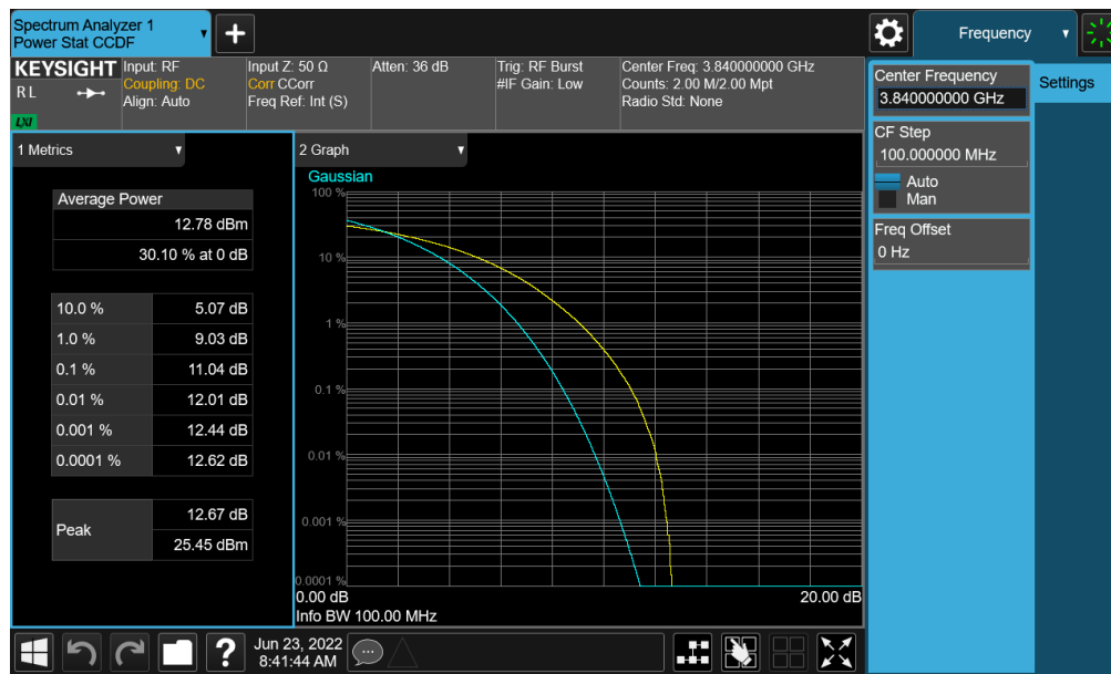
Plot 7-431. PAR Plot (NR Band n77 (C-Band) - 100MHz 256-QAM - Full RB - Antenna D)
