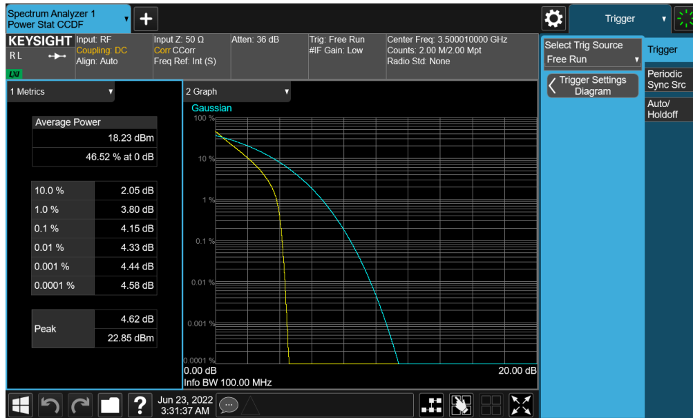
Plot 7-426. PAR Plot (NR Band n77 (DoD) - 100MHz \pi/2 BPSK - Full RB – Antenna D)
