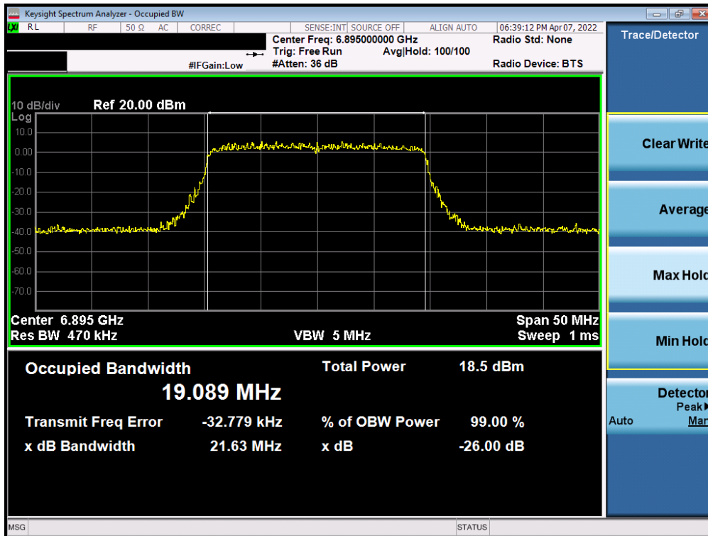
Plot 7-96. 26dB Bandwidth Plot MIMO ANT2 (20MHz 802.11a (UNII Band 8) – Ch. 189)
