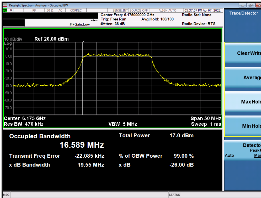
Plot 7-54. 26dB Bandwidth Plot MIMO ANT2 (20MHz 802.11a (UNII Band 5) – Ch. 45)
