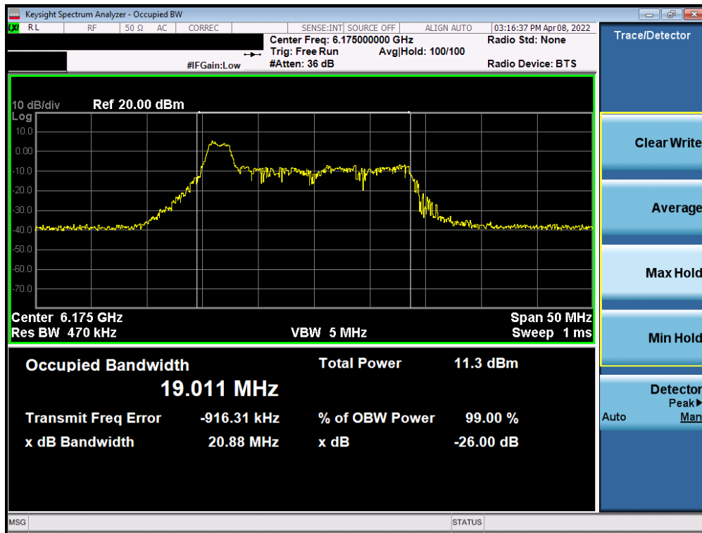
Plot 7-2. Occupied Bandwidth Plot MIMO ANT1 (20MHz BW 802.11ax (26 Tones) (UNII Band 5) – Ch. 45)
