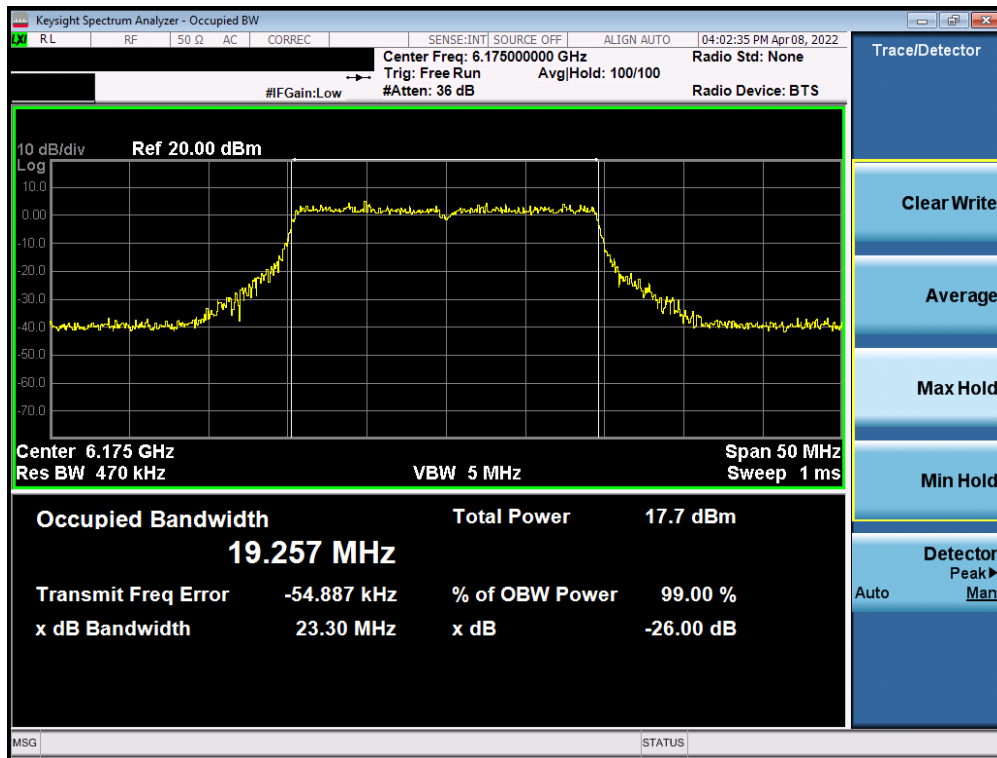
Plot 7-42. Occupied Bandwidth Plot MIMO ANT1 (20MHz BW 802.11ax (Full Tone) (UNII Band 5) – Ch. 45)
