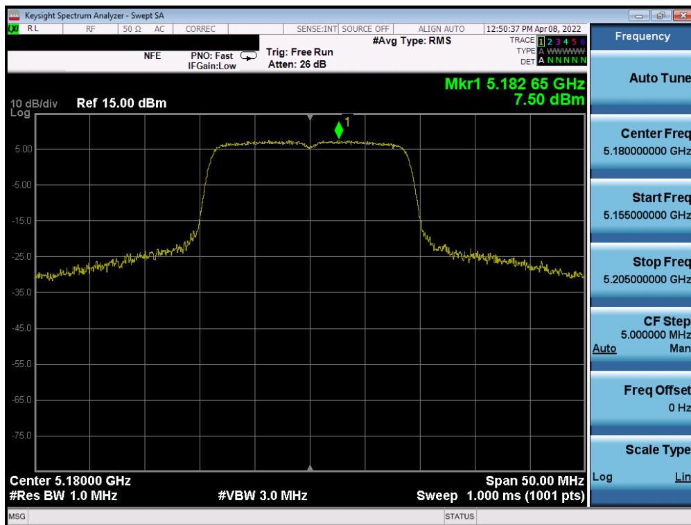
Plot 7-265. Power Spectral Density Plot MIMO ANT2 (20MHz BW 802.11n (UNII Band 1) – Ch. 36)
