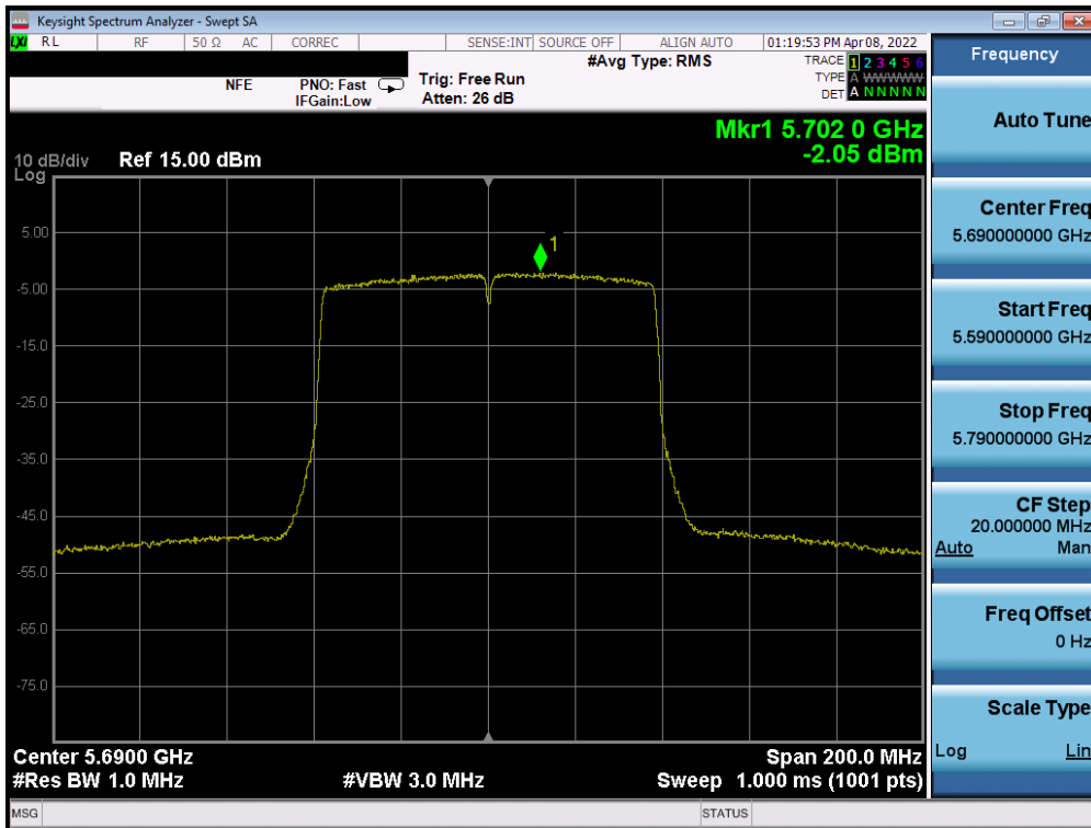
Plot 7-311. Power Spectral Density Plot MIMO ANT2 (80MHz BW 802.11ac (UNII Band 2C) – Ch. 138)
