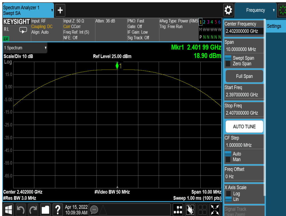
Plot 7-28. Peak Power Plot (Bluetooth (LE), 2Mbps – Ch. 0) – Antenna 1
