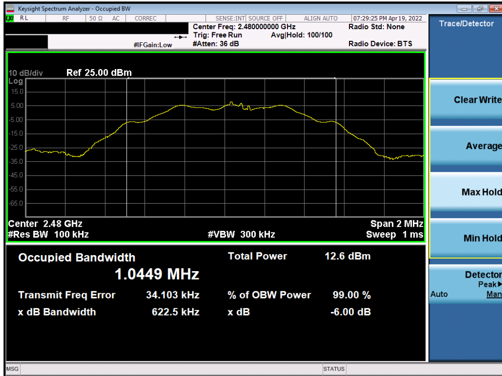
Plot 7-3. 6dB Bandwidth Plot (Bluetooth (LE), 125kbps – Ch. 39) – Antenna 1
