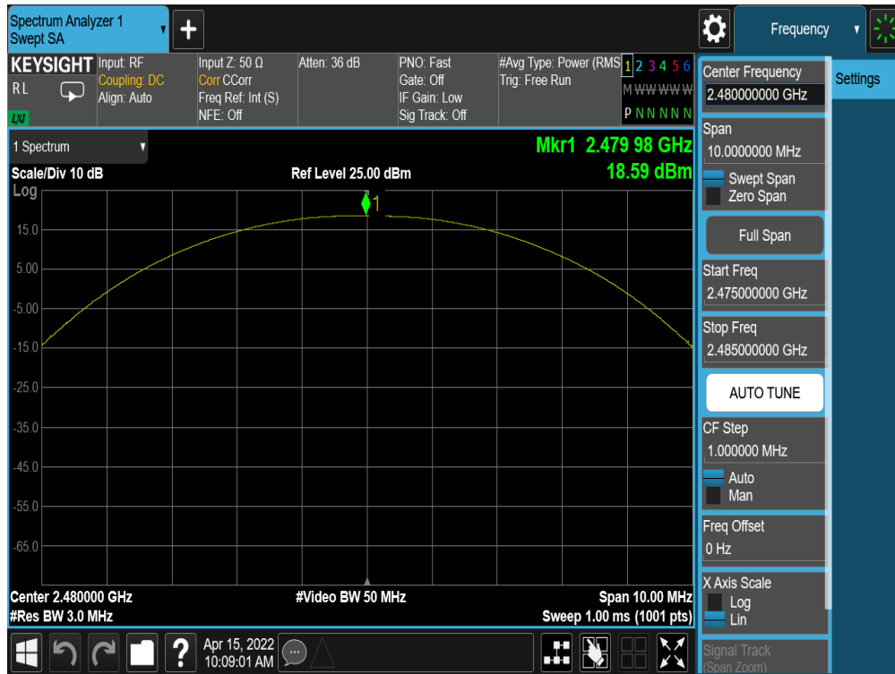
Plot 7-27. Peak Power Plot (Bluetooth (LE), 1Mbps – Ch. 39) – Antenna 1
