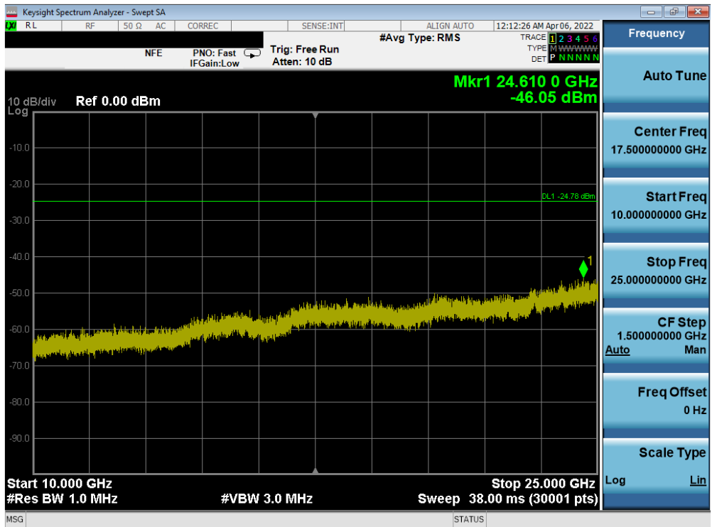
Plot 7-78. Conducted Spurious Plot ANT1 (802.11b – Ch. 6)
