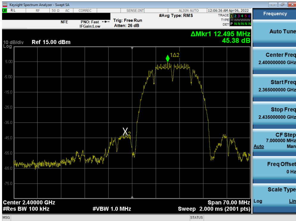
Plot 7-43. Band Edge Plot ANT1 (802.11b – Ch. 1)
