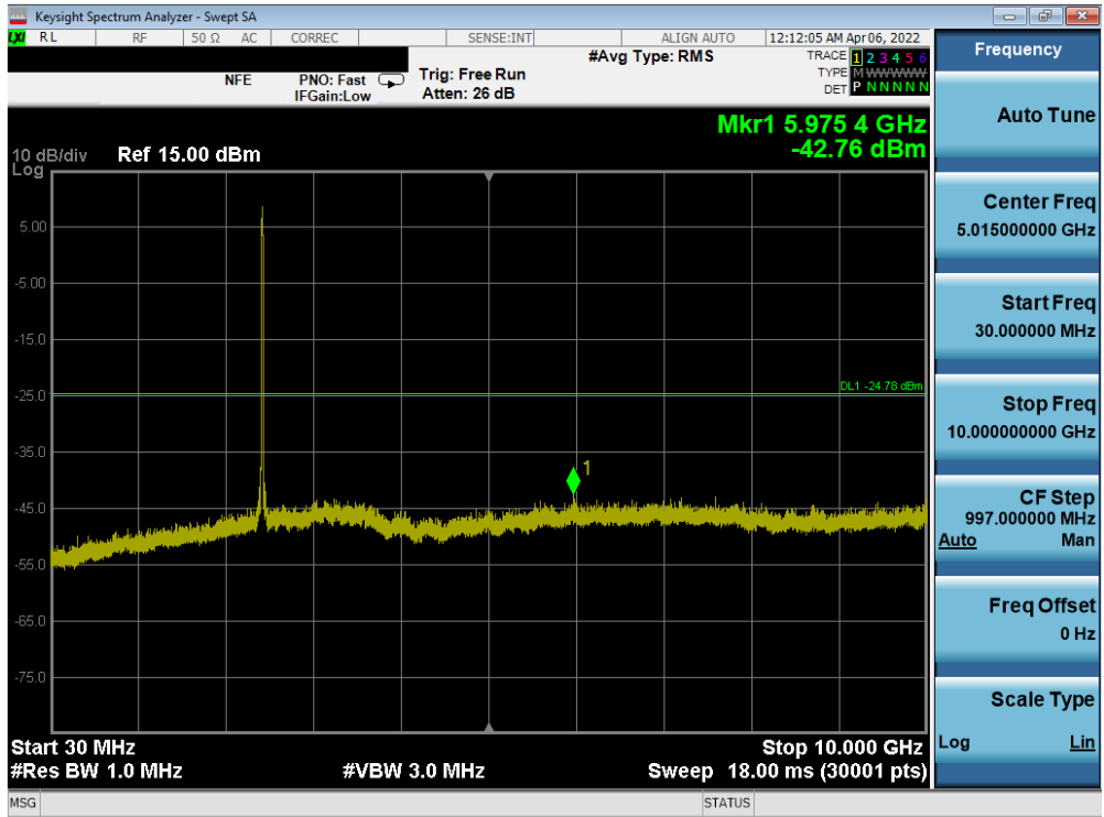
Plot 7-77. Conducted Spurious Plot ANT1 (802.11b – Ch. 6)
