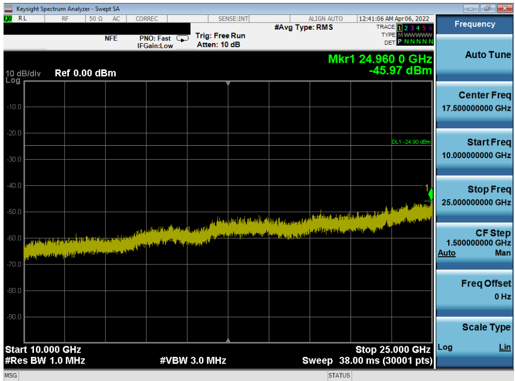
Plot 7-86. Conducted Spurious Plot ANT2 (802.11b – Ch. 11)
