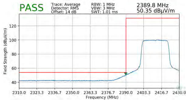
Plot 7-103. Radiated Restricted Lower Band Edge Measurement MIMO (Average) - Open
