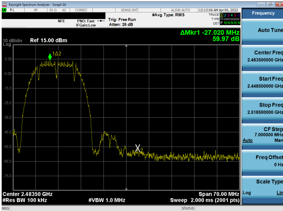
Plot 7-44. Band Edge Plot ANT1 (802.11b – Ch. 11)
