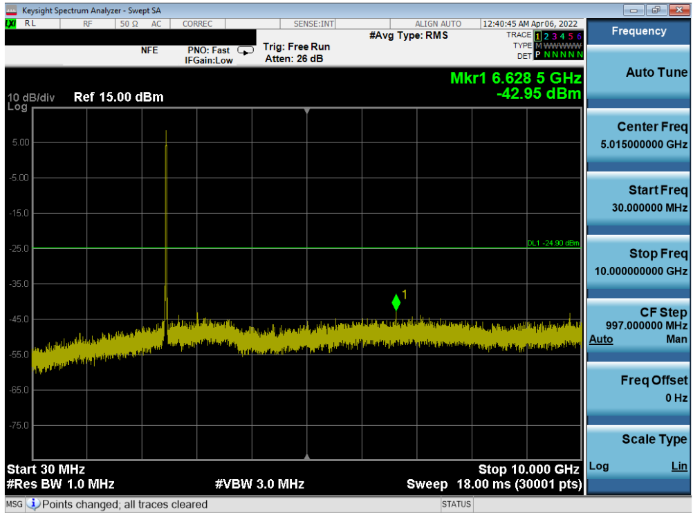
Plot 7-85. Conducted Spurious Plot ANT2 (802.11b – Ch. 11)
