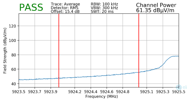
Plot 7-355. Radiated Lower Band Edge Plot MIMO (Average – UNII Band 5)
