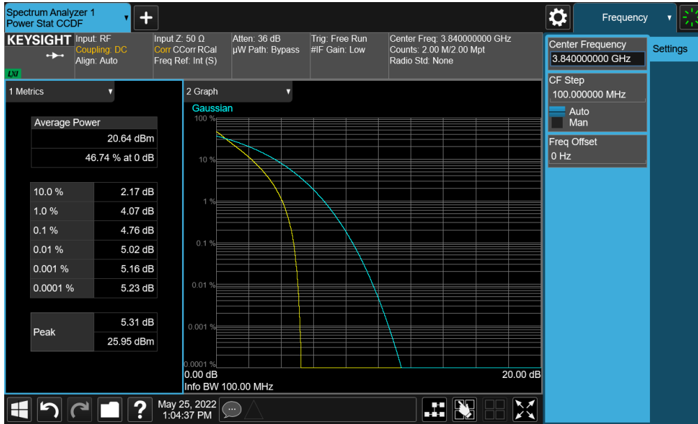
Plot 7-355. PAR Plot (NR Band n77 (C-Band) - 100MHz DFT-s-OFDM BPSK - Full RB - Ant G)
