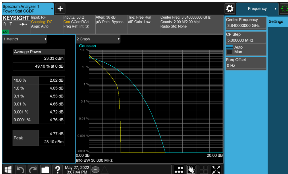
Plot 7-343. PAR Plot (NR Band n77 (C-Band) - 30MHz DFT-s-OFDM BPSK - Full RB - Ant E)
