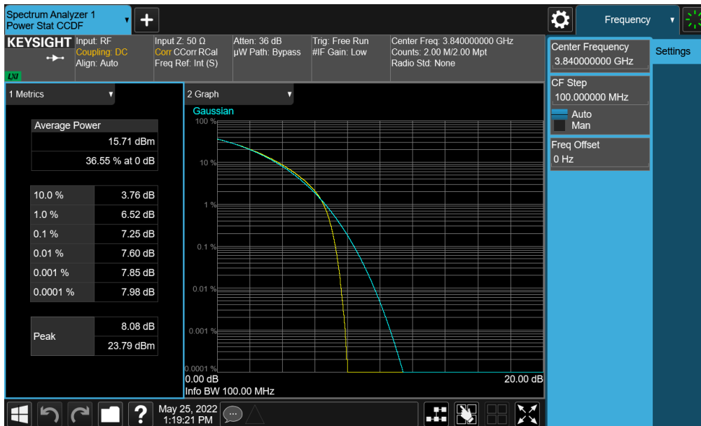
Plot 7-359. PAR Plot (NR Band n77 (C-Band) - 100MHz CP-OFDM QPSK - Full RB - Ant D)
