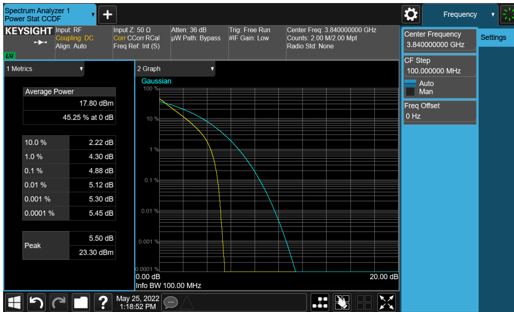
Plot 7-358. PAR Plot (NR Band n77 (C-Band) - 100MHz DFT-s-OFDM BPSK - Full RB - Ant D)
