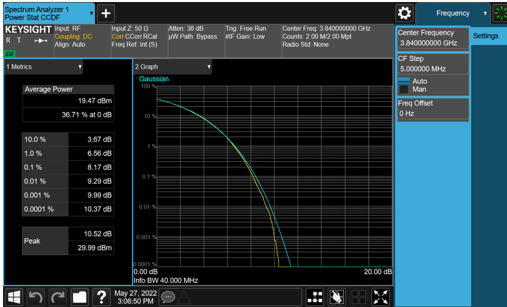
Plot 7-342. PAR Plot (NR Band n77 (C-Band) - 40MHz CP-OFDM 256-QAM - Full RB - Ant E)
