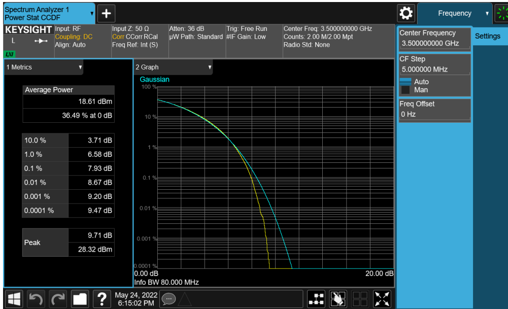
Plot 7-369. PAR Plot (NR Band n77 (DoD) - 80MHz CP-OFDM 256-QAM - Full RB - Ant F)
