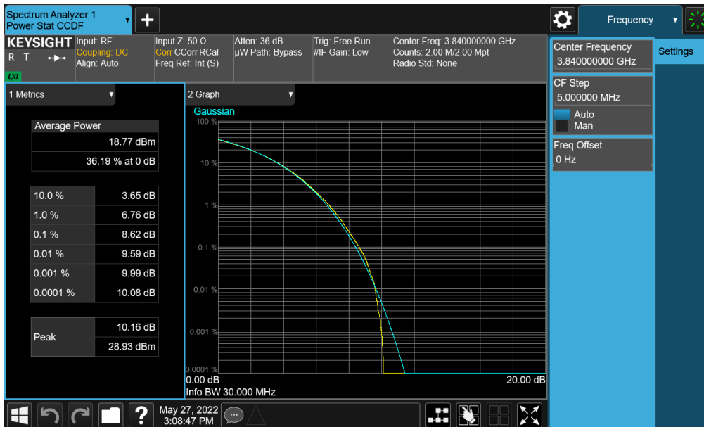
Plot 7-345. PAR Plot (NR Band n77 (C-Band) - 30MHz CP-OFDM 256-QAM - Full RB - Ant E)
