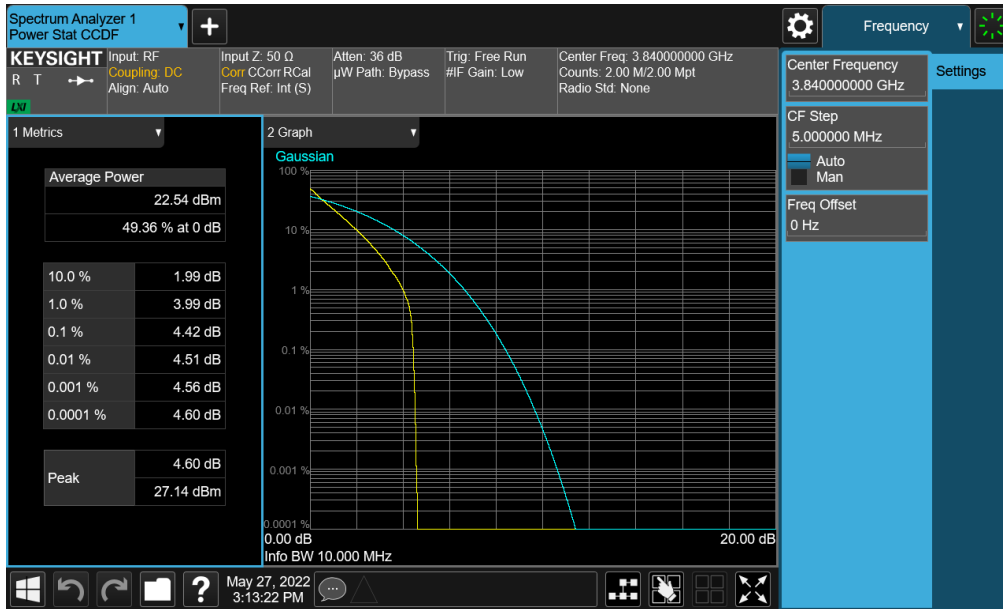
Plot 7-352. PAR Plot (NR Band n77 (C-Band) - 10MHz DFT-s-OFDM BPSK - Full RB - Ant E)
