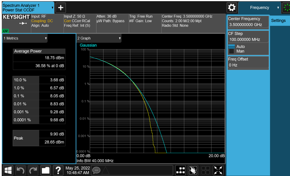
Plot 7-381. PAR Plot (NR Band n77 (DoD) - 40MHz CP-OFDM 256-QAM - Full RB - Ant F)
