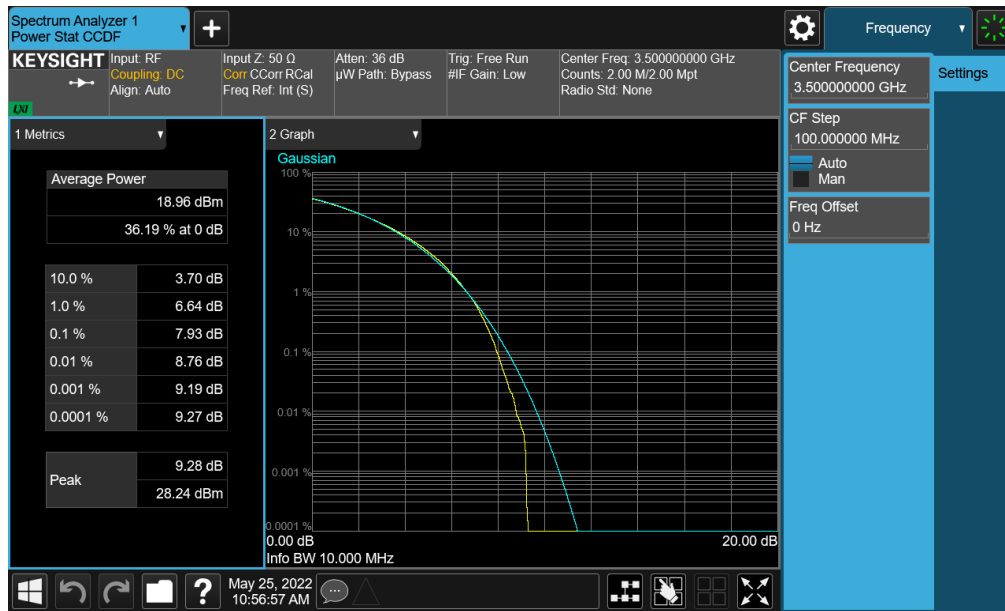
Plot 7-393. PAR Plot (NR Band n77 (DoD) - 10MHz CP-OFDM 256-QAM - Full RB - Ant F)
