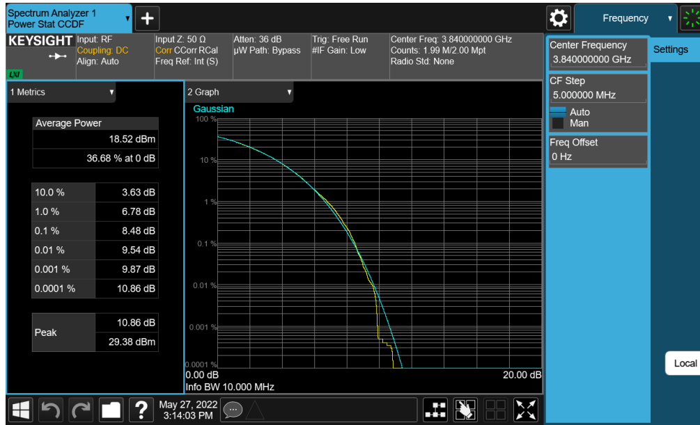
Plot 7-354. PAR Plot (NR Band n77 (C-Band) - 10MHz CP-OFDM 256-QAM - Full RB - Ant E)
