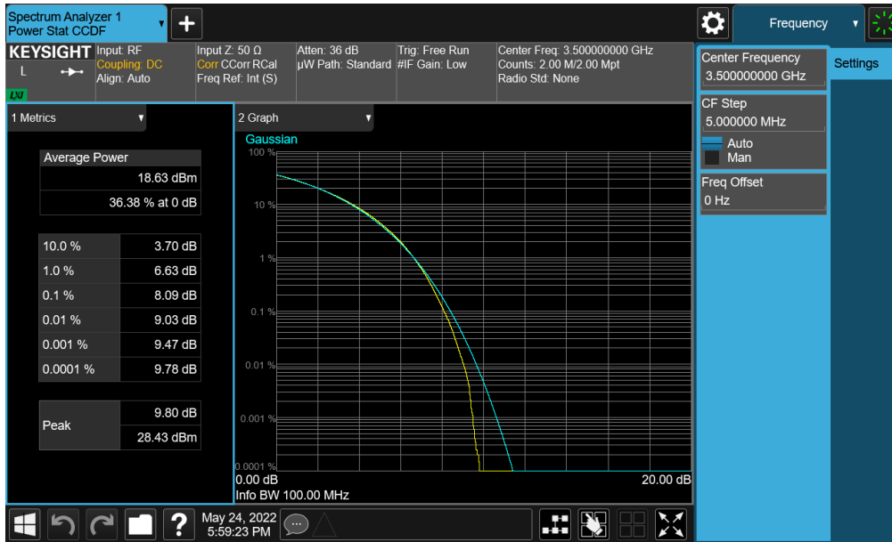
Plot 7-363. PAR Plot (NR Band n77 (DoD) - 100MHz CP-OFDM 256-QAM - Full RB - Ant F)
