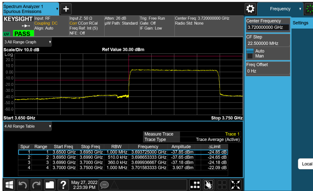
Plot 7-227. Lower ACP Plot (NR Band n77 (C-Band) - 40MHz CP-OFDM-QPSK – Full RB - Ant E)
