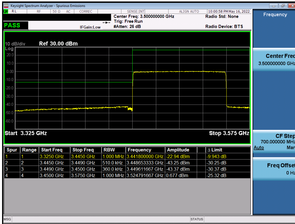
Plot 7-241. Lower ACP Plot (NR Band n77 (DoD) - 100MHz CP-OFDM-QPSK – Full RB - Ant F)
