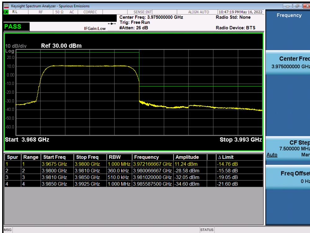
Plot 7-214. Upper ACP Plot (NR Band n77 (C-Band) - 10MHz CP-OFDM-QPSK – Full RB - Ant F)
