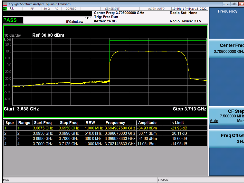
Plot 7-213. Lower ACP Plot (NR Band n77 (C-Band) - 10MHz CP-OFDM-QPSK – Full RB - Ant F)
