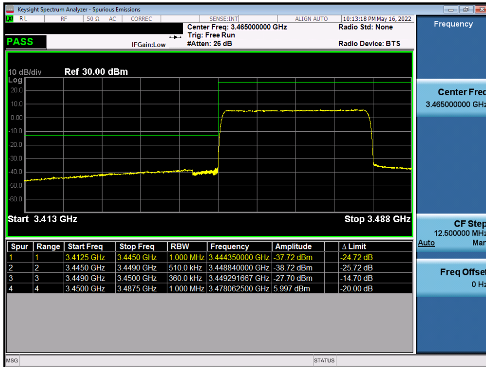
Plot 7-255. Lower ACP Plot (NR Band n77 (DoD) - 30MHz CP-OFDM-QPSK – Full RB - Ant F)
