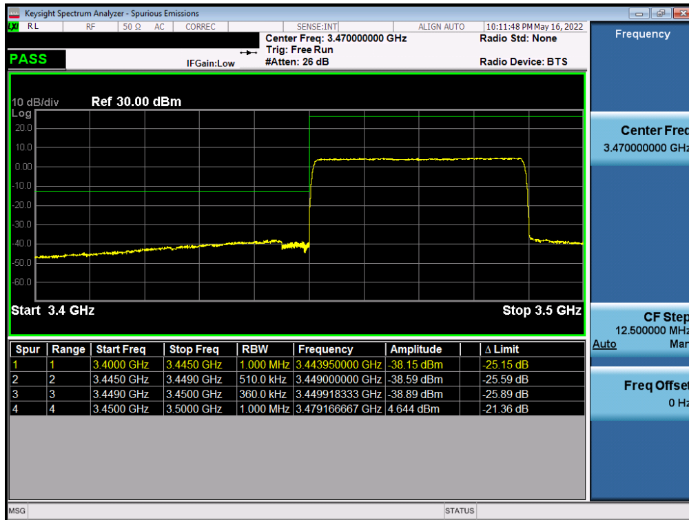
Plot 7-253. Lower ACP Plot (NR Band n77 (DoD) - 40MHz CP-OFDM-QPSK – Full RB - Ant F)
