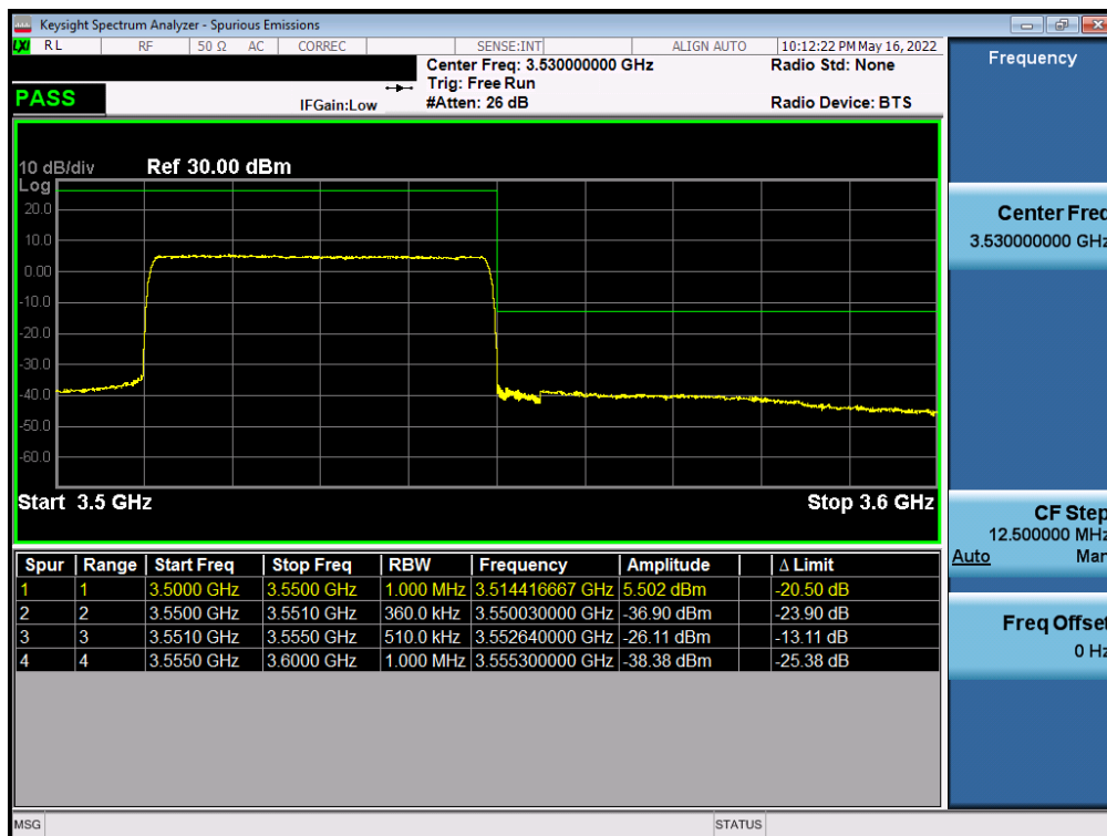
Plot 7-254. Upper ACP Plot (NR Band n77 (DoD) - 40MHz CP-OFDM-QPSK – Full RB - Ant F)
