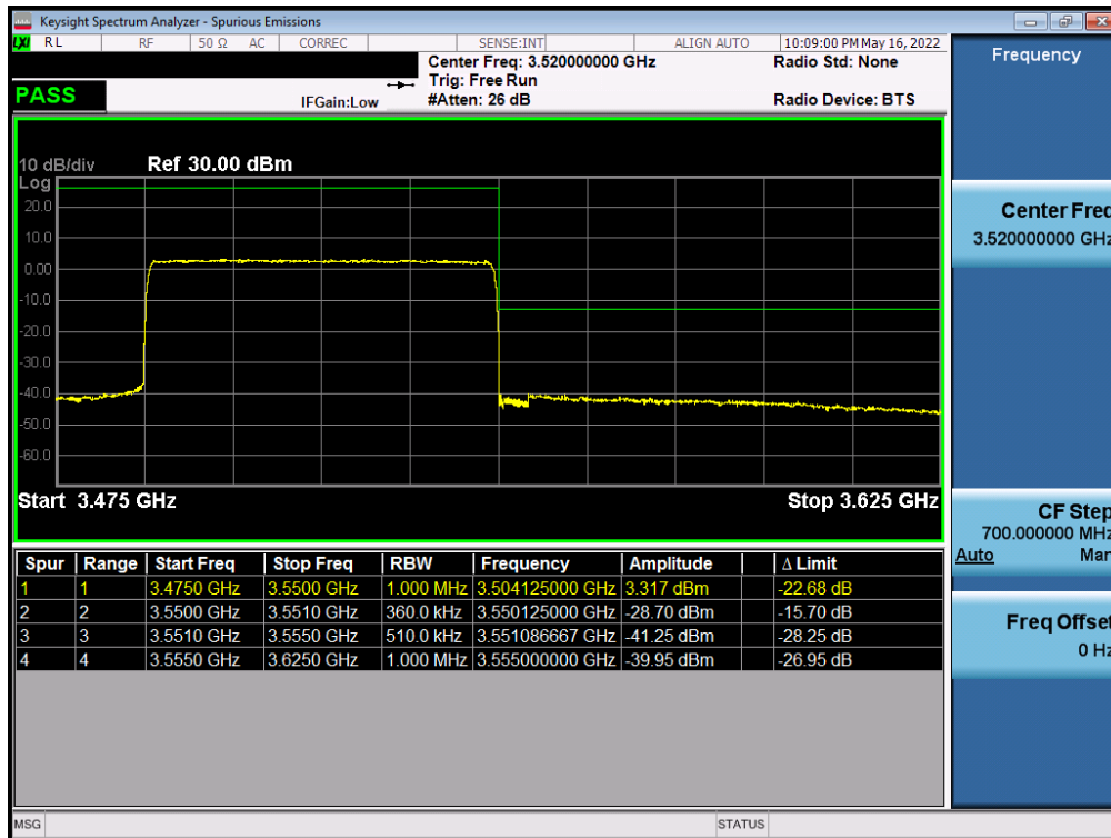
Plot 7-250. Upper ACP Plot (NR Band n77 (DoD) - 60MHz CP-OFDM-QPSK – Full RB - Ant F)
