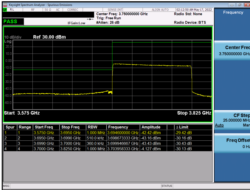
Plot 7-239. Lower ACP Plot (NR Band n77 (C-Band) - 100MHz CP-OFDM-QPSK – Full RB - Ant D)
