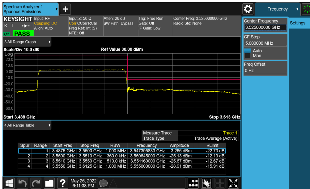
Plot 7-274. Upper ACP Plot (NR Band n77 (DoD) - 50MHz CP-OFDM-QPSK – Full RB - Ant E)
