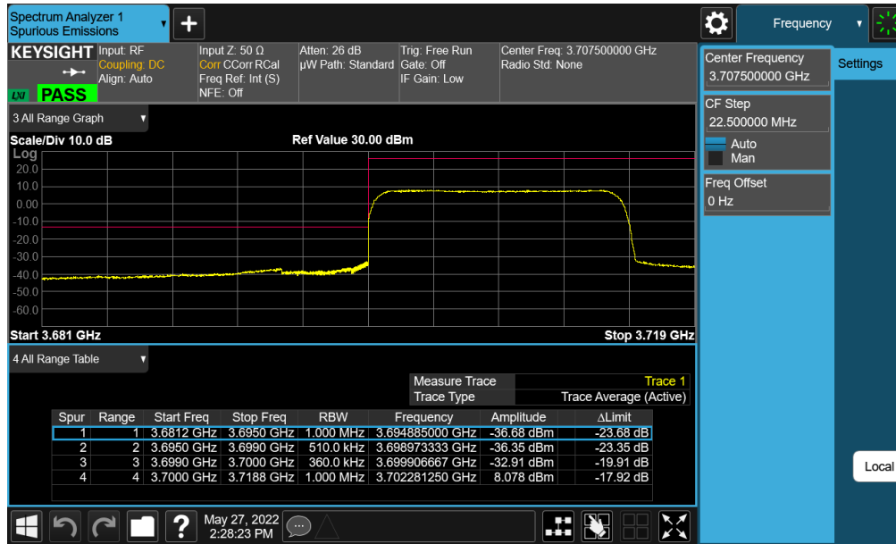
Plot 7-233. Lower ACP Plot (NR Band n77 (C-Band) - 15MHz CP-OFDM-QPSK – Full RB - Ant E)
