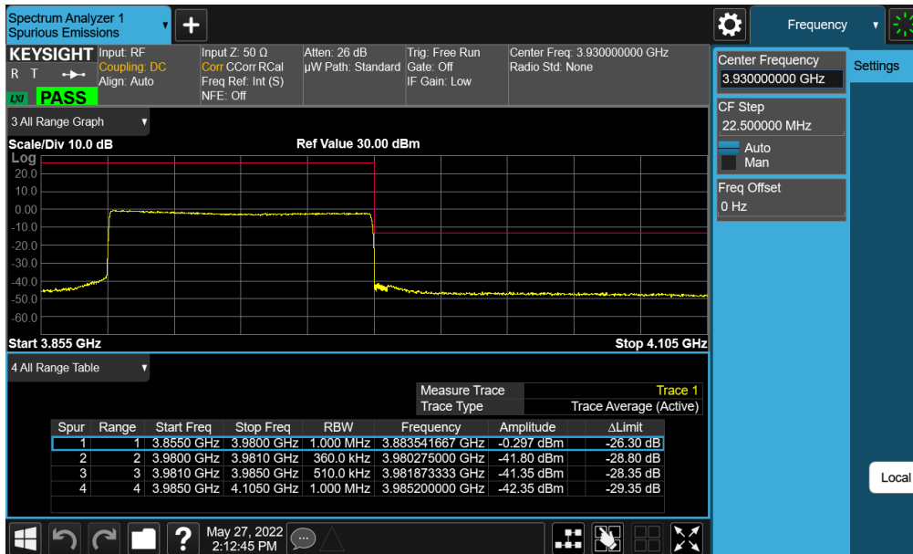
Plot 7-216. Upper ACP Plot (NR Band n77 (C-Band) - 100MHz CP-OFDM-QPSK – Full RB - Ant E)
