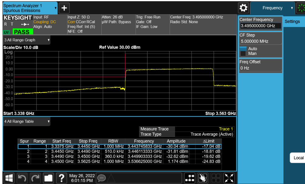
Plot 7-265. Lower ACP Plot (NR Band n77 (DoD) - 90MHz CP-OFDM-QPSK – Full RB - Ant E)
