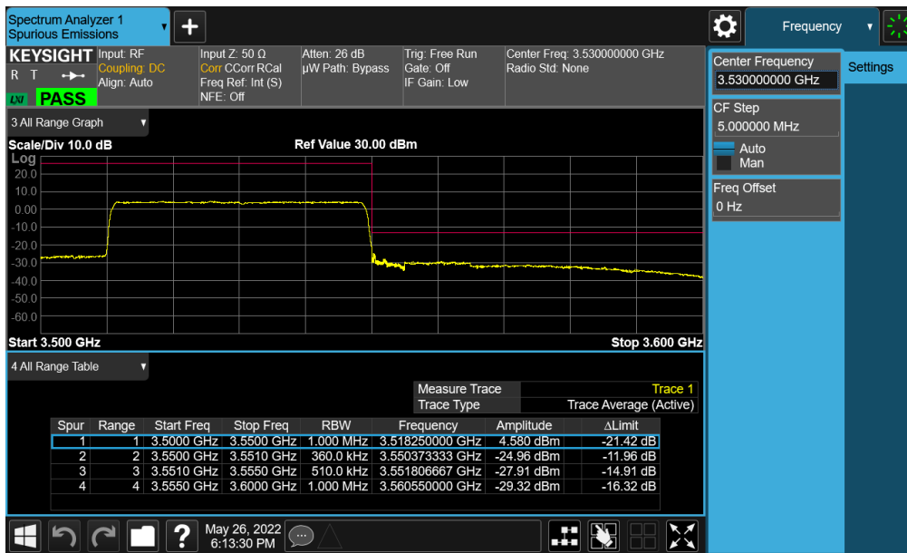
Plot 7-276. Upper ACP Plot (NR Band n77 (DoD) - 40MHz CP-OFDM-QPSK – Full RB - Ant E)
