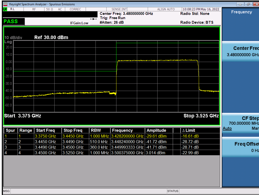
Plot 7-249. Lower ACP Plot (NR Band n77 (DoD) - 60MHz CP-OFDM-QPSK – Full RB - Ant F)
