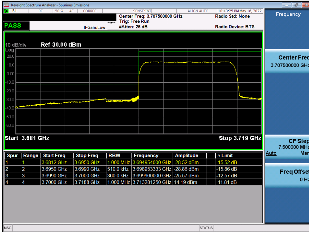
Plot 7-211. Lower ACP Plot (NR Band n77 (C-Band) - 15MHz CP-OFDM-QPSK – Full RB - Ant F)
