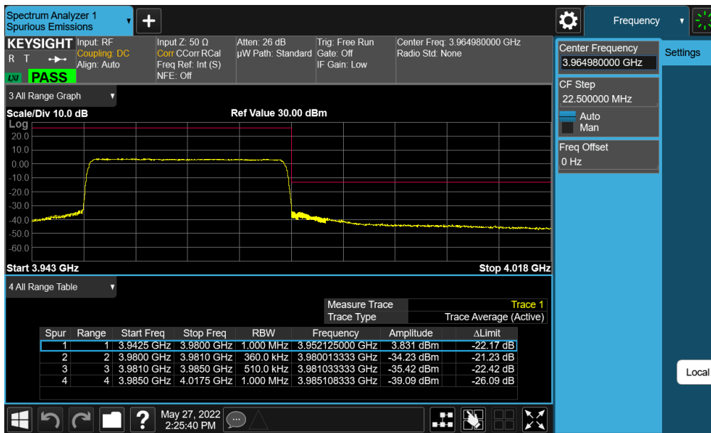
Plot 7-230. Upper ACP Plot (NR Band n77 (C-Band) - 30MHz CP-OFDM-QPSK – Full RB - Ant E)
