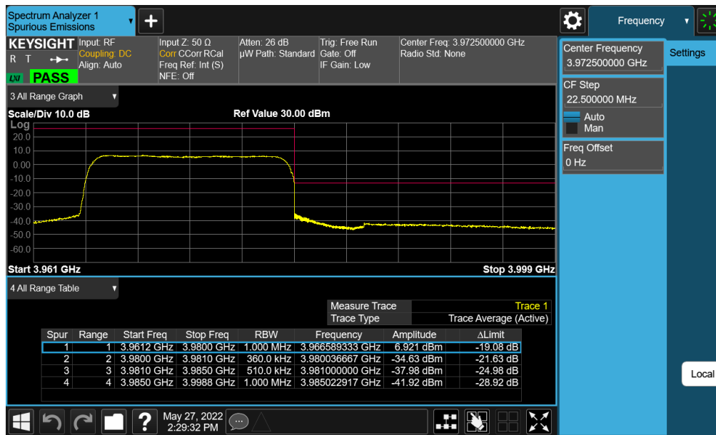
Plot 7-234. Upper ACP Plot (NR Band n77 (C-Band) - 15MHz CP-OFDM-QPSK – Full RB - Ant E)
