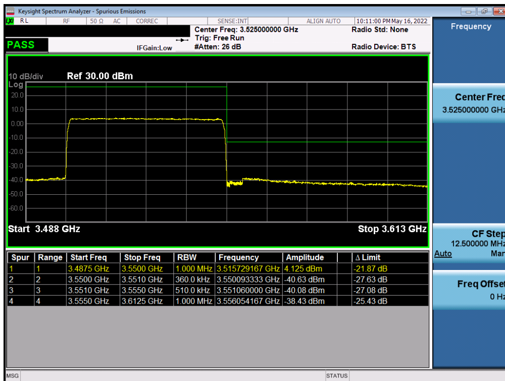
Plot 7-252. Upper ACP Plot (NR Band n77 (DoD) - 50MHz CP-OFDM-QPSK – Full RB - Ant F)
