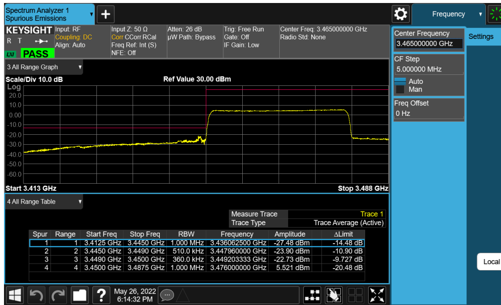
Plot 7-277. Lower ACP Plot (NR Band n77 (DoD) - 30MHz CP-OFDM-QPSK – Full RB - Ant E)
