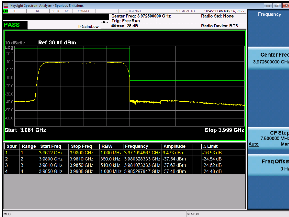
Plot 7-212. Upper ACP Plot (NR Band n77 (C-Band) - 15MHz CP-OFDM-QPSK – Full RB - Ant F)
