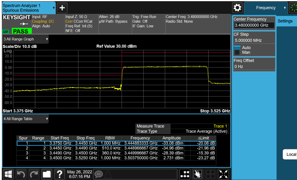
Plot 7-271. Lower ACP Plot (NR Band n77 (DoD) - 60MHz CP-OFDM-QPSK – Full RB - Ant E)
