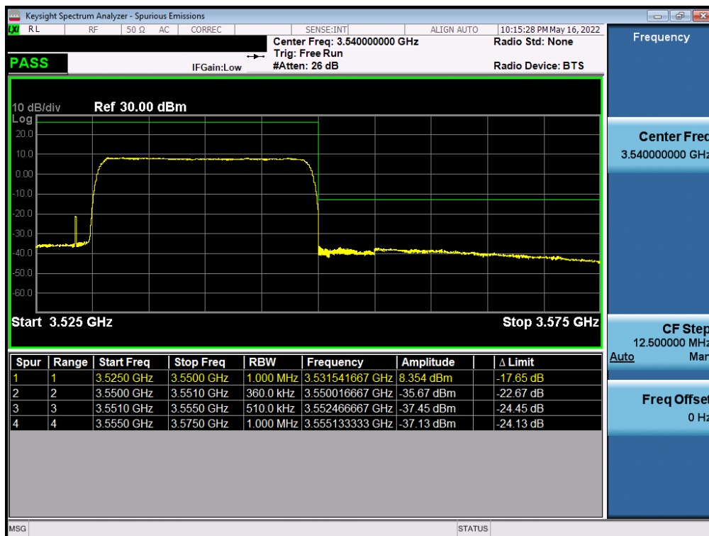
Plot 7-258. Upper ACP Plot (NR Band n77 (DoD) - 20MHz CP-OFDM-QPSK – Full RB - Ant F)
