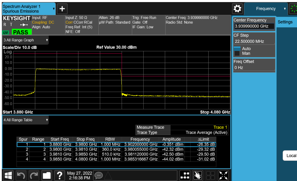
Plot 7-220. Upper ACP Plot (NR Band n77 (C-Band) - 80MHz CP-OFDM-QPSK – Full RB - Ant E)
