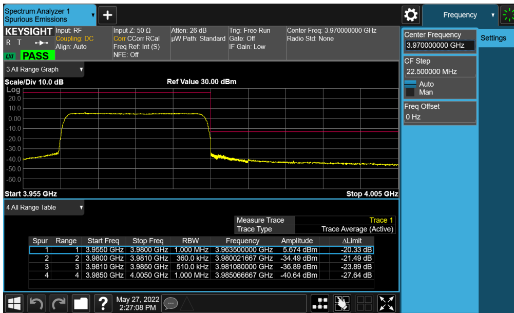
Plot 7-232. Upper ACP Plot (NR Band n77 (C-Band) - 20MHz CP-OFDM-QPSK – Full RB - Ant E)
