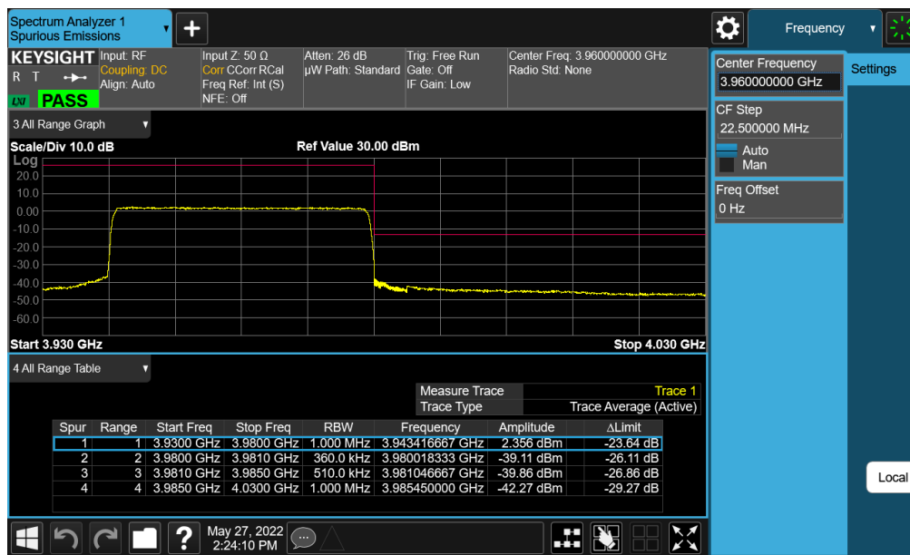
Plot 7-228. Upper ACP Plot (NR Band n77 (C-Band) - 40MHz CP-OFDM-QPSK – Full RB - Ant E)
