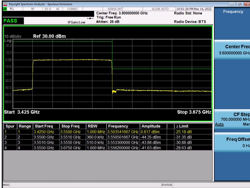
Plot 7-242. Upper ACP Plot (NR Band n77 (DoD) - 100MHz CP-OFDM-QPSK – Full RB - Ant F)
