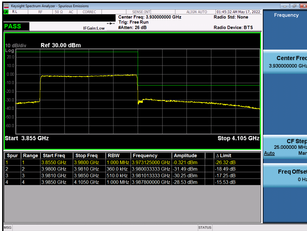
Plot 7-238. Upper ACP Plot (NR Band n77 (C-Band) - 100MHz CP-OFDM-QPSK – Full RB - Ant G)
