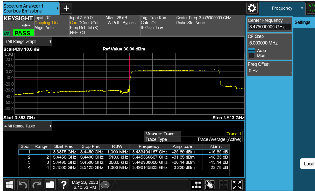
Plot 7-273. Lower ACP Plot (NR Band n77 (DoD) - 50MHz CP-OFDM-QPSK – Full RB - Ant E)
