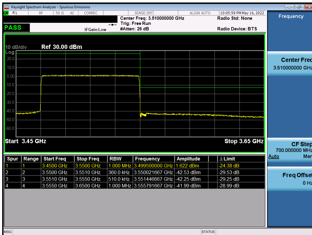
Plot 7-246. Upper ACP Plot (NR Band n77 (DoD) - 80MHz CP-OFDM-QPSK – Full RB - Ant F)
