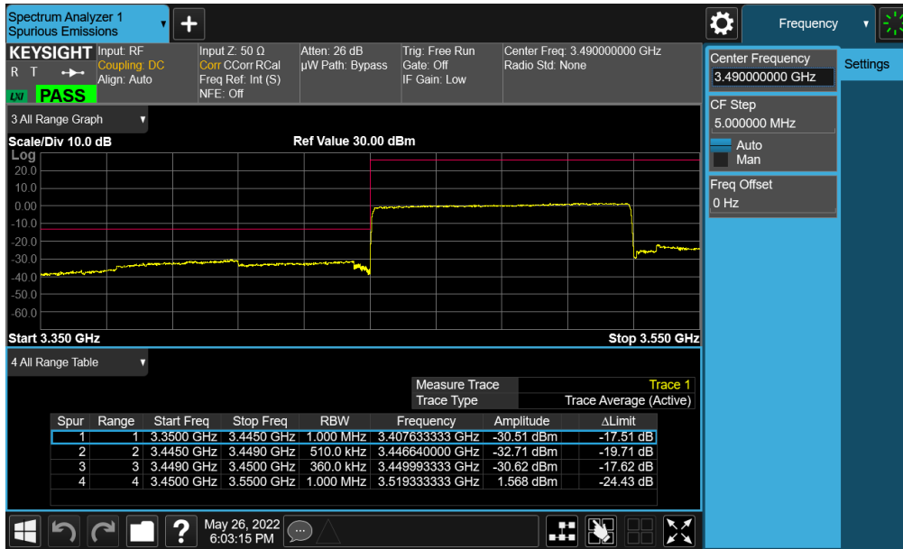
Plot 7-267. Lower ACP Plot (NR Band n77 (DoD) - 80MHz CP-OFDM-QPSK – Full RB - Ant E)
