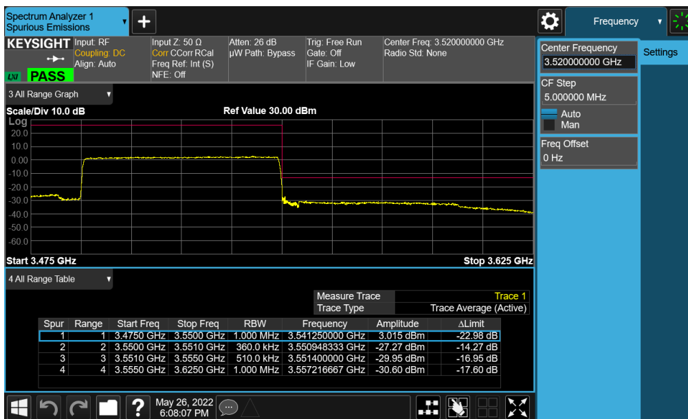
Plot 7-272. Upper ACP Plot (NR Band n77 (DoD) - 60MHz CP-OFDM-QPSK – Full RB - Ant E)
