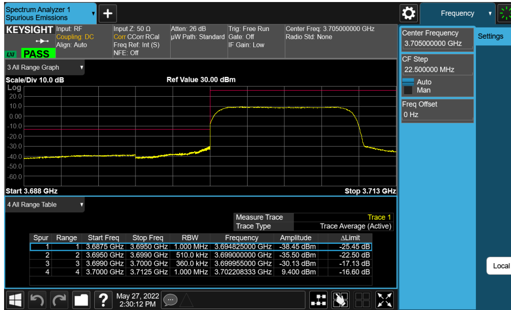
Plot 7-235. Lower ACP Plot (NR Band n77 (C-Band) - 10MHz CP-OFDM-QPSK – Full RB - Ant E)
