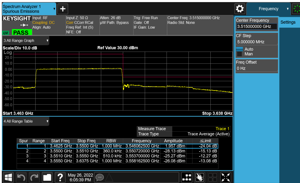
Plot 7-270. Upper ACP Plot (NR Band n77 (DoD) - 70MHz CP-OFDM-QPSK – Full RB - Ant E)
