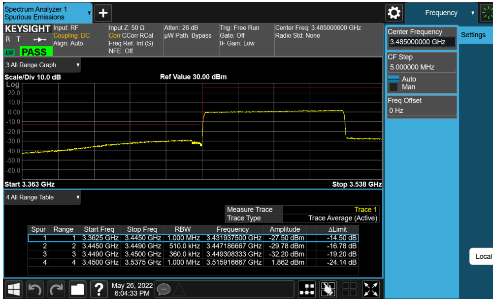
Plot 7-269. Lower ACP Plot (NR Band n77 (DoD) - 70MHz CP-OFDM-QPSK – Full RB - Ant E)
