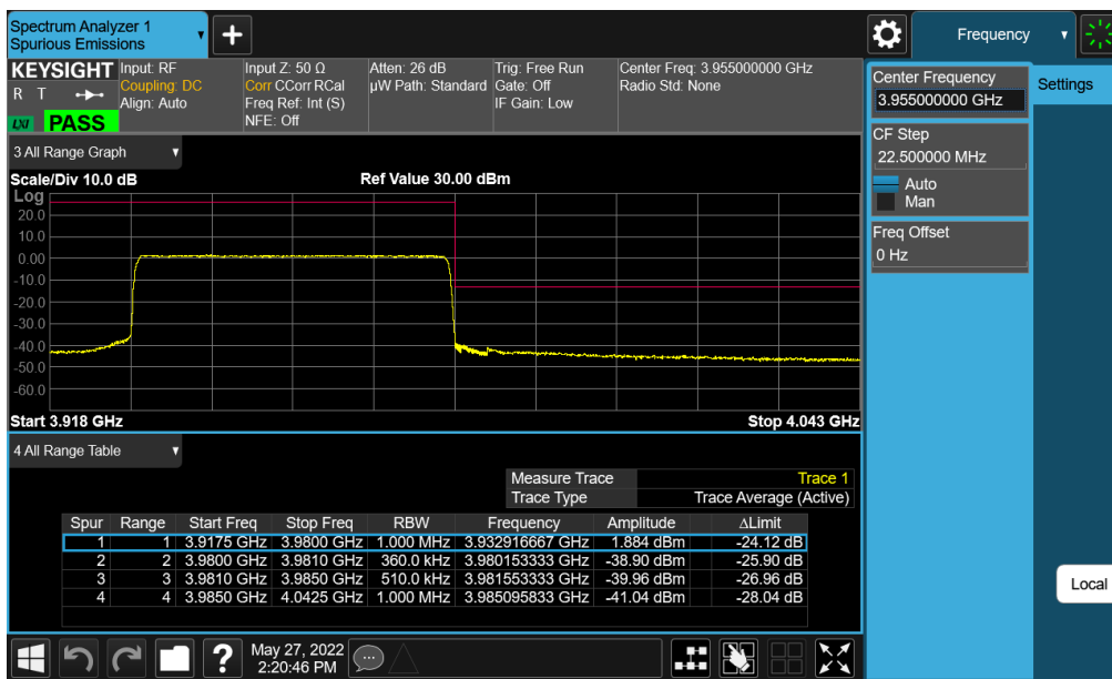
Plot 7-226. Upper ACP Plot (NR Band n77 (C-Band) - 50MHz CP-OFDM-QPSK – Full RB - Ant E)
