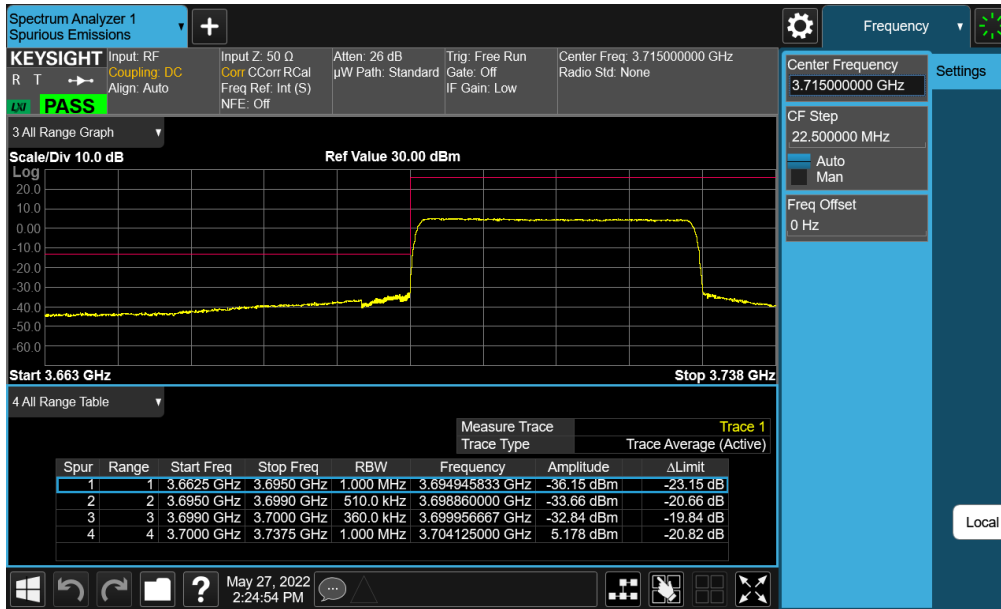
Plot 7-229. Lower ACP Plot (NR Band n77 (C-Band) - 30MHz CP-OFDM-QPSK – Full RB - Ant E)
