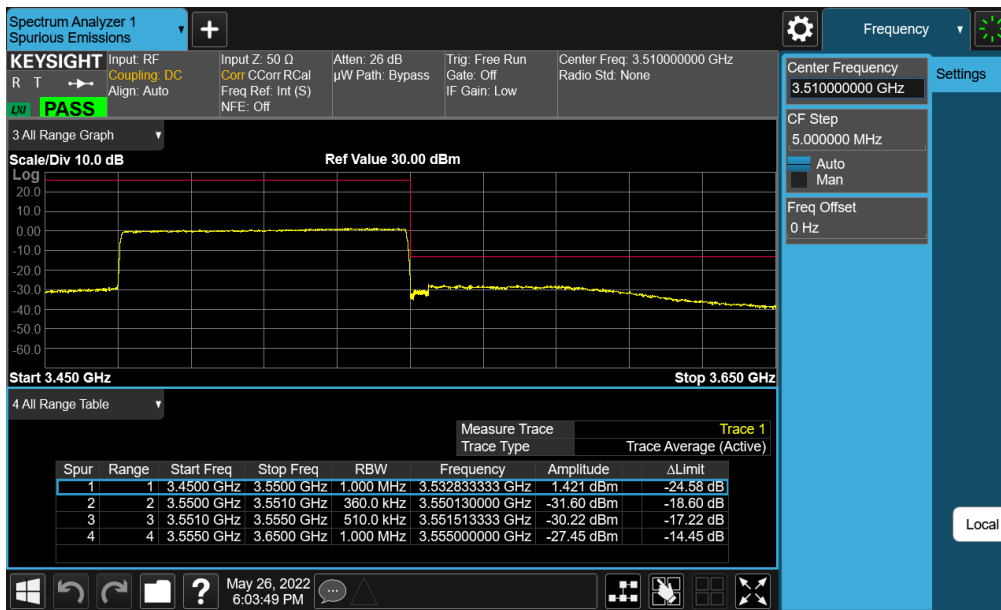
Plot 7-268. Upper ACP Plot (NR Band n77 (DoD) - 80MHz CP-OFDM-QPSK – Full RB - Ant E)
