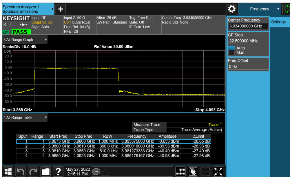
Plot 7-218. Upper ACP Plot (NR Band n77 (C-Band) - 90MHz CP-OFDM-QPSK – Full RB - Ant E)
