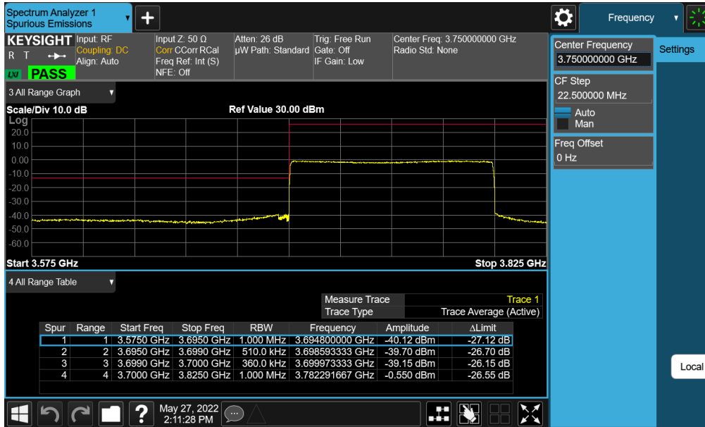
Plot 7-215. Lower ACP Plot (NR Band n77 (C-Band) - 100MHz CP-OFDM-QPSK – Full RB - Ant E)
