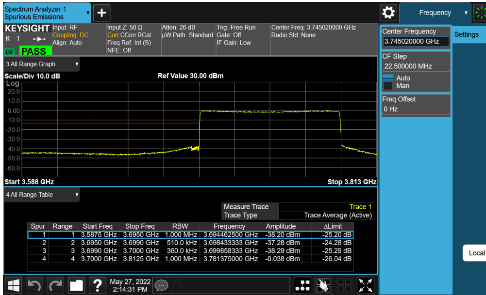
Plot 7-217. Lower ACP Plot (NR Band n77 (C-Band) - 90MHz CP-OFDM-QPSK – Full RB - Ant E)
