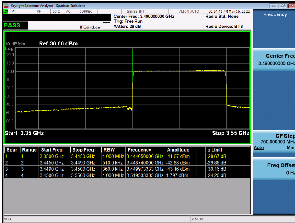
Plot 7-245. Lower ACP Plot (NR Band n77 (DoD) - 80MHz CP-OFDM-QPSK – Full RB - Ant F)
