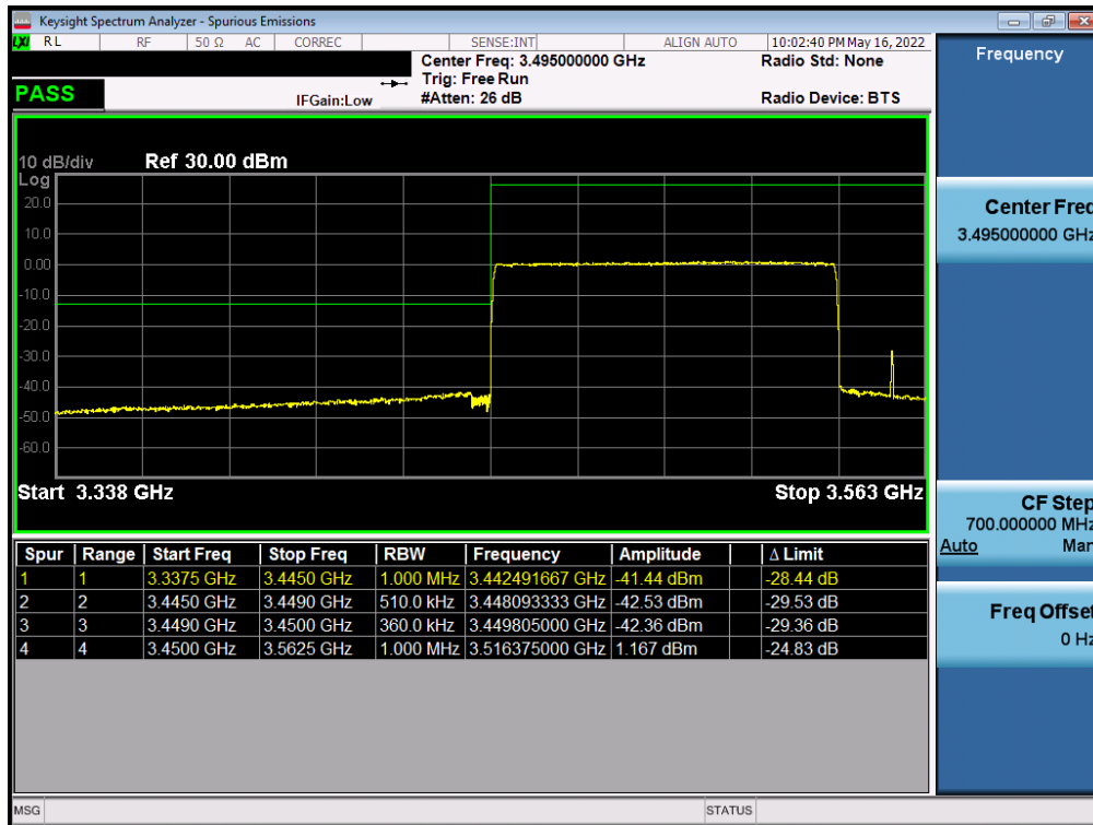
Plot 7-243. Lower ACP Plot (NR Band n77 (DoD) - 90MHz CP-OFDM-QPSK – Full RB - Ant F)
