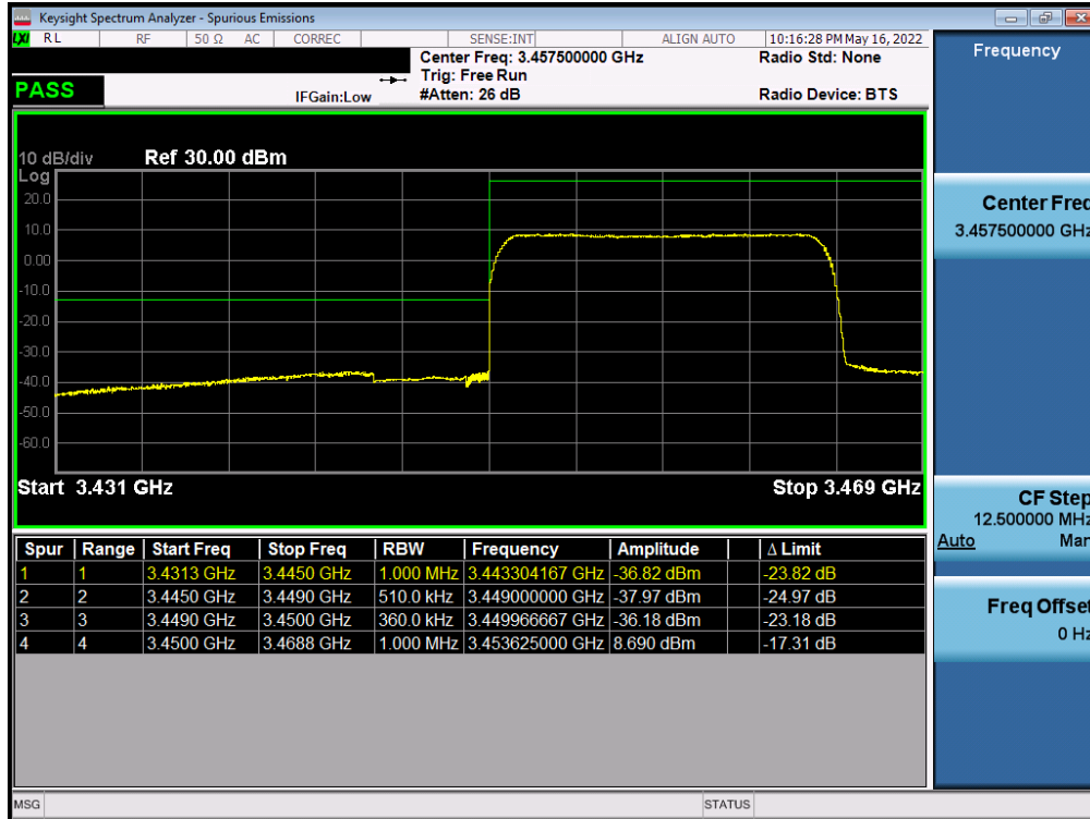
Plot 7-259. Lower ACP Plot (NR Band n77 (DoD) - 15MHz CP-OFDM-QPSK – Full RB - Ant F)
