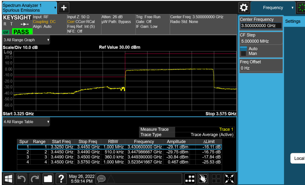
Plot 7-263. Lower ACP Plot (NR Band n77 (DoD) - 100MHz CP-OFDM-QPSK – Full RB - Ant E)
