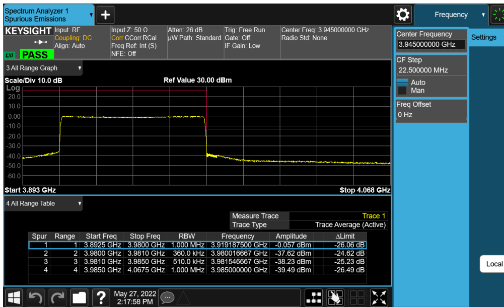
Plot 7-222. Upper ACP Plot (NR Band n77 (C-Band) - 70MHz CP-OFDM-QPSK – Full RB - Ant E)
