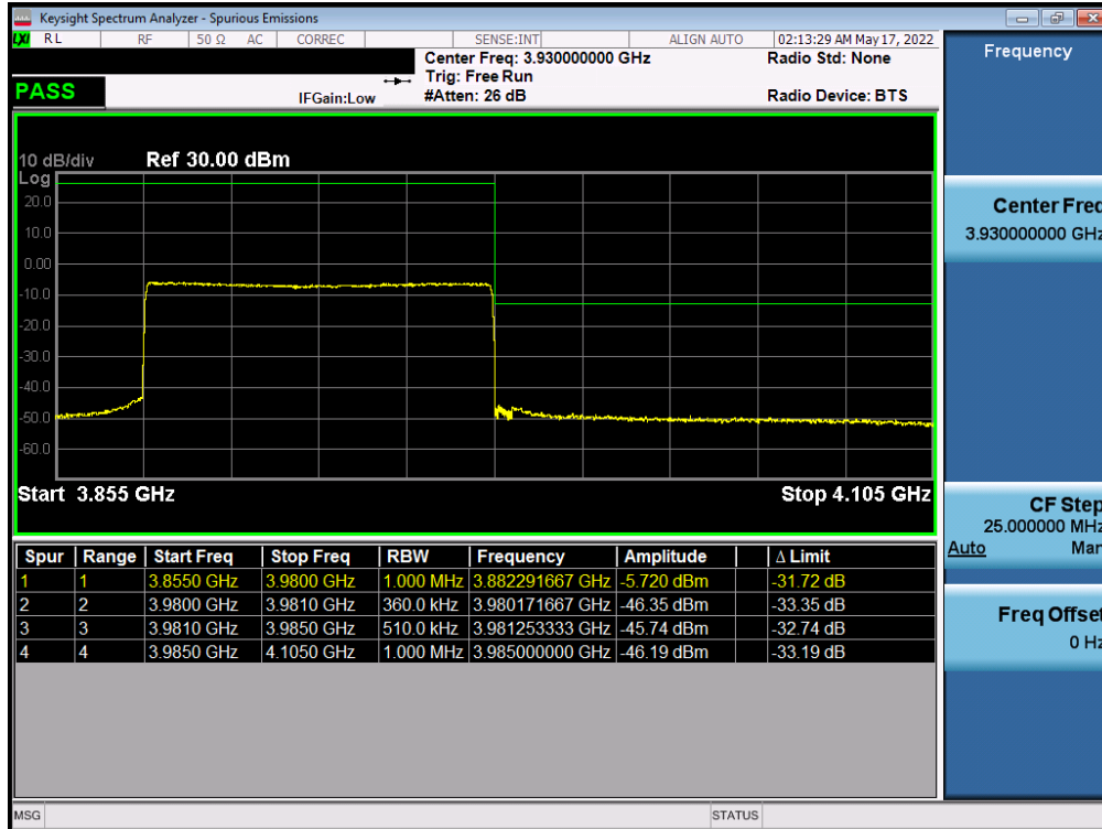
Plot 7-240. Upper ACP Plot (NR Band n77 (C-Band) - 100MHz CP-OFDM-QPSK – Full RB - Ant D)
