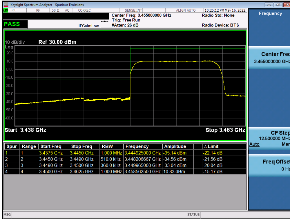
Plot 7-261. Lower ACP Plot (NR Band n77 (DoD) - 10MHz CP-OFDM-QPSK – Full RB - Ant F)
