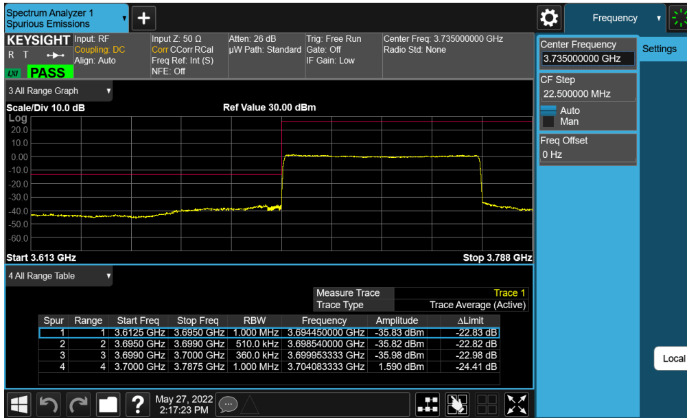
Plot 7-221. Lower ACP Plot (NR Band n77 (C-Band) - 70MHz CP-OFDM-QPSK – Full RB - Ant E)
