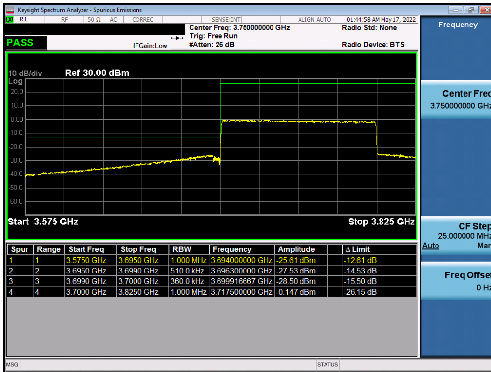
Plot 7-237. Lower ACP Plot (NR Band n77 (C-Band) - 100MHz CP-OFDM-QPSK – Full RB - Ant G)
