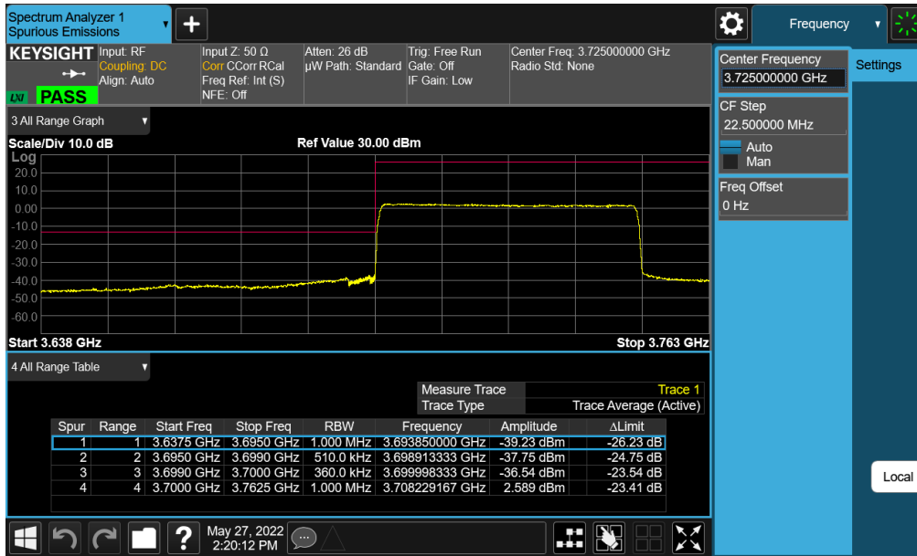
Plot 7-225. Lower ACP Plot (NR Band n77 (C-Band) - 50MHz CP-OFDM-QPSK – Full RB - Ant E)
