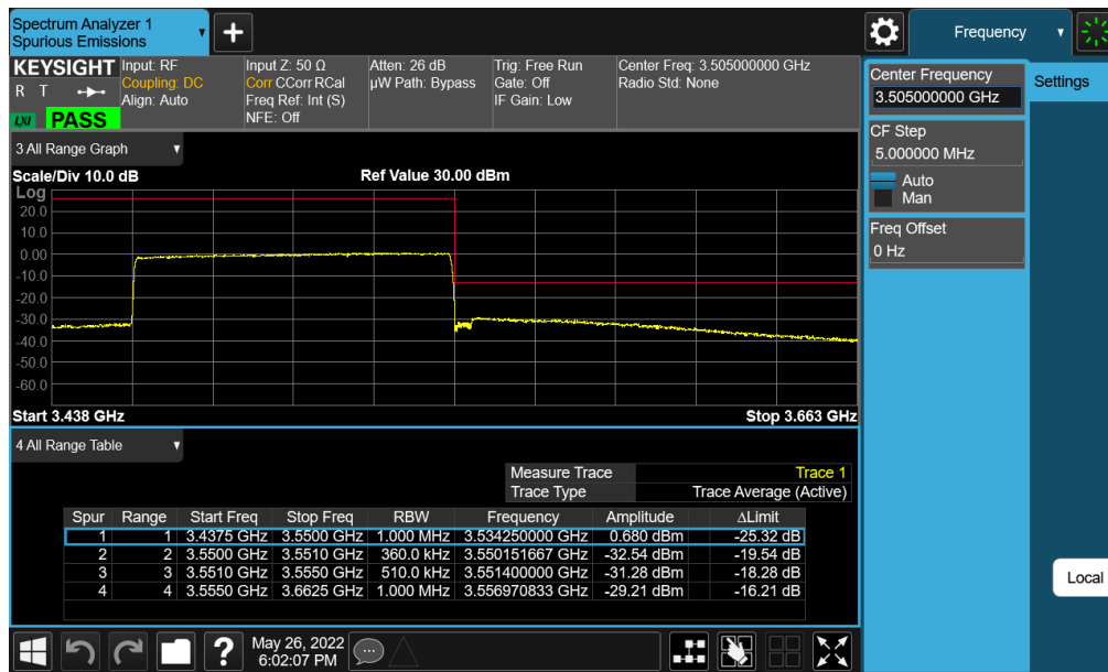
Plot 7-266. Upper ACP Plot (NR Band n77 (DoD) - 90MHz CP-OFDM-QPSK – Full RB - Ant E)
