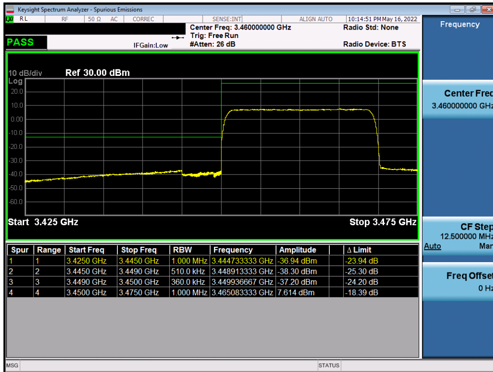
Plot 7-257. Lower ACP Plot (NR Band n77 (DoD) - 20MHz CP-OFDM-QPSK – Full RB - Ant F)
