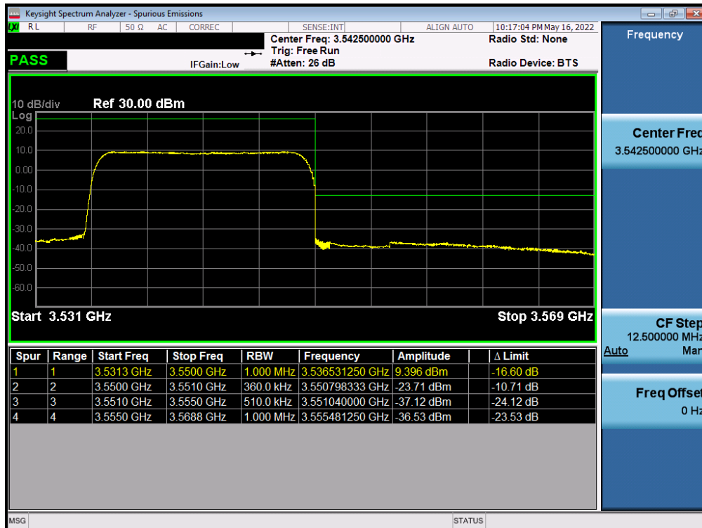
Plot 7-260. Upper ACP Plot (NR Band n77 (DoD) - 15MHz CP-OFDM-QPSK – Full RB - Ant F)
