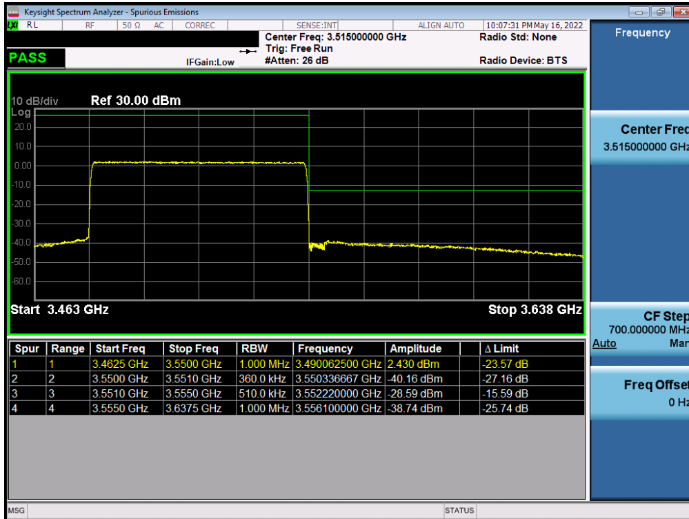
Plot 7-248. Upper ACP Plot (NR Band n77 (DoD) - 70MHz CP-OFDM-QPSK – Full RB - Ant F)
