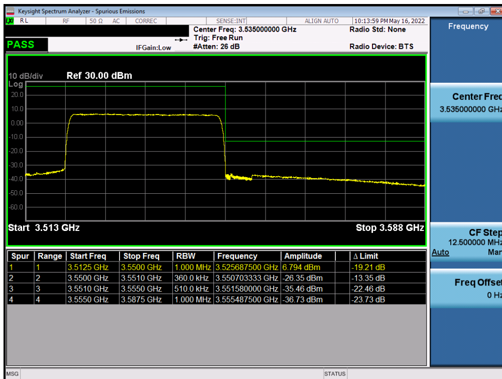
Plot 7-256. Upper ACP Plot (NR Band n77 (DoD) - 30MHz CP-OFDM-QPSK – Full RB - Ant F)
