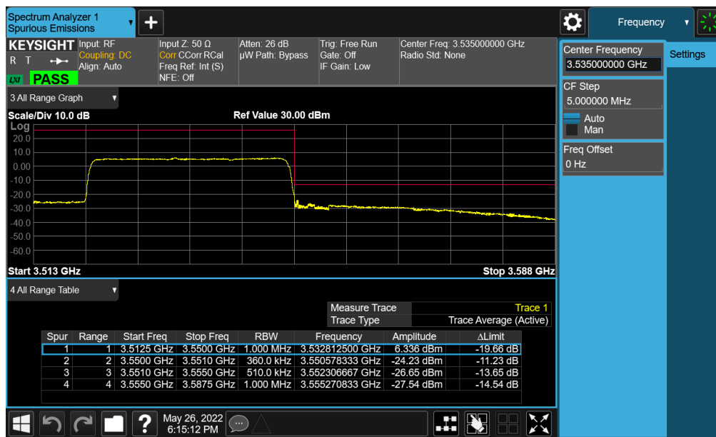
Plot 7-278. Upper ACP Plot (NR Band n77 (DoD) - 30MHz CP-OFDM-QPSK – Full RB - Ant E)
