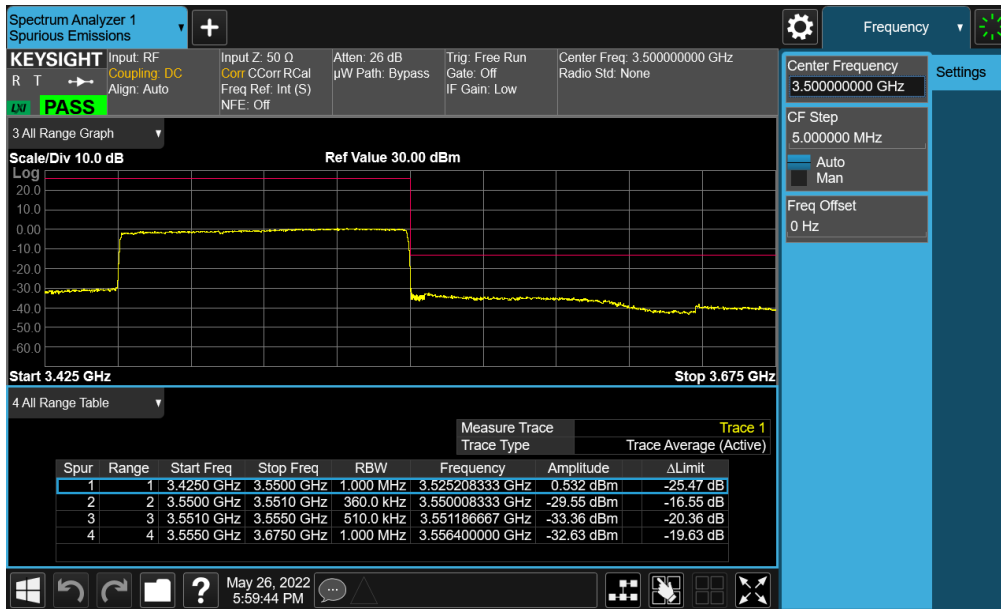
Plot 7-264. Upper ACP Plot (NR Band n77 (DoD) - 100MHz CP-OFDM-QPSK – Full RB - Ant E)
