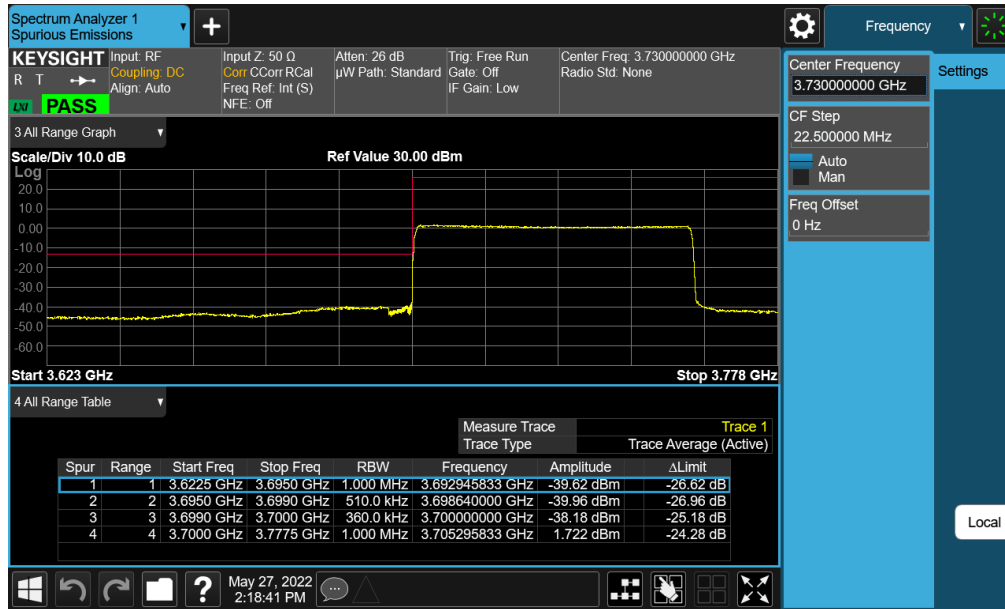
Plot 7-223. Lower ACP Plot (NR Band n77 (C-Band) - 60MHz CP-OFDM-QPSK - Full RB - Ant E)
