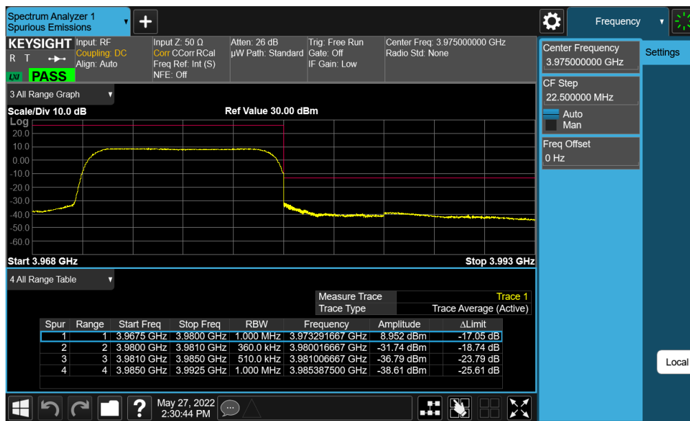
Plot 7-236. Upper ACP Plot (NR Band n77 (C-Band) - 10MHz CP-OFDM-QPSK – Full RB - Ant E)
