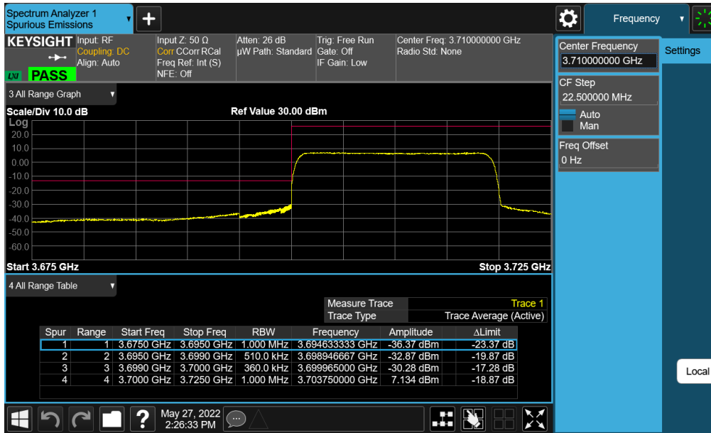
Plot 7-231. Lower ACP Plot (NR Band n77 (C-Band) - 20MHz CP-OFDM-QPSK – Full RB - Ant E)
