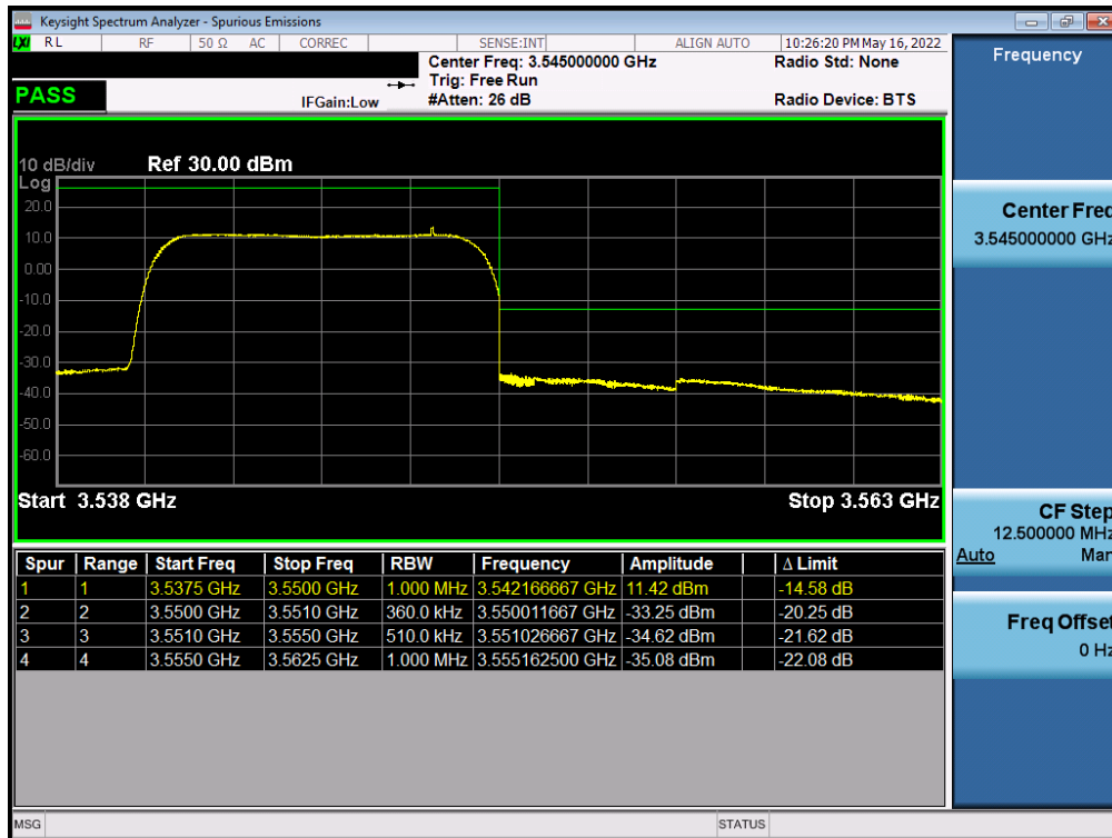
Plot 7-262. Upper ACP Plot (NR Band n77 (DoD) - 10MHz CP-OFDM-QPSK – Full RB - Ant F)
