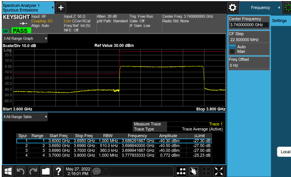
Plot 7-219. Lower ACP Plot (NR Band n77 (C-Band) - 80MHz CP-OFDM-QPSK – Full RB - Ant E)
