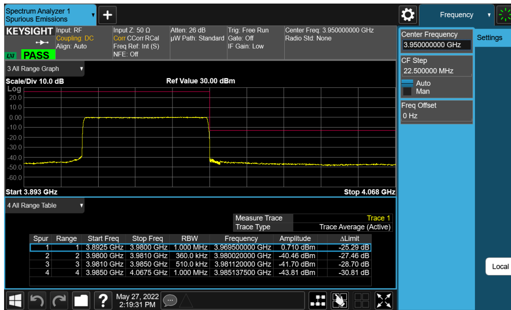
Plot 7-224. Upper ACP Plot (NR Band n77 (C-Band) - 60MHz CP-OFDM-QPSK - Full RB - Ant E)
