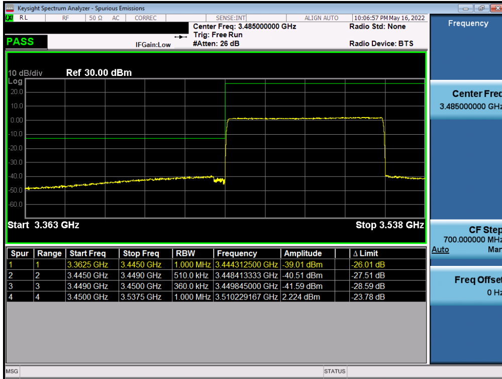
Plot 7-247. Lower ACP Plot (NR Band n77 (DoD) - 70MHz CP-OFDM-QPSK – Full RB - Ant F)
