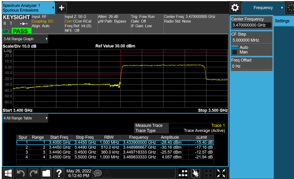
Plot 7-275. Lower ACP Plot (NR Band n77 (DoD) - 40MHz CP-OFDM-QPSK – Full RB - Ant E)
