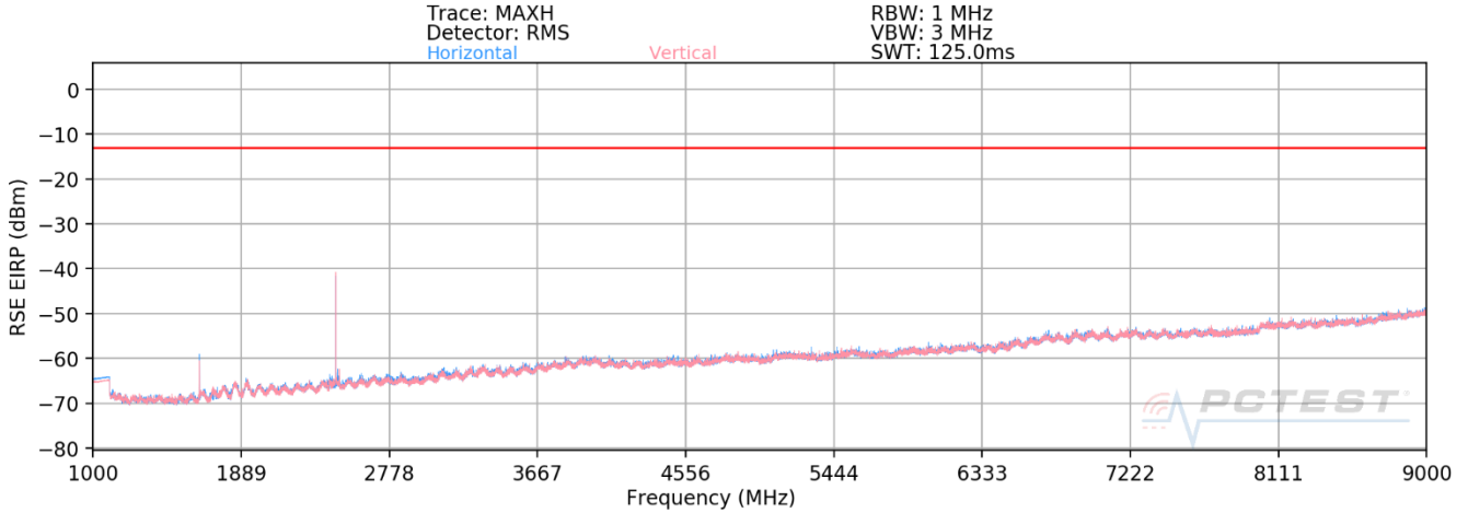
Plot 7-24. Radiated Spurious Plot Above 1GHz (LTE Band 26) – CLOSE
