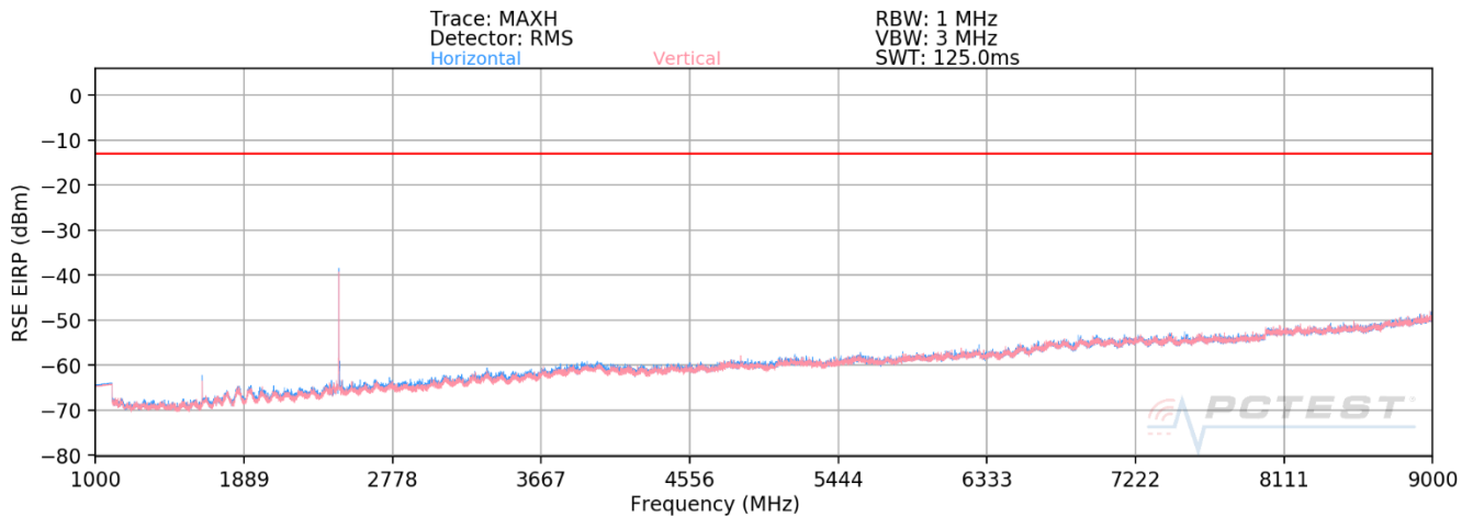
Plot 7-23. Radiated Spurious Plot Above 1GHz (LTE Band 26) – OPEN
