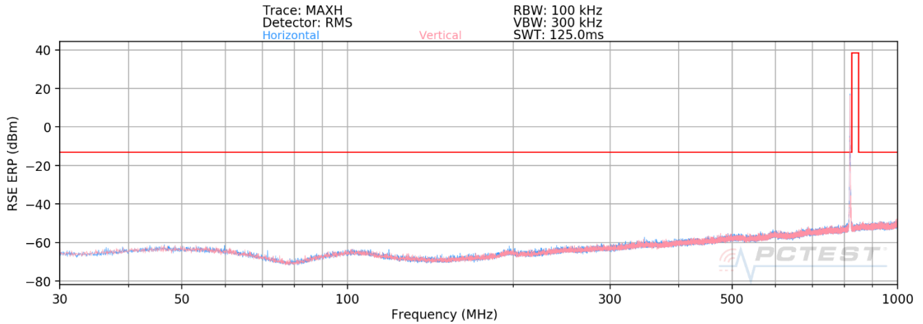
Plot 7-22. Radiated Spurious Plot Below 1GHz (LTE Band 26) – OPEN
