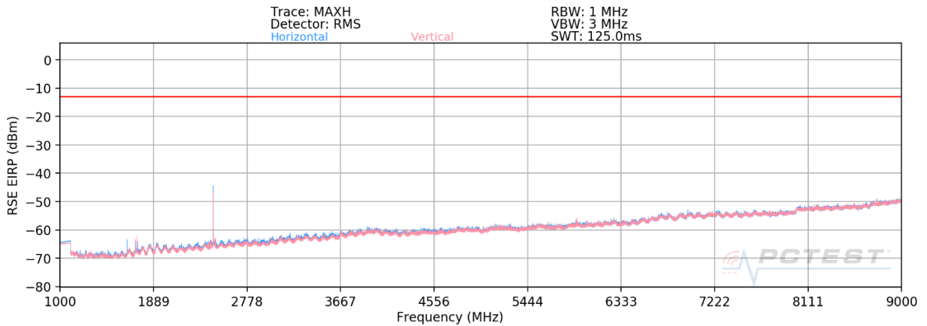
Plot 7-26. Radiated Spurious Plot Above 1GHz (LTE Band 26) – CLOSE
