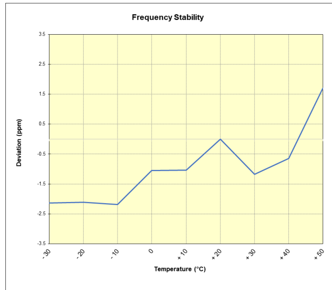
Plot 7-27. LTE Band 26 Frequency Stability Chart
