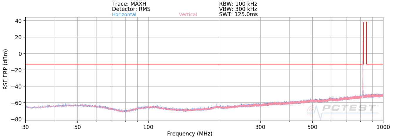
Plot 7-25. Radiated Spurious Plot Below 1GHz (LTE Band 26) – CLOSE
