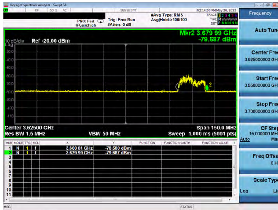
Plot 7-44. Run#2 End User Device Frequency of Operations
