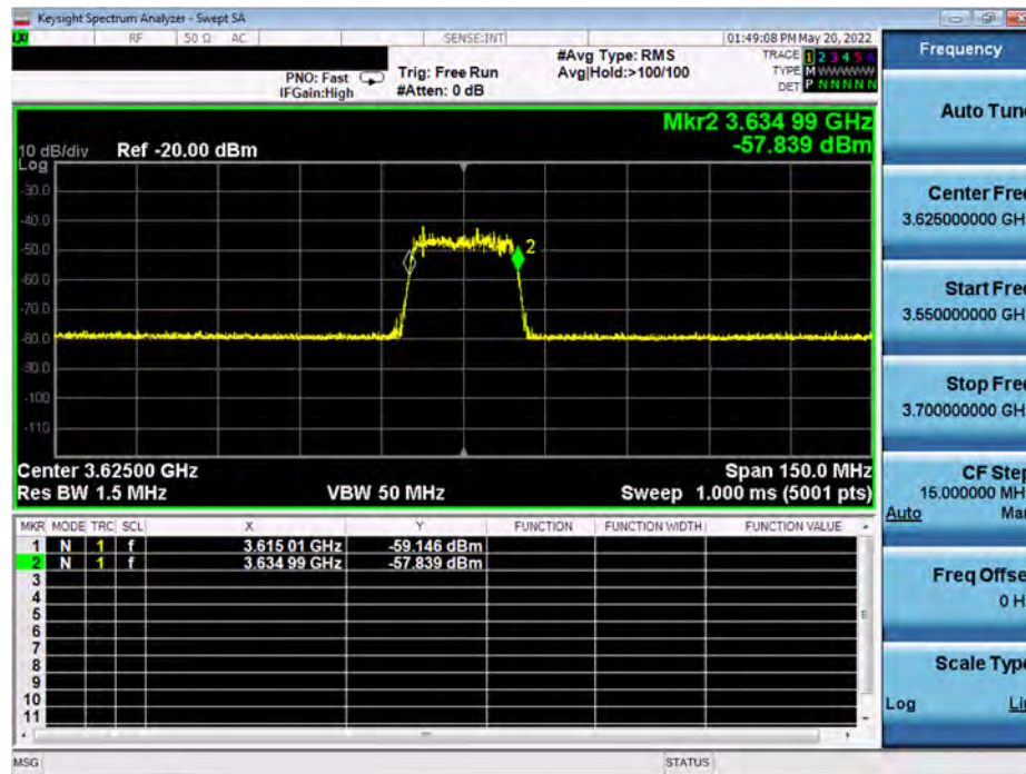
Plot 7-42. Run#1 End User Device Frequency of Operations
