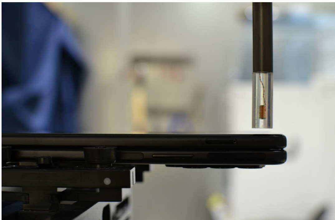
Figure 13-2 Test Setup for Wireless Device
