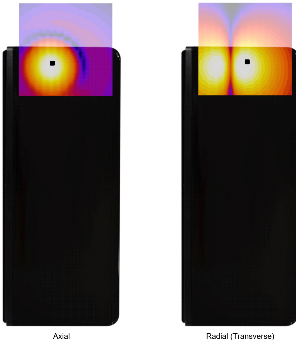
Figure 13-3 T-Coil Scan Overlay Magnetic Field Distributions
