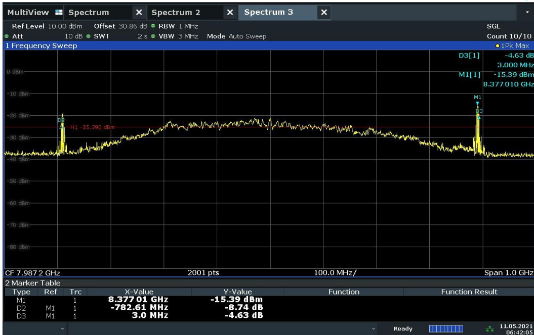
Plot 7-22. BANDWIDTH Plot – CH.9 - SP0 – Preamble 11
