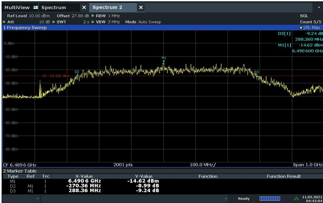
Plot 7-13. BANDWIDTH Plot – CH.5 - SP0 – Preamble 27
