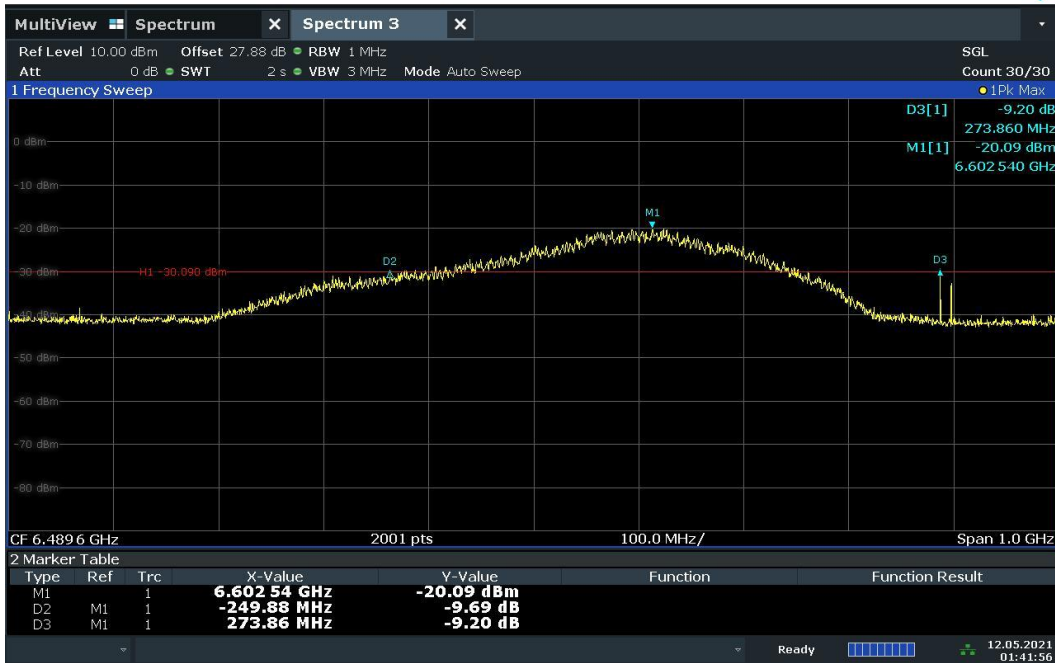
Plot 7-39. BANDWIDTH Plot – CH.5 – SP3 – Preamble 11
