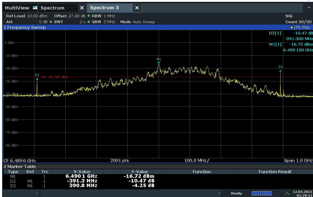
Plot 7-34. BANDWIDTH Plot – CH.5 - SP0 – Preamble 10
