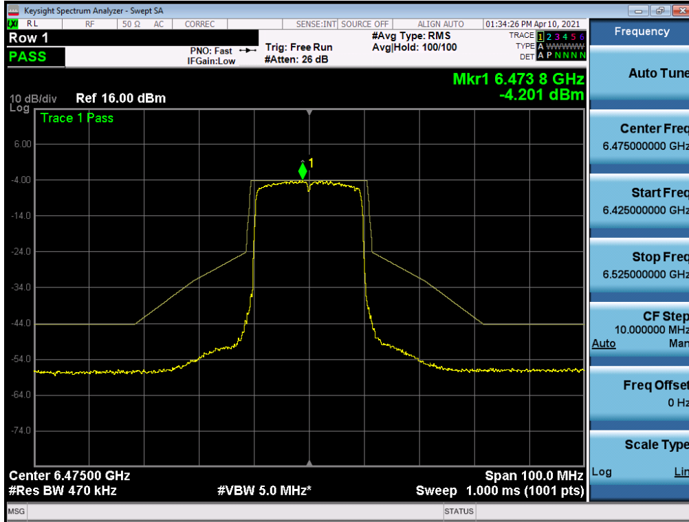
Plot 7-316. In-Band Emission Measurement Plot MIMO ANT2 (20MHz 802.11ax (UNII Band 6) – Ch. 105)
