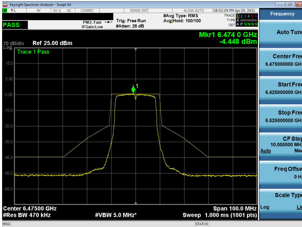
Plot 7-237. In-Band Emission Measurement Plot SISO ANT1 (20MHz 802.11a (UNII Band 6) – Ch. 105)
