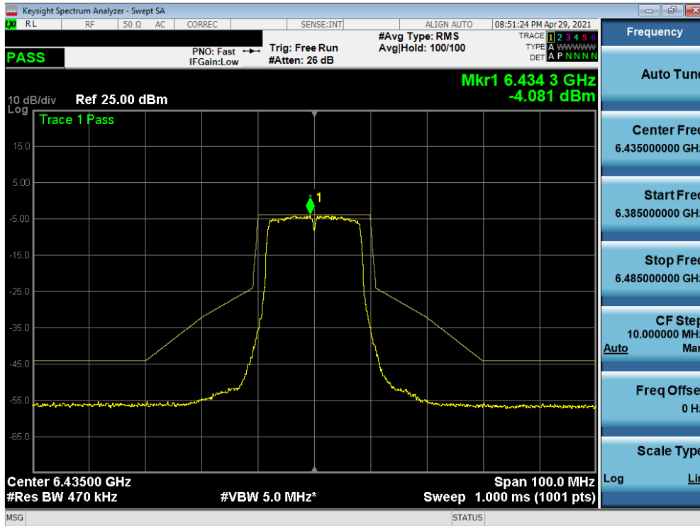
Plot 7-236. In-Band Emission Measurement Plot SISO ANT1 (20MHz 802.11a (UNII Band 6) – Ch. 97)
