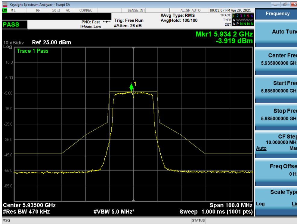
Plot 7-233. In-Band Emission Measurement Plot SISO ANT1 (20MHz 802.11a (UNII Band 5) – Ch. 2)
