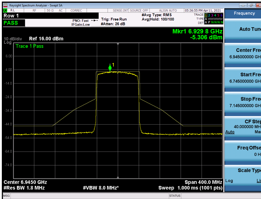
Plot 7-294. In-Band Emission Measurement Plot MIMO ANT1 (80MHz 802.11ax (UNII Band 8) – Ch. 199)
