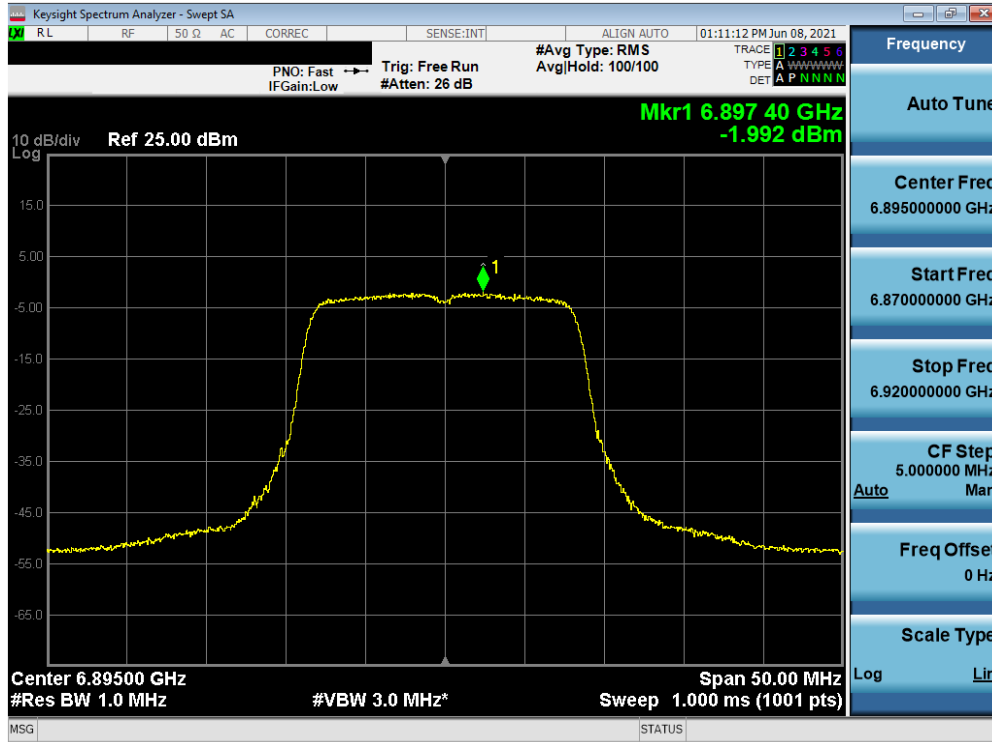
Plot 7-221. Power Spectral Density Measurement Plot MIMO ANT2 (20MHz 802.11a (UNII Band 8) – Ch. 189)
