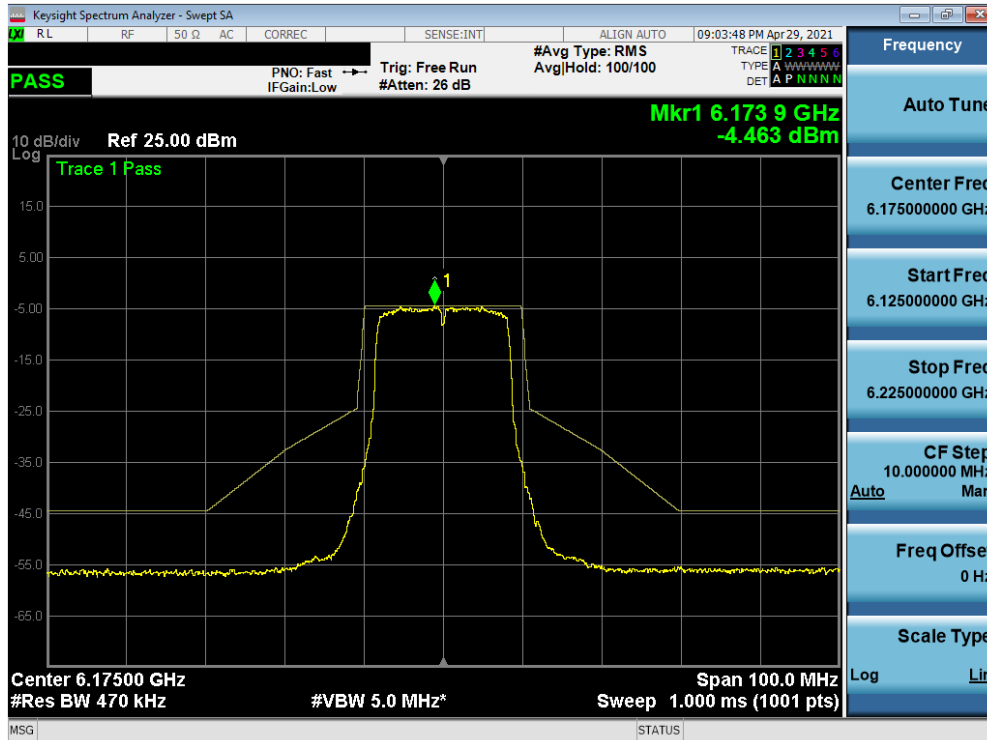
Plot 7-234. In-Band Emission Measurement Plot SISO ANT1 (20MHz 802.11a (UNII Band 5) – Ch. 45)
