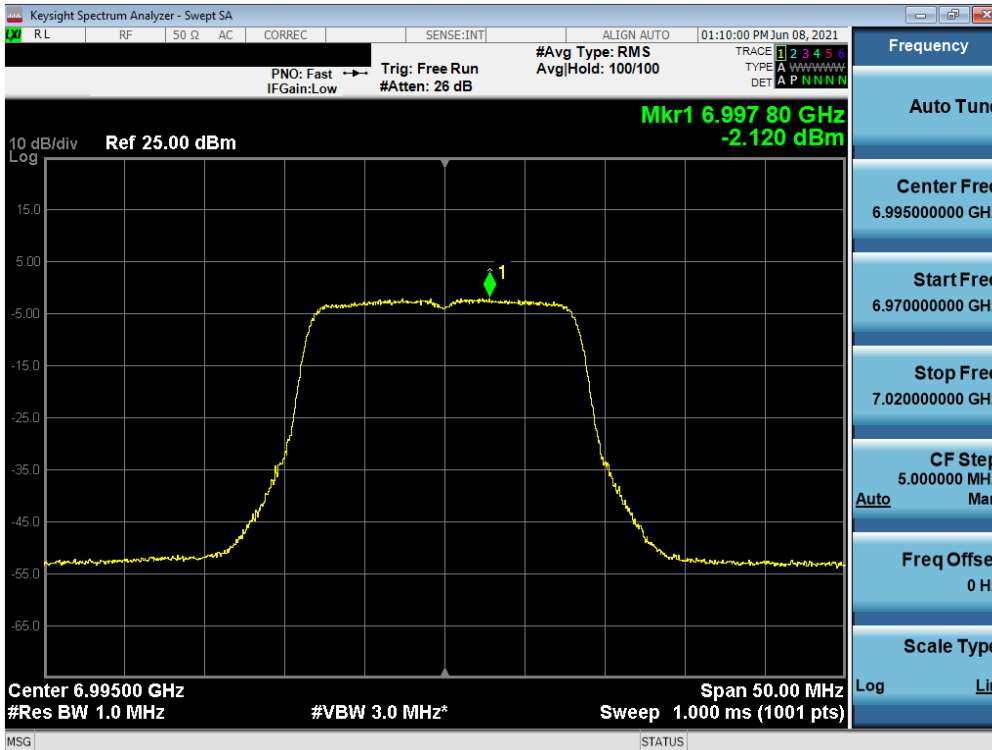
Plot 7-222. Power Spectral Density Measurement Plot MIMO ANT2 (20MHz 802.11a (UNII Band 8) – Ch. 209)
