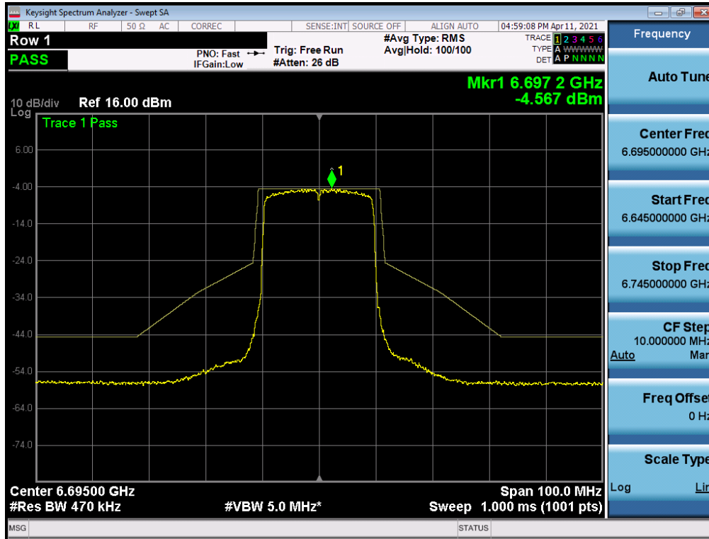
Plot 7-275. In-Band Emission Measurement Plot MIMO ANT1 (20MHz 802.11ax (UNII Band 7) – Ch. 149)
