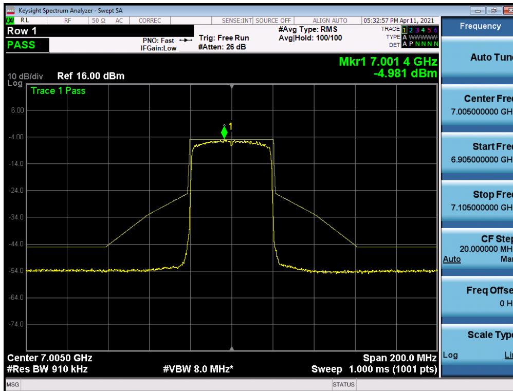
Plot 7-292. In-Band Emission Measurement Plot MIMO ANT1 (40MHz 802.11ax (UNII Band 8) – Ch. 211)
