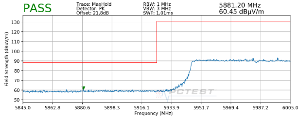
Plot 7-448. Radiated Lower Band Edge Plot MIMO (Peak – UNII Band 5)
