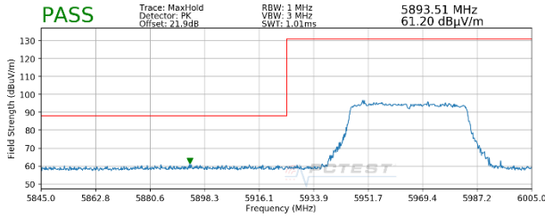
Plot 7-446. Radiated Lower Band Edge Plot MIMO (Peak – UNII Band 5)
