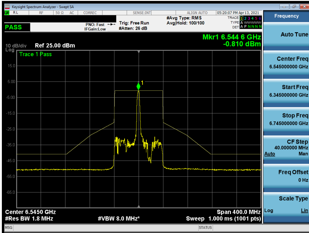
Plot 7-385. In-Band Emission Plot MIMO ANT2 (80MHz BW 802.11ax (26 Tones) (UNII Band 7) – Ch. 119)
