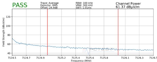
Plot 7-444. Radiated Upper Band Edge Plot MIMO (Average – UNII Band 8)
