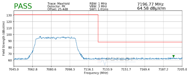
Plot 7-447. Radiated Upper Band Edge Plot MIMO (Peak – UNII Band 8)
