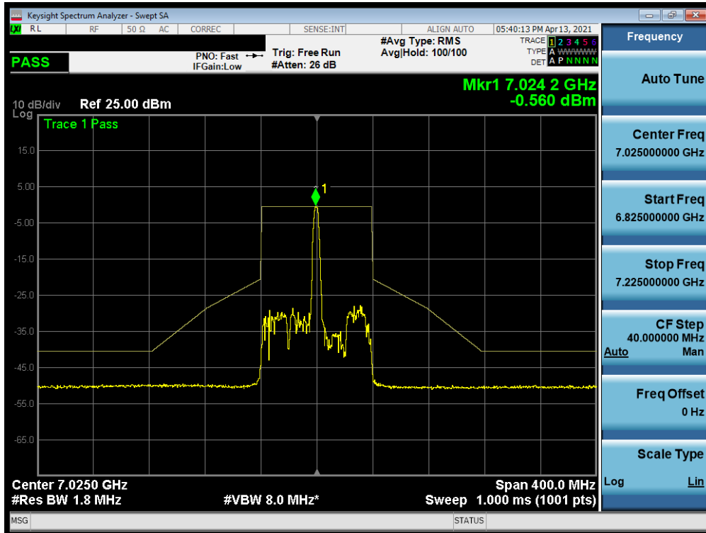
Plot 7-397. In-Band Emission Plot MIMO ANT2 (80MHz BW 802.11ax (26 Tones) (UNII Band 8) – Ch. 215)
