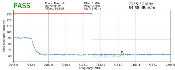
Plot 7-449. Radiated Upper Band Edge Plot MIMO (Peak – UNII Band 8)
