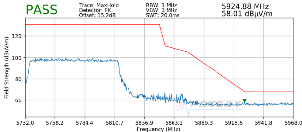
Plot 7-297. Radiated Upper Band Edge Plot MIMO (Peak – UNII Band 3 – 996 Tones)
