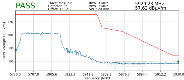
Plot 7-288. Radiated Upper Band Edge Plot MIMO (Peak – UNII Band 3 – 484 Tones)
