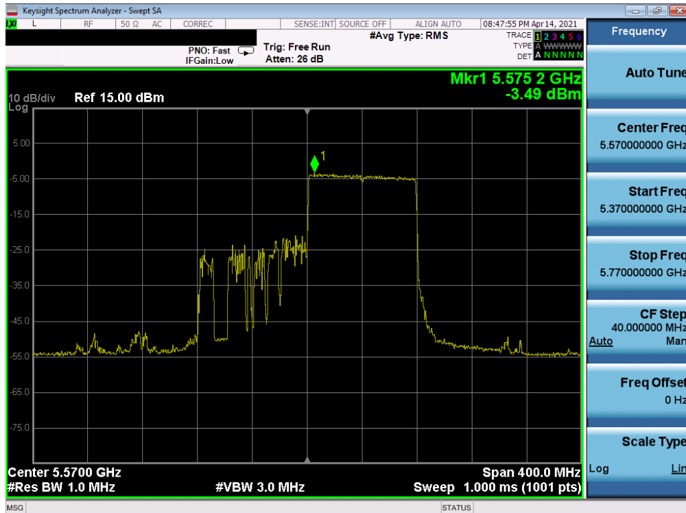
Plot 7-242. Power Spectral Density Plot MIMO ANT2 (160MHz BW(U) 802.11ax – Full Tones (UNII Band 2C) – Ch. 114)
