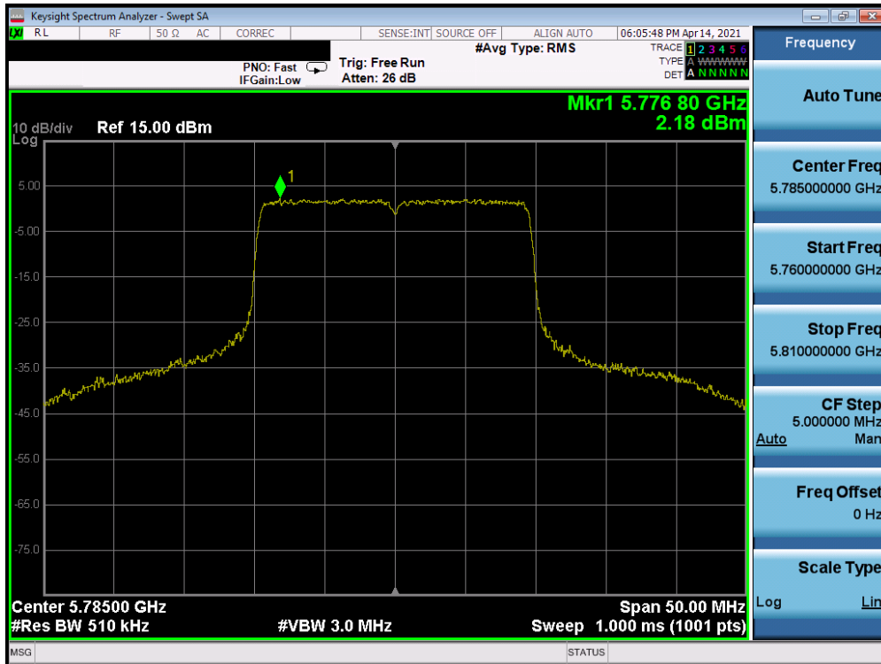
Plot 7-244. Power Spectral Density Plot MIMO ANT2 (20MHz BW 802.11ax – Full Tones (UNII Band 3) – Ch. 157)
