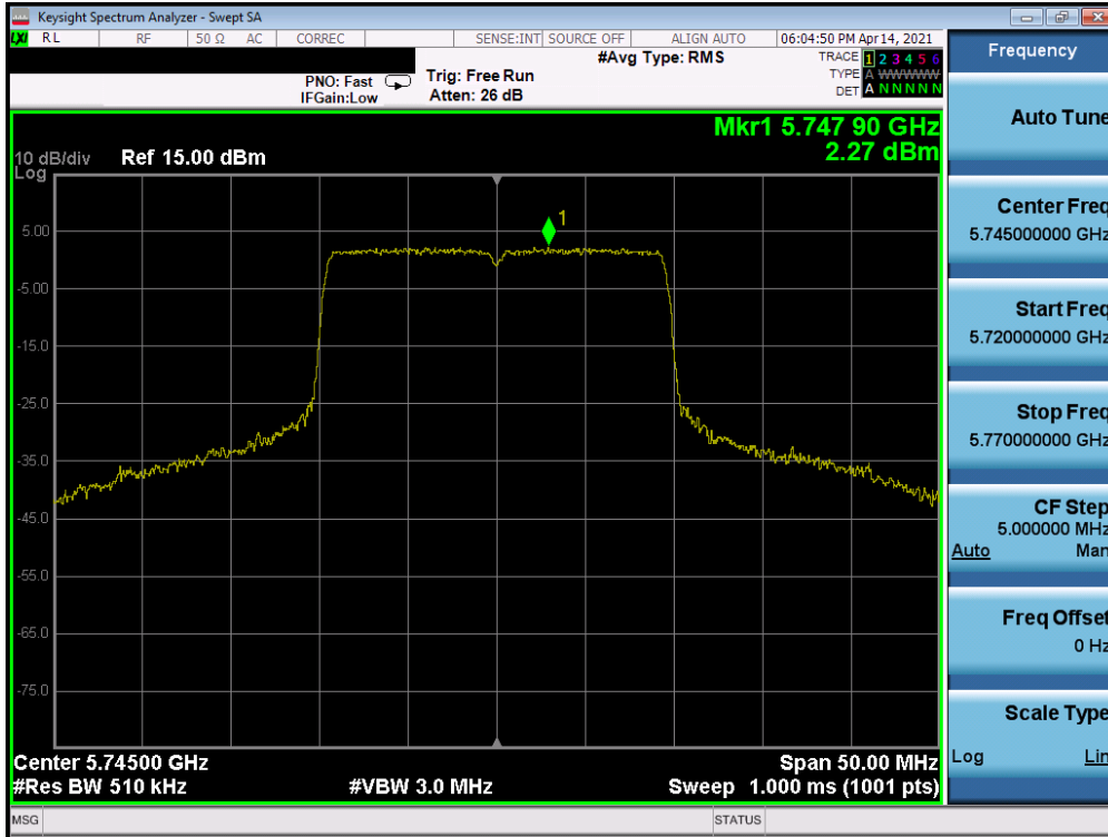
Plot 7-243. Power Spectral Density Plot MIMO ANT2 (20MHz BW 802.11ax – Full Tones (UNII Band 3) – Ch. 149)
