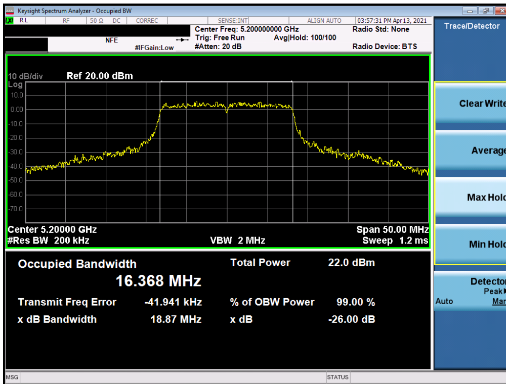
Plot 7-57. 26dB Bandwidth Plot MIMO ANT1 (802.11a (UNII Band 1) – Ch. 40)
