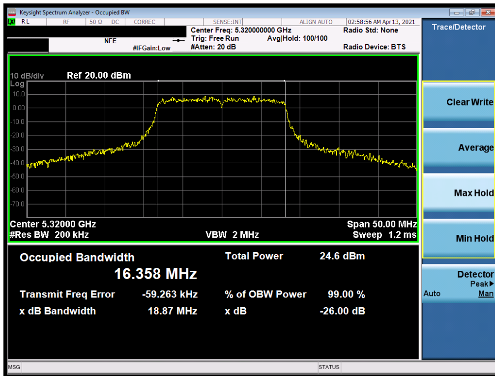
Plot 7-20. 26dB Bandwidth Plot SISO ANT1 (802.11a (UNII Band 2A) – Ch. 64)
