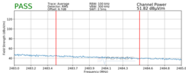
Plot 7-87. Radiated Restricted Upper Band Edge Measurement MIMO (Average – 106 Tones)
