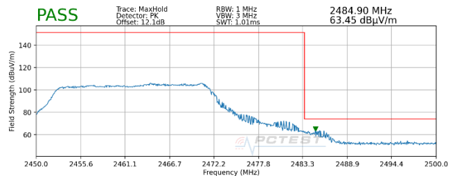
Plot 7-100. Radiated Restricted Band Edge Measurement MIMO with WCP (Peak)
