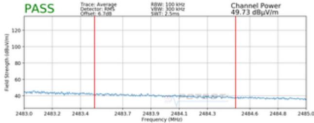
Plot 7-97. Radiated Restricted Upper Band Edge Measurement MIMO (Average – 242 Tones)
