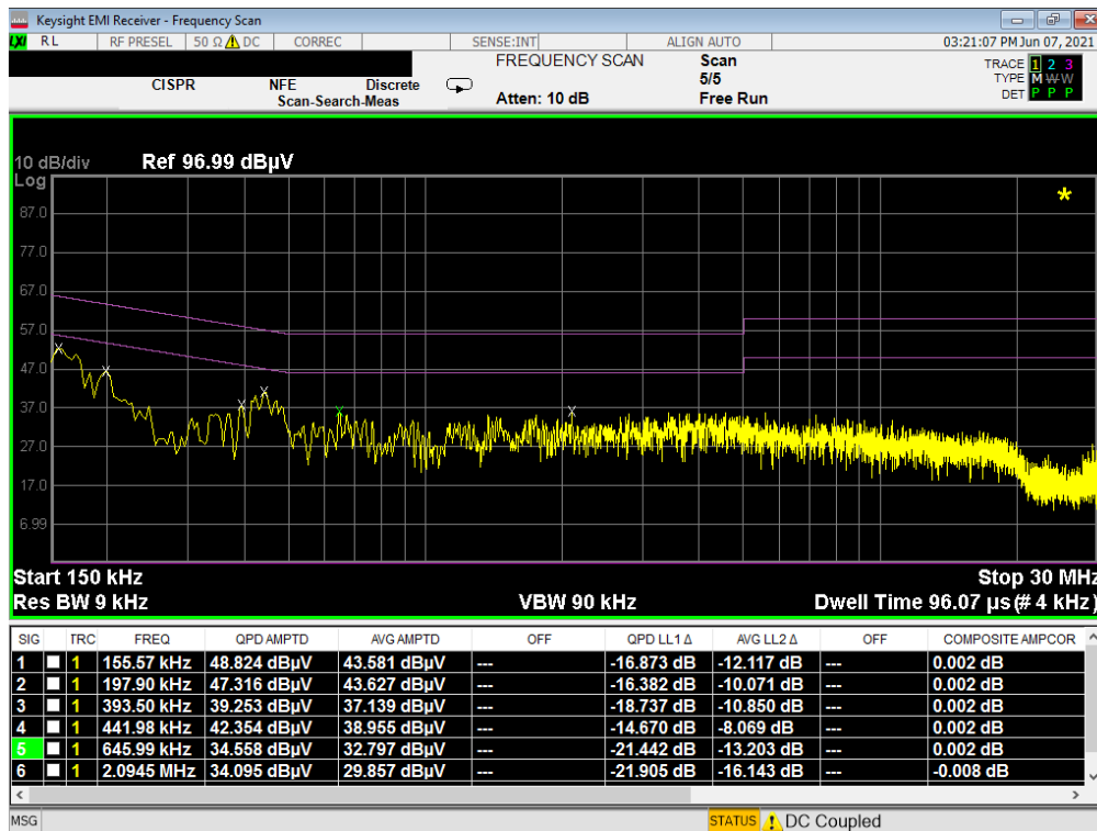
Plot 7-61. Line Conducted Plot with Bluetooth LE (N) with WCP
