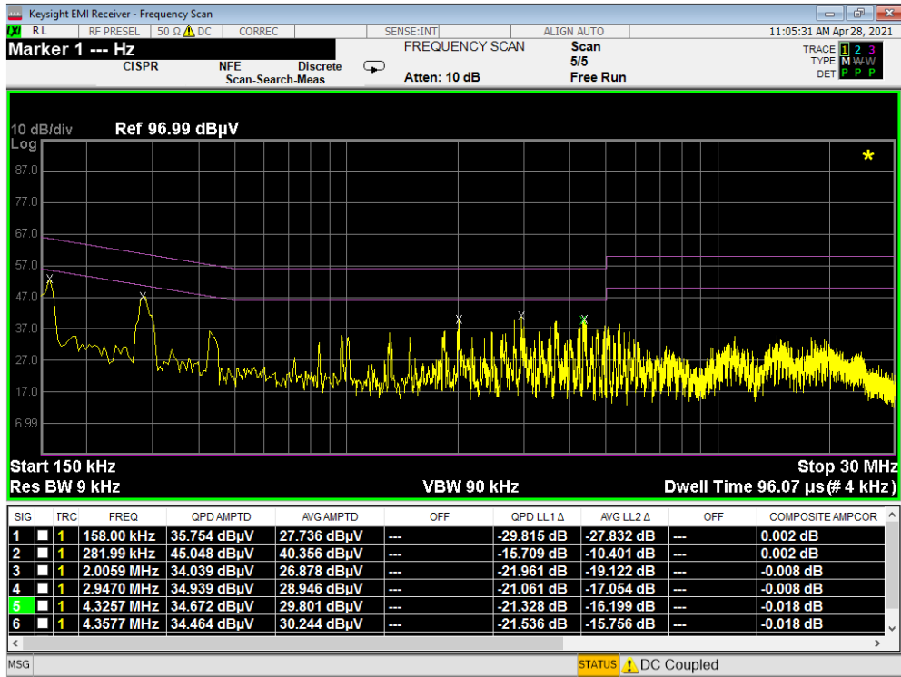
Plot 7-58. Line Conducted Plot with Bluetooth LE (L1) OPEN
