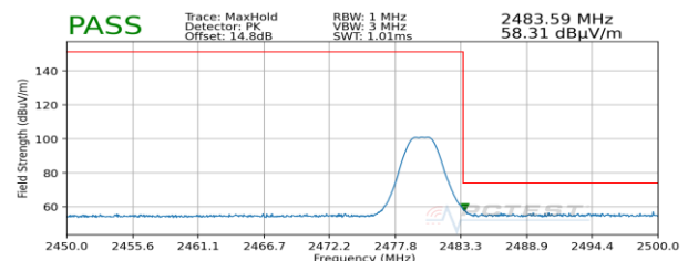
Plot 7-54. Radiated Restricted Upper Band Edge Measurement (Peak) - CLOSED
