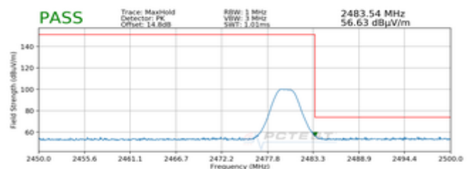
Plot 7-56. Radiated Restricted Upper Band Edge Measurement (Peak) - WCP
