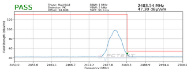
Plot 7-55. Radiated Restricted Upper Band Edge Measurement (Average) - WCP
