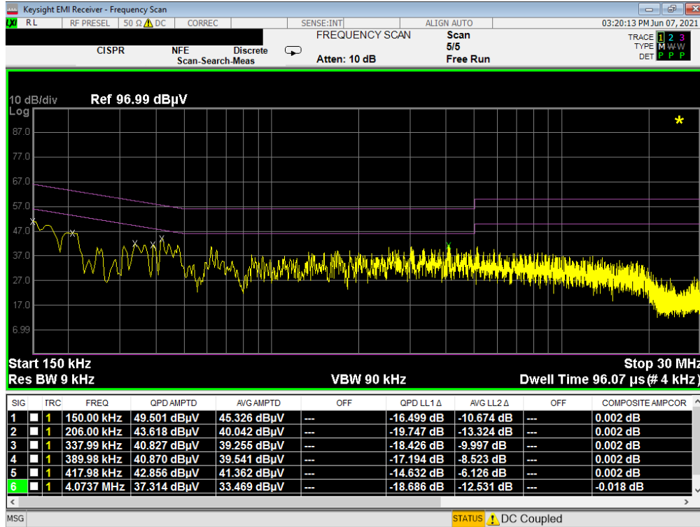
Plot 7-60. Line Conducted Plot with Bluetooth LE (L1) with WCP
