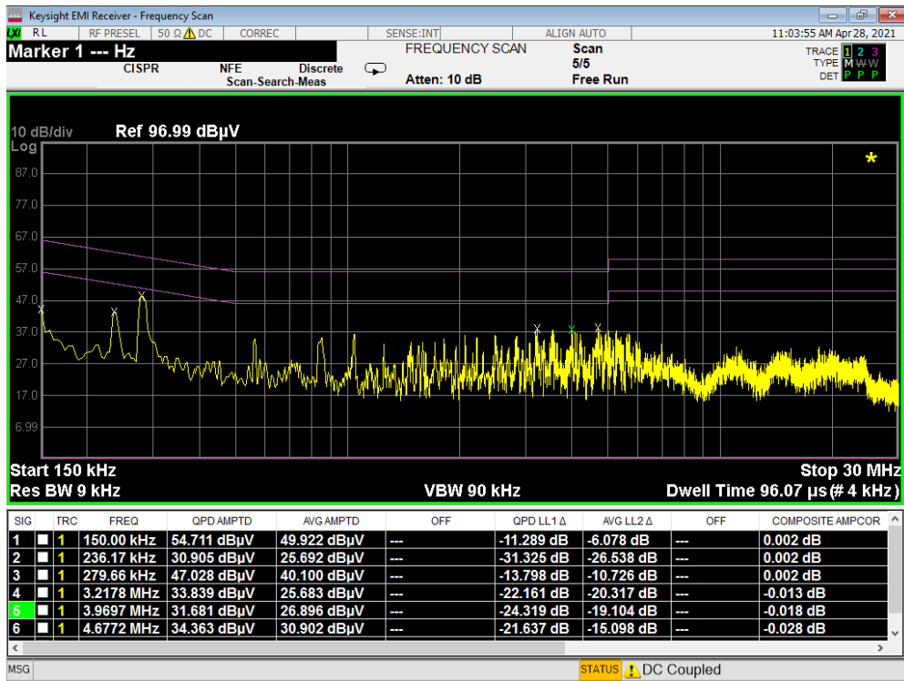
Plot 7-59. Line Conducted Plot with Bluetooth LE (N) OPEN
