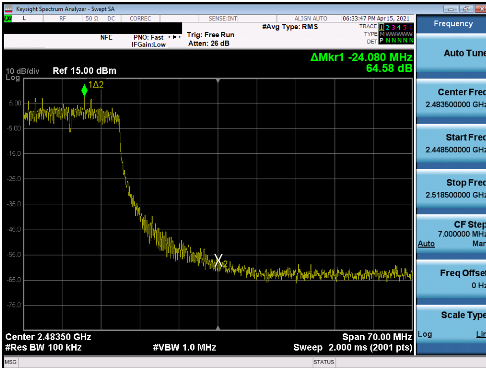
Plot 7-100. Band Edge Plot MIMO ANT1 (802.11n (2.4GHz) – Ch. 10)
