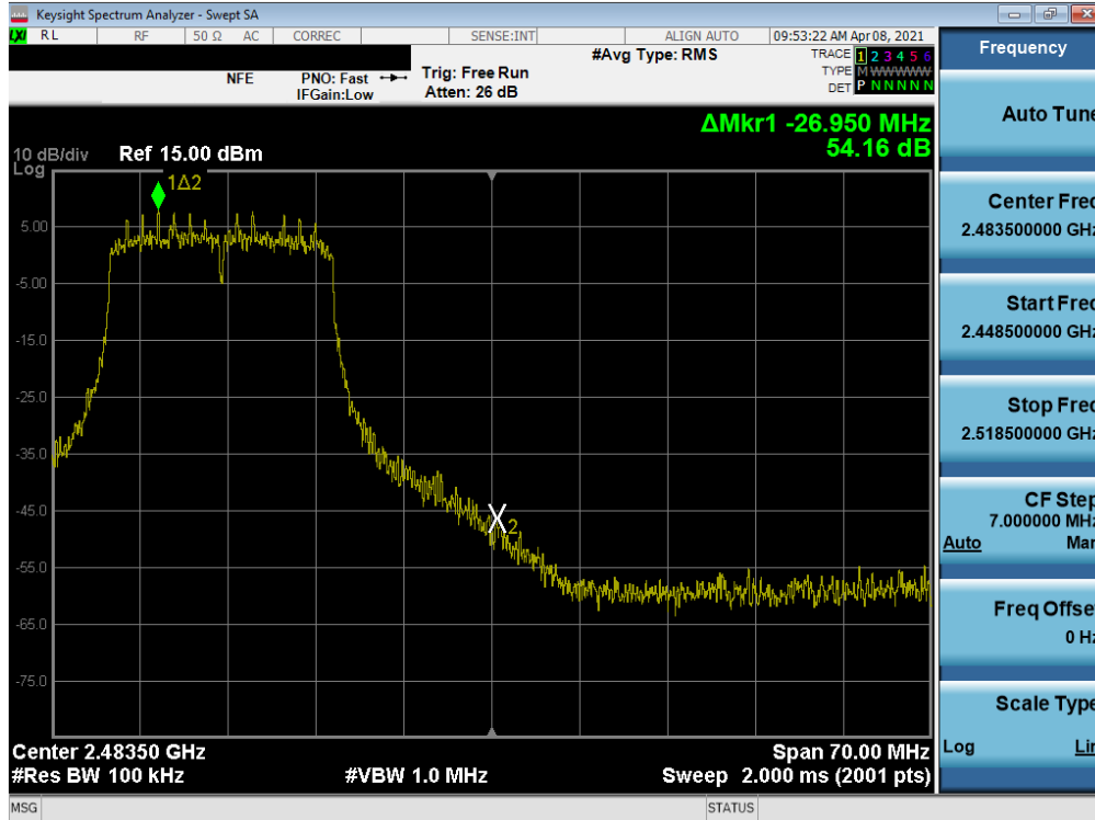
Plot 7-101. Band Edge Plot MIMO ANT1 (802.11n (2.4GHz) – Ch. 11)
