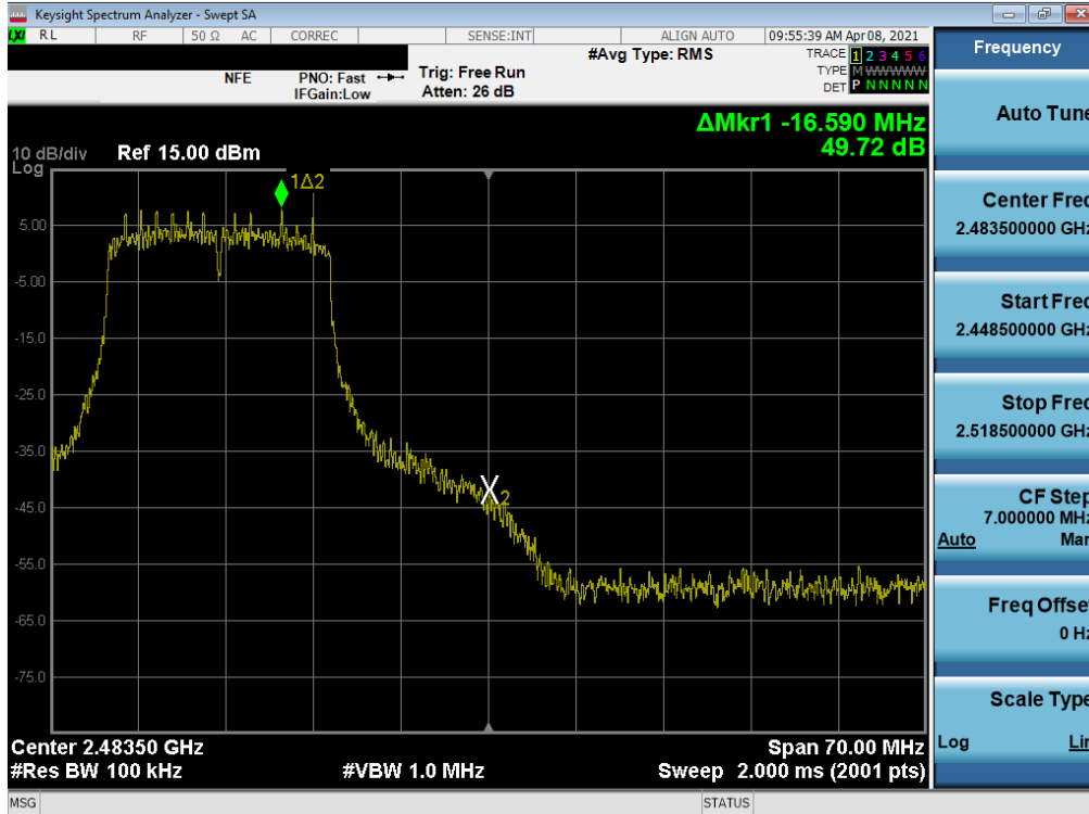
Plot 7-119. Band Edge Plot MIMO ANT2 (802.11n (2.4GHz) – Ch. 11)
