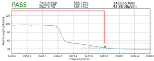
Plot 7-163. Radiated Restricted Upper Band Edge Measurement SISO ANT2 (Average) – OPEN
