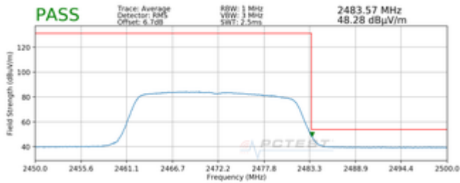
Plot 7-179. Radiated Restricted Upper Band Edge Measurement MIMO (Average) – OPEN
