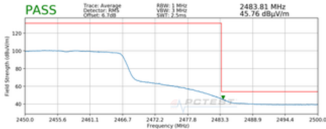
Plot 7-173. Radiated Restricted Upper Band Edge Measurement MIMO (Average) – OPEN
