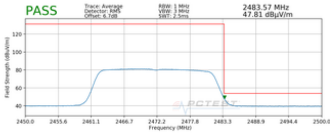
Plot 7-169. Radiated Restricted Upper Band Edge Measurement SISO ANT2 (Average) – OPEN
