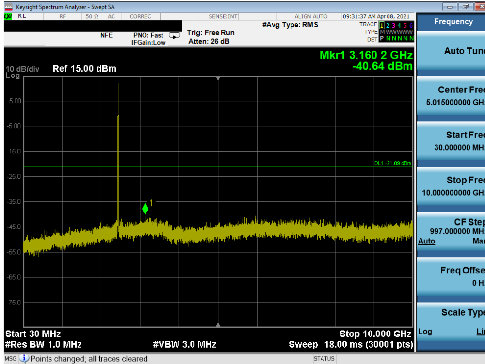
Plot 7-143. Conducted Spurious Plot MIMO ANT2 (802.11b – Ch. 11)
