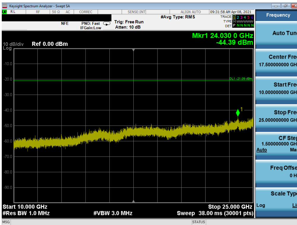
Plot 7-144. Conducted Spurious Plot MIMO ANT2 (802.11b – Ch. 11)
