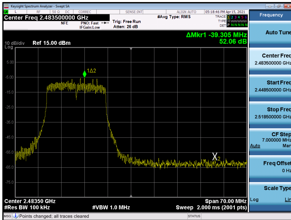
Plot 7-120. Band Edge Plot MIMO ANT2 (802.11n (2.4GHz) – Ch. 12)
