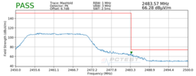
Plot 7-182. Radiated Restricted Band Edge Measurement MIMO with WCP (Peak) – OPEN
