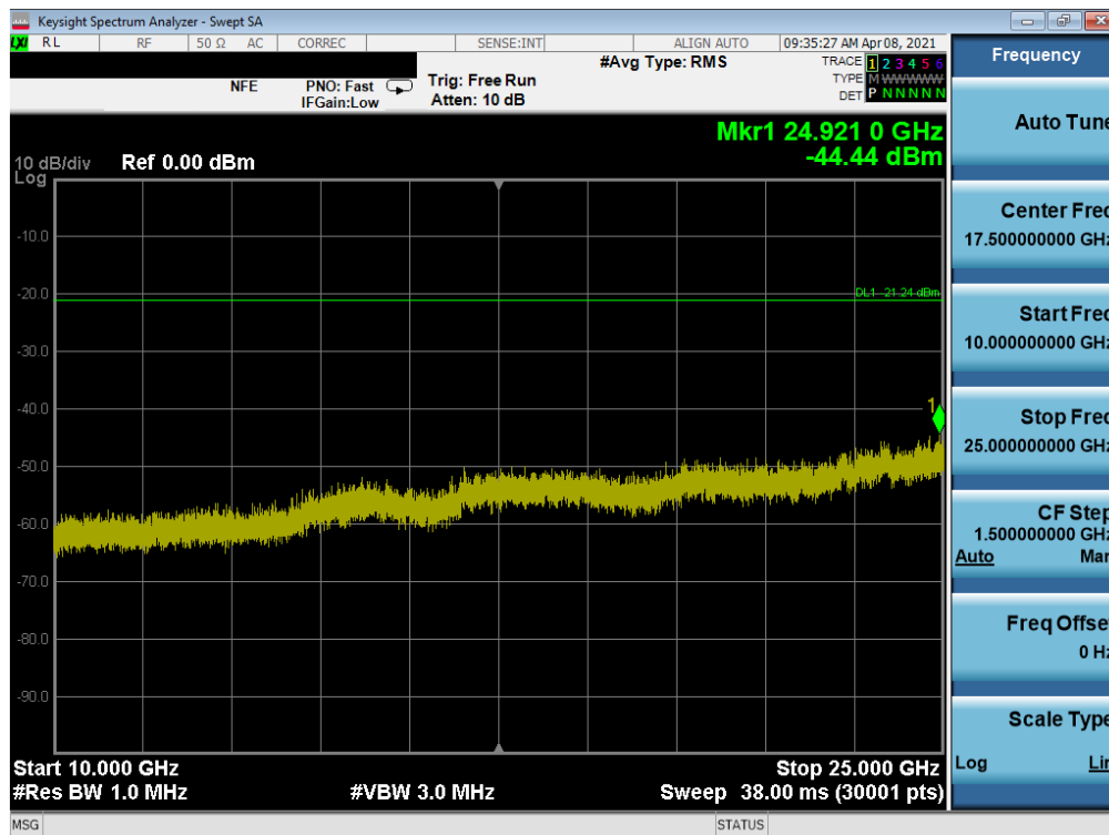
Plot 7-142. Conducted Spurious Plot MIMO ANT2 (802.11b – Ch. 6)
