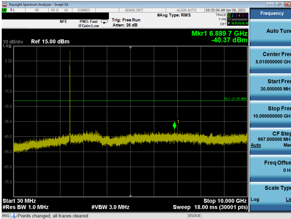
Plot 7-141. Conducted Spurious Plot MIMO ANT2 (802.11b – Ch. 6)
