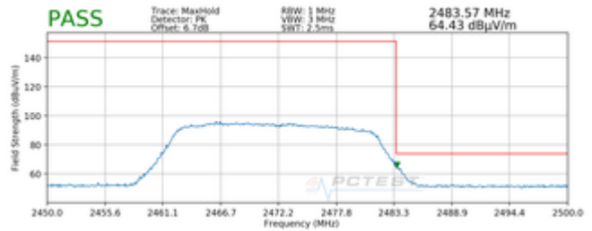
Plot 7-180. Radiated Restricted Upper Band Edge Measurement MIMO (Peak) – OPEN
