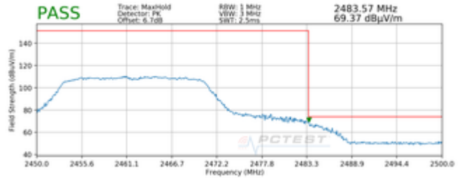
Plot 7-176. Radiated Restricted Upper Band Edge Measurement MIMO (Peak) – OPEN
