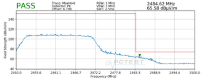
Plot 7-166. Radiated Restricted Upper Band Edge Measurement SISO ANT2 (Peak) – OPEN
