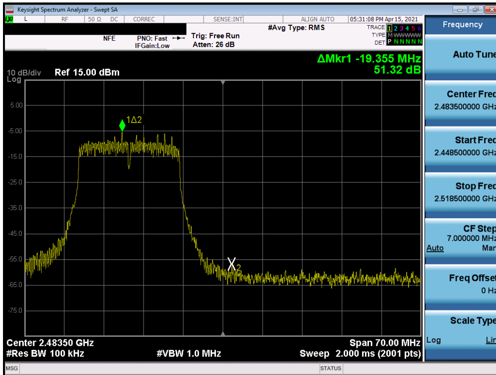
Plot 7-102. Band Edge Plot MIMO ANT1 (802.11n (2.4GHz) – Ch. 12)
