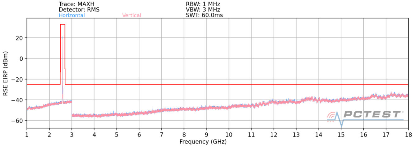
Plot 7-41. Radiated Spurious Plot (LTE Band 41(PC3))- CLOSED
