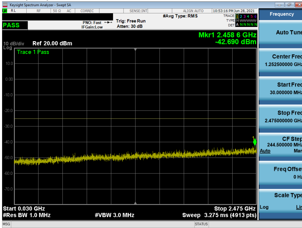
Plot 7-19. Conducted Spurious Plot (ULCA LTE B41(PC3) - 20MHz QPSK - RB Size 1, RB Offset 0 - Low Channel)
