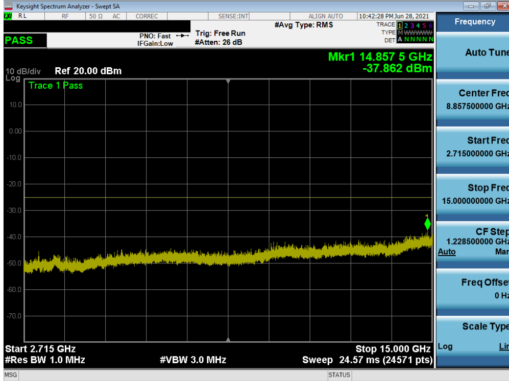
Plot 7-29. Conducted Spurious Plot (ULCA LTE B41(PC3) - 20MHz QPSK - RB Size 1, RB Offset 0 - High Channel)
