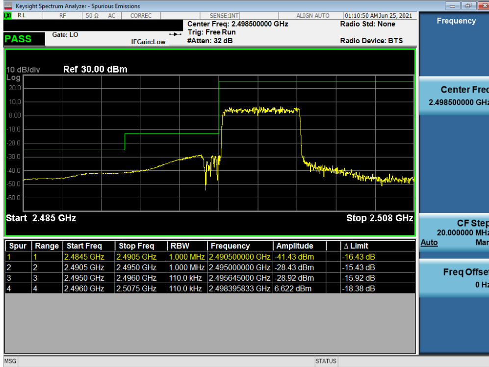
Plot 7-37. Lower ACP Plot (LTE Band 41(PC3) - 5MHz QPSK – Full RB)
