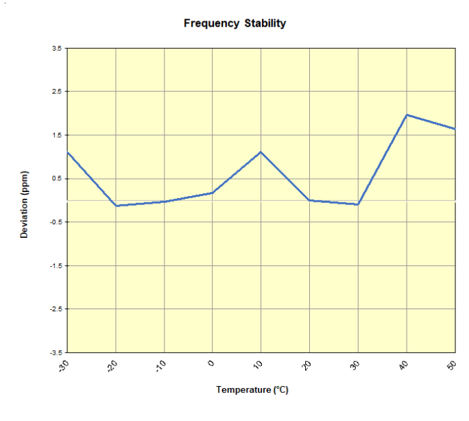
Plot 7-49. Frequency Stability Chart
