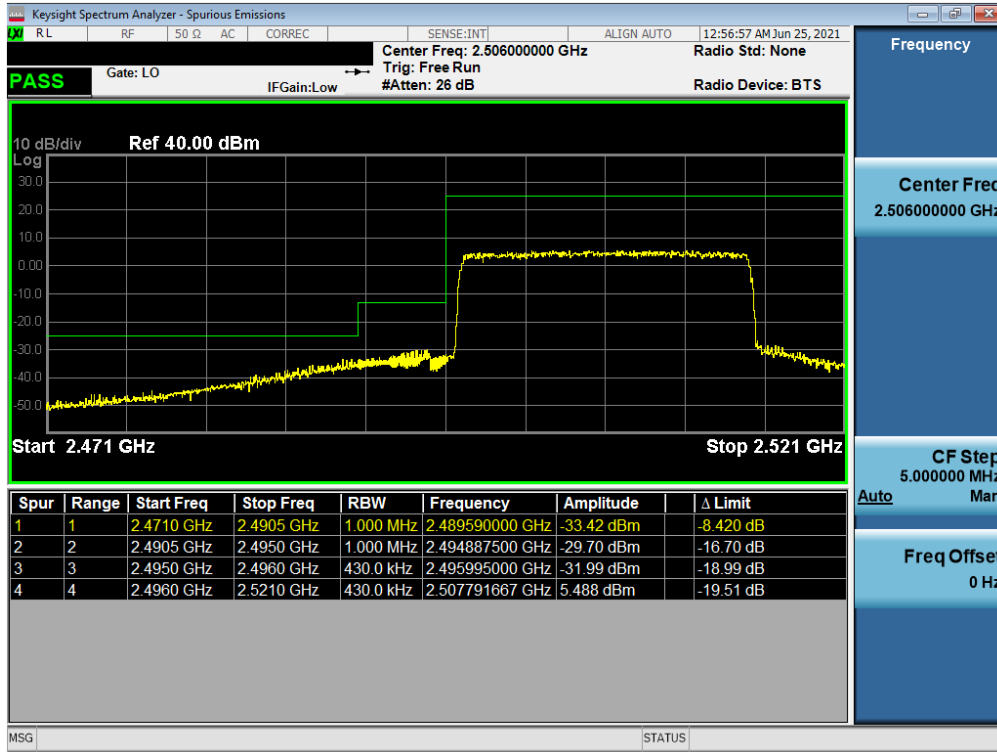
Plot 7-31. Lower ACP Plot (LTE Band 41(PC3) - 20MHz QPSK - Full RB)
