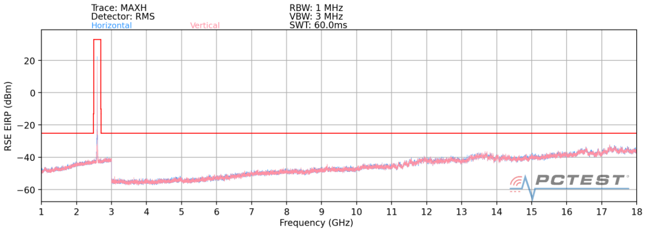
Plot 7-42. Radiated Spurious Plot (LTE Band 41(PC3))- OPEN
