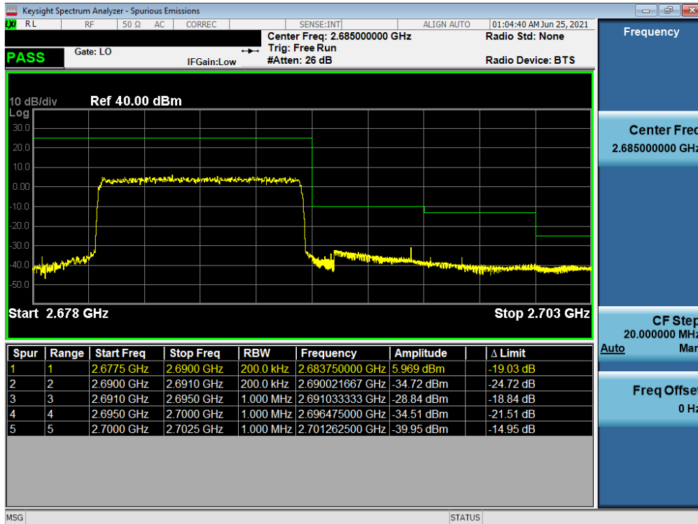
Plot 7-36. Upper ACP Plot (LTE Band 41(PC3) - 10MHz QPSK - Full RB)
