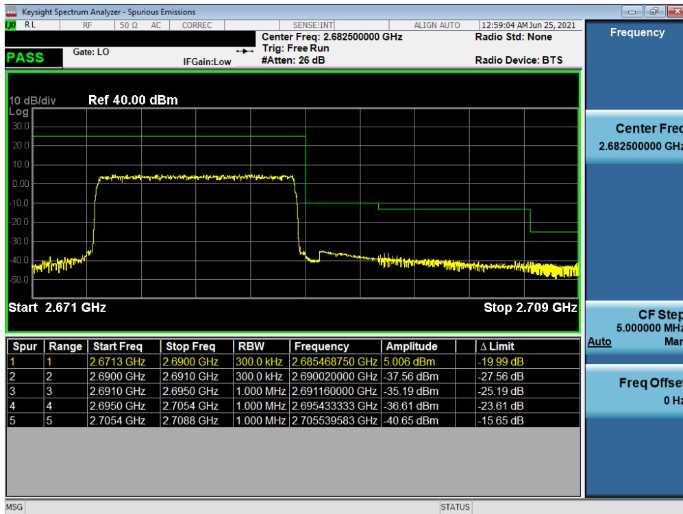
Plot 7-34. Upper ACP Plot (LTE Band 41(PC3) - 15MHz QPSK – Full RB)
