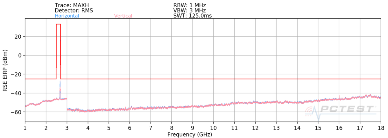
Plot 7-48. Radiated Spurious Plot (ULCA LTE B41(PC3))- High Channel- OPEN
