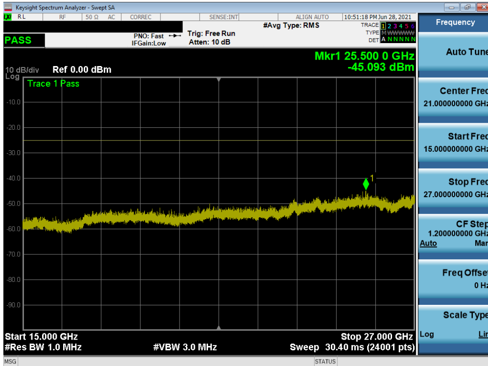
Plot 7-26. Conducted Spurious Plot (ULCA LTE B41(PC3) - 20MHz QPSK - RB Size 1, RB Offset 0 - Mid Channel)
