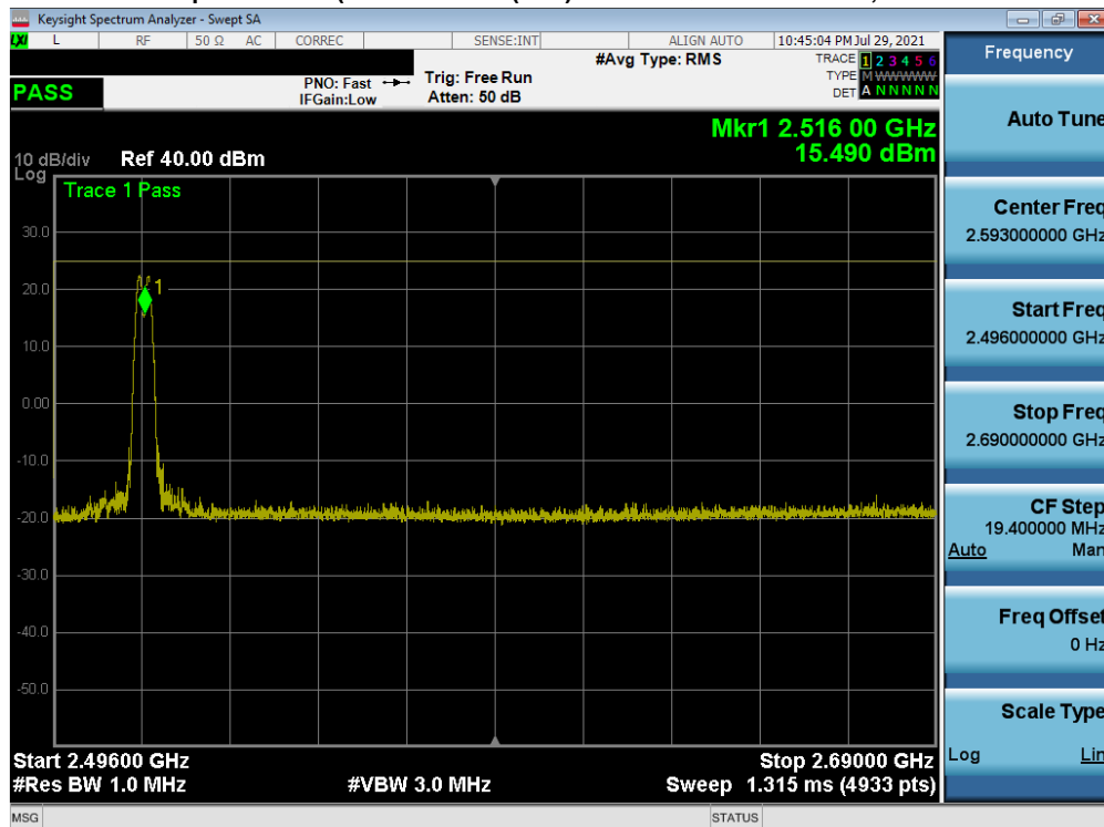
Plot 7-20. Conducted Spurious Plot (ULCA LTE B41(PC3) - 20MHz QPSK - RB Size 1, RB Offset 0 - Low Channel)
