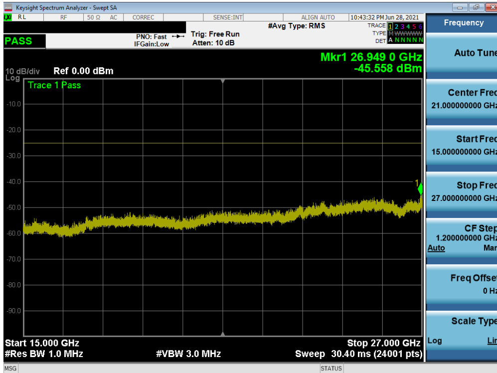
Plot 7-30. Conducted Spurious Plot (ULCA LTE B41(PC3) - 20MHz QPSK - RB Size 1, RB Offset 0 - High Channel)
