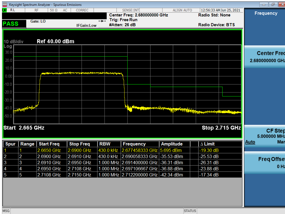
Plot 7-32. Upper ACP Plot (LTE Band 41(PC3) - 20MHz QPSK - Full RB)
