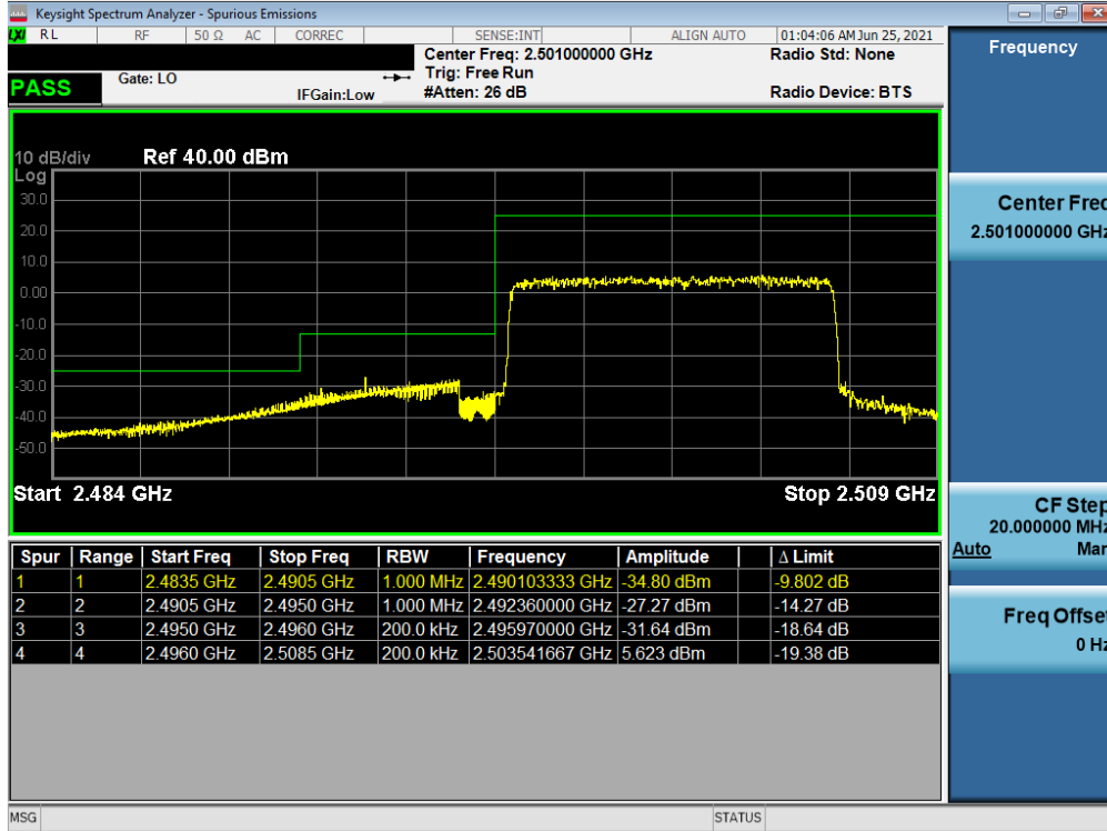
Plot 7-35. Lower ACP Plot (LTE Band 41(PC3) - 10MHz QPSK - Full RB)
