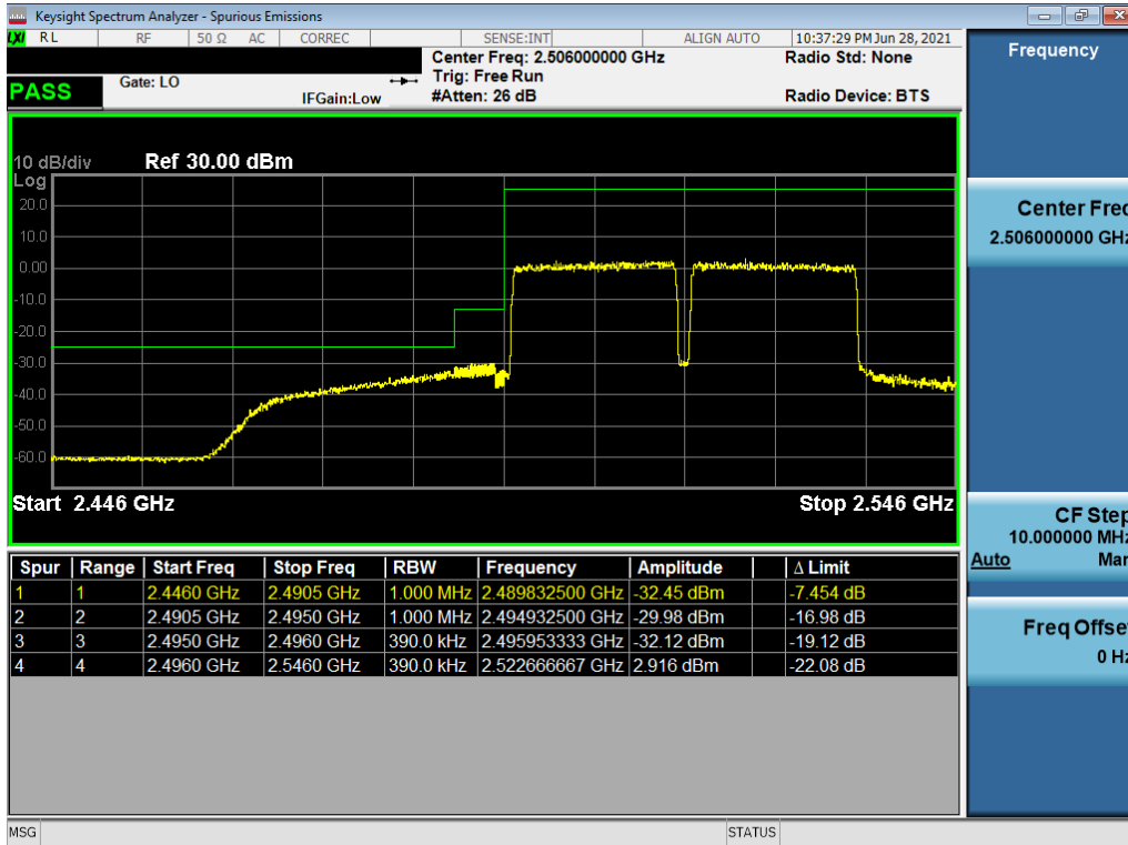
Plot 7-39. Lower ACP Plot (ULCA LTE B41(PC3) - 20MHz QPSK - Full RB - Ant1)
