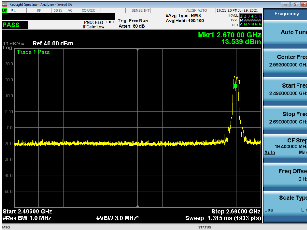
Plot 7-28. Conducted Spurious Plot (ULCA LTE B41(PC3) - 20MHz QPSK - RB Size 1, RB Offset 0 - High Channel)
