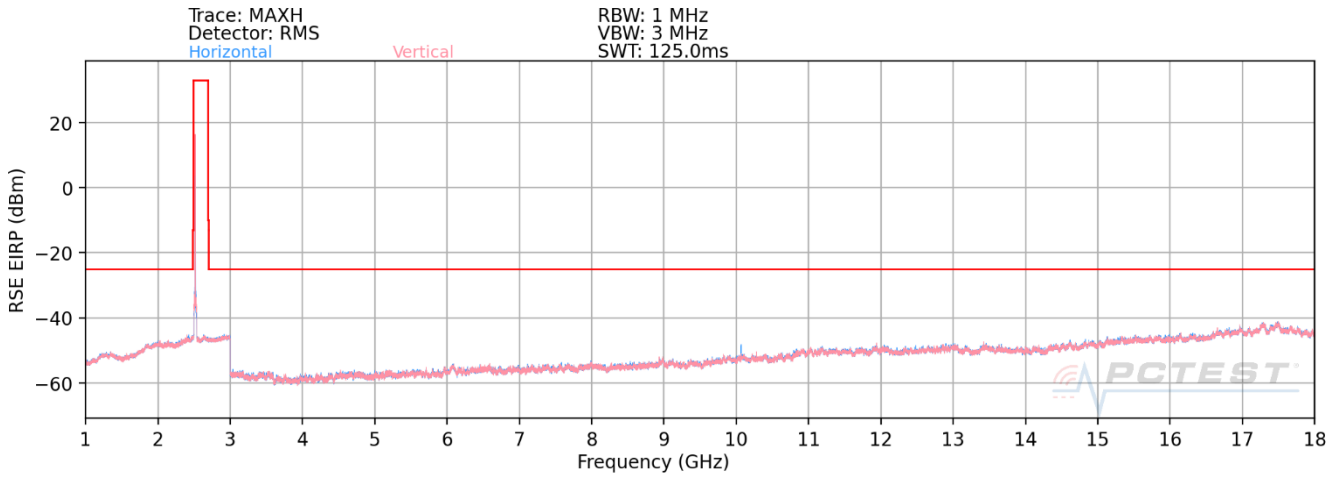
Plot 7-43. Radiated Spurious Plot (ULCA LTE B41(PC3))- Low Channel- CLOSE
