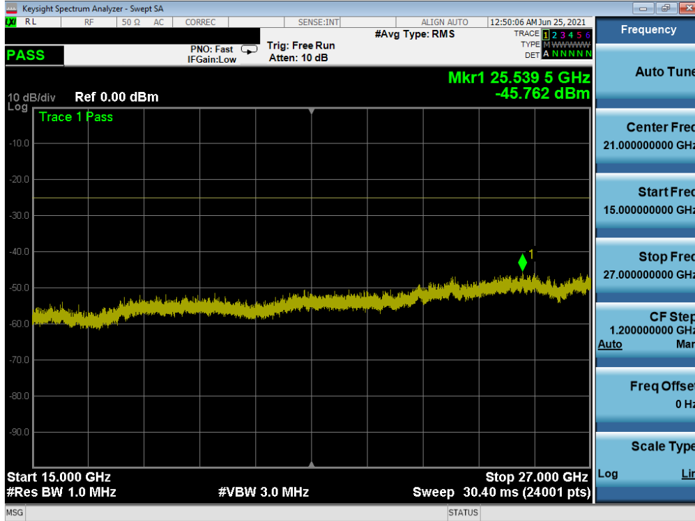
Plot 7-18. Conducted Spurious Plot (LTE Band 41(PC3) - 20MHz QPSK - RB Size 1, RB Offset 0 - High Channel)
