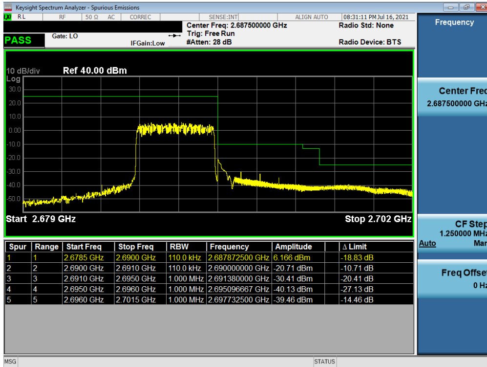
Plot 7-38. Upper ACP Plot (LTE Band 41(PC3) - 5MHz QPSK – Full RB)
