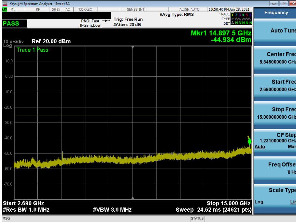
Plot 7-25. Conducted Spurious Plot (ULCA LTE B41(PC3) - 20MHz QPSK - RB Size 1, RB Offset 0 - Mid Channel)
