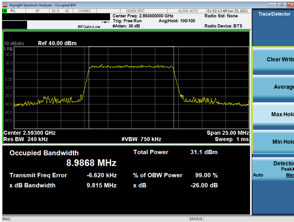
Plot 7-7. Occupied Bandwidth Plot (LTE Band 41(PC3) - 10MHz 16-QAM - Full RB)
