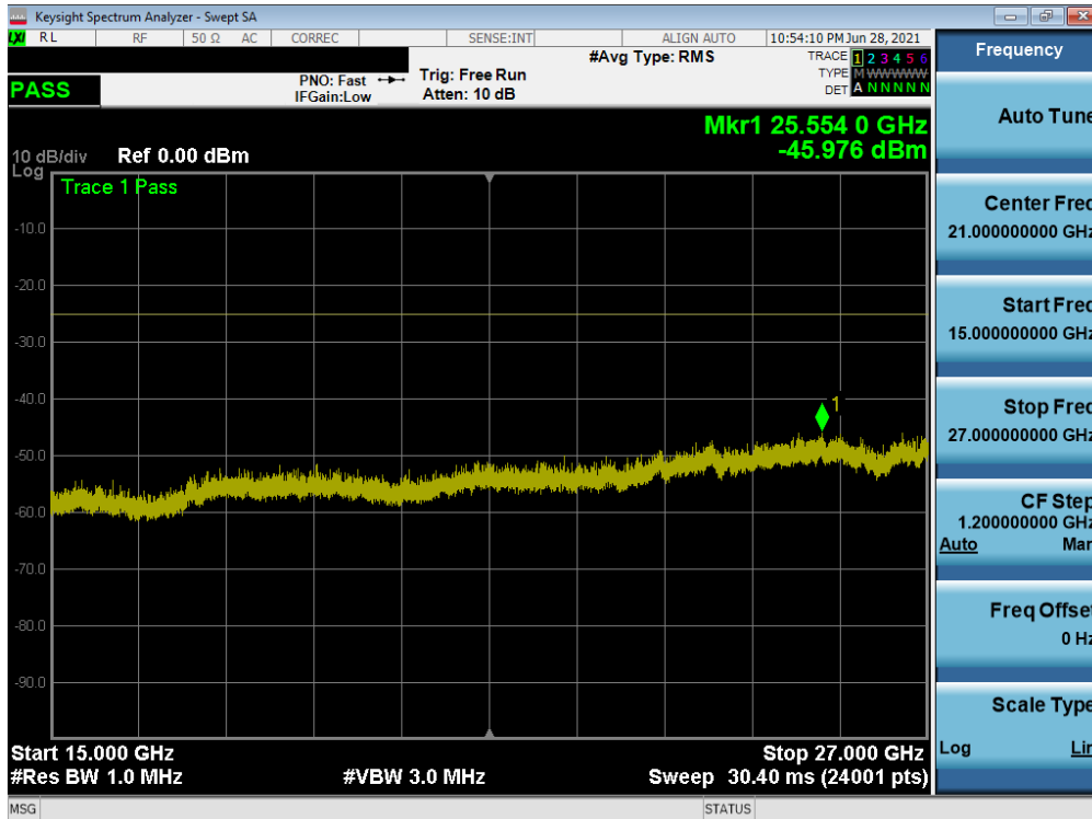
Plot 7-22. Conducted Spurious Plot (ULCA LTE B41(PC3) - 20MHz QPSK - RB Size 1, RB Offset 0 - Low Channel)
