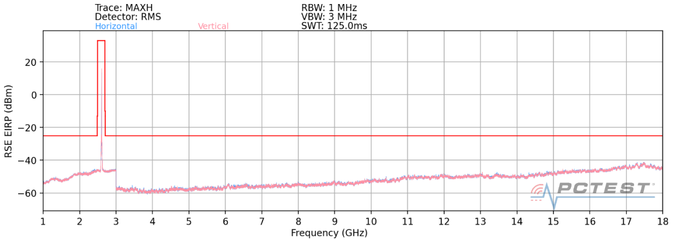
Plot 7-44. Radiated Spurious Plot (ULCA LTE B41(PC3))- Mid Channel- CLOSE
