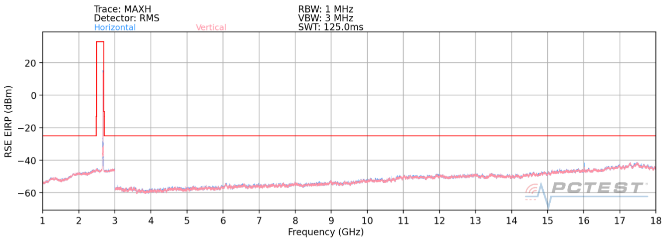
Plot 7-45. Radiated Spurious Plot (ULCA LTE B41(PC3))- High Channel- CLOSE
