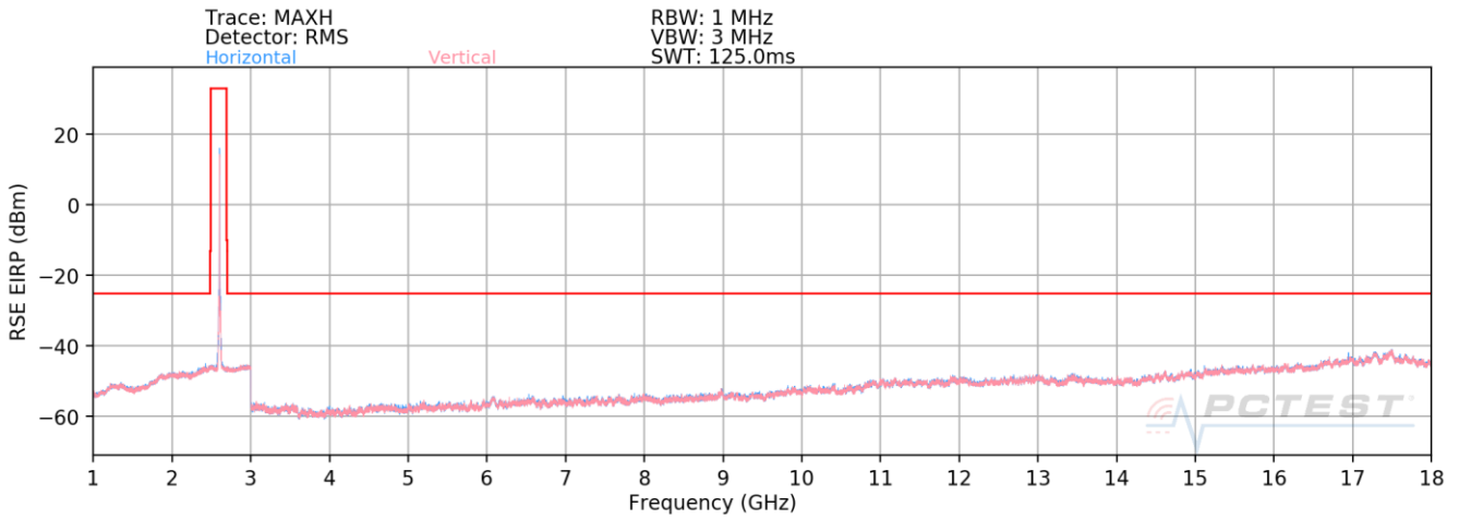
Plot 7-46. Radiated Spurious Plot (ULCA LTE B41(PC3))- Low Channel- OPEN
