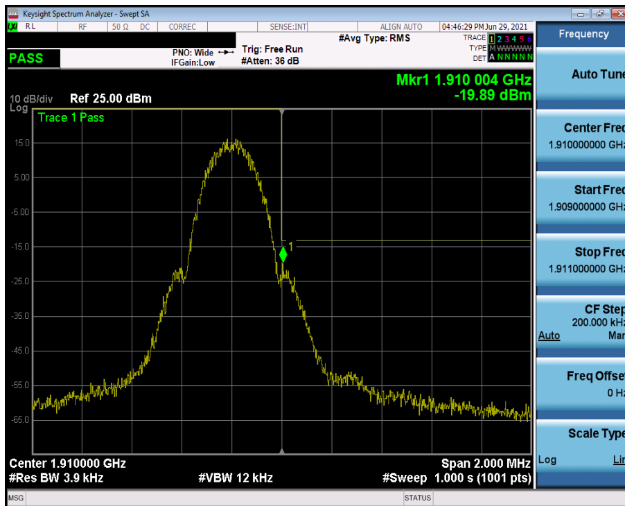
Plot 7-13. Upper Band Edge Plot (GSM PCS – Ch. 810)
