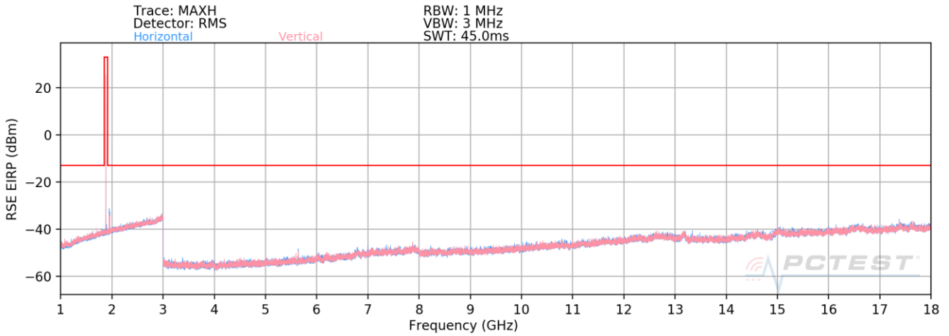
Plot 7-17. Radiated Spurious Plot (GPRS PCS)- CLOSED
