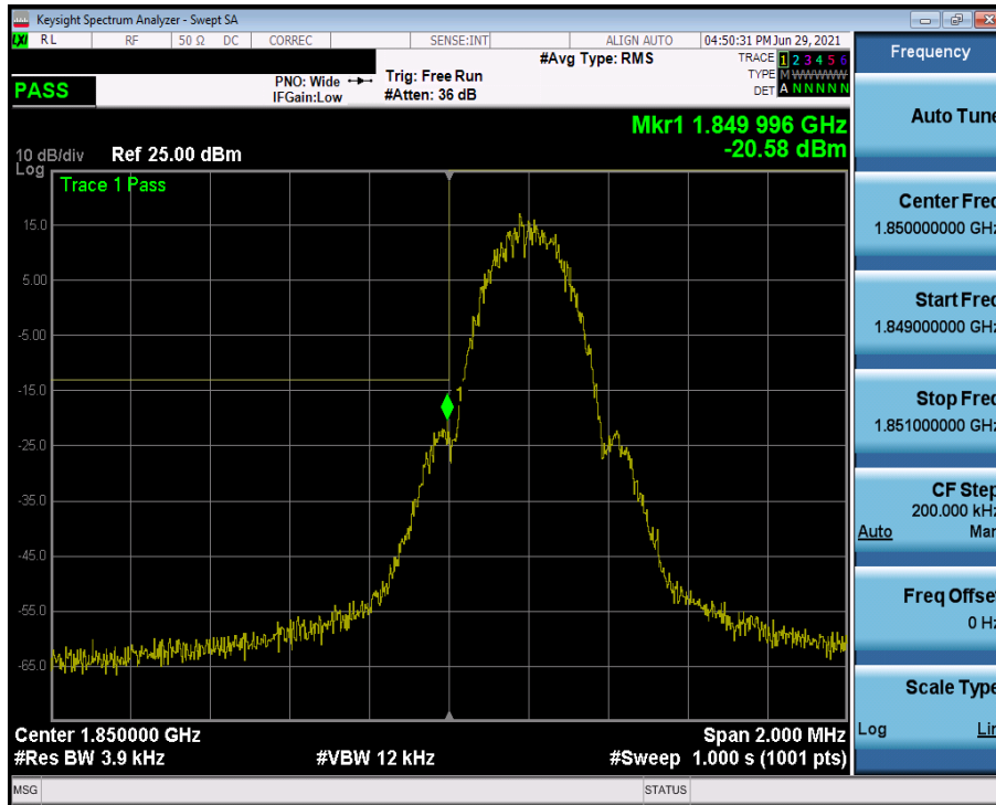
Plot 7-12. Lower Band Edge Plot (GSM PCS – Ch. 512)
