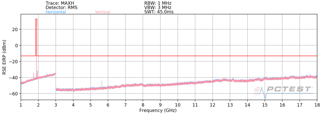
Plot 7-16. Radiated Spurious Plot (GPRS PCS)- OPEN
