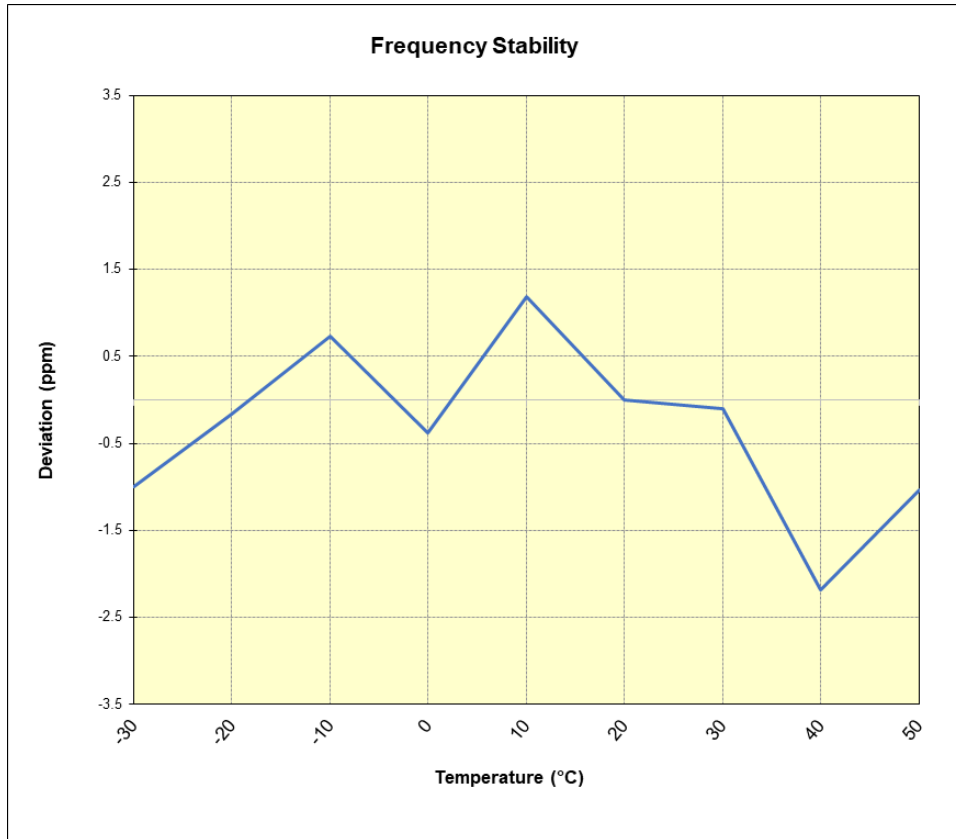
Plot 7-18. GSM/GPRS PCS Frequency Stability Chart
