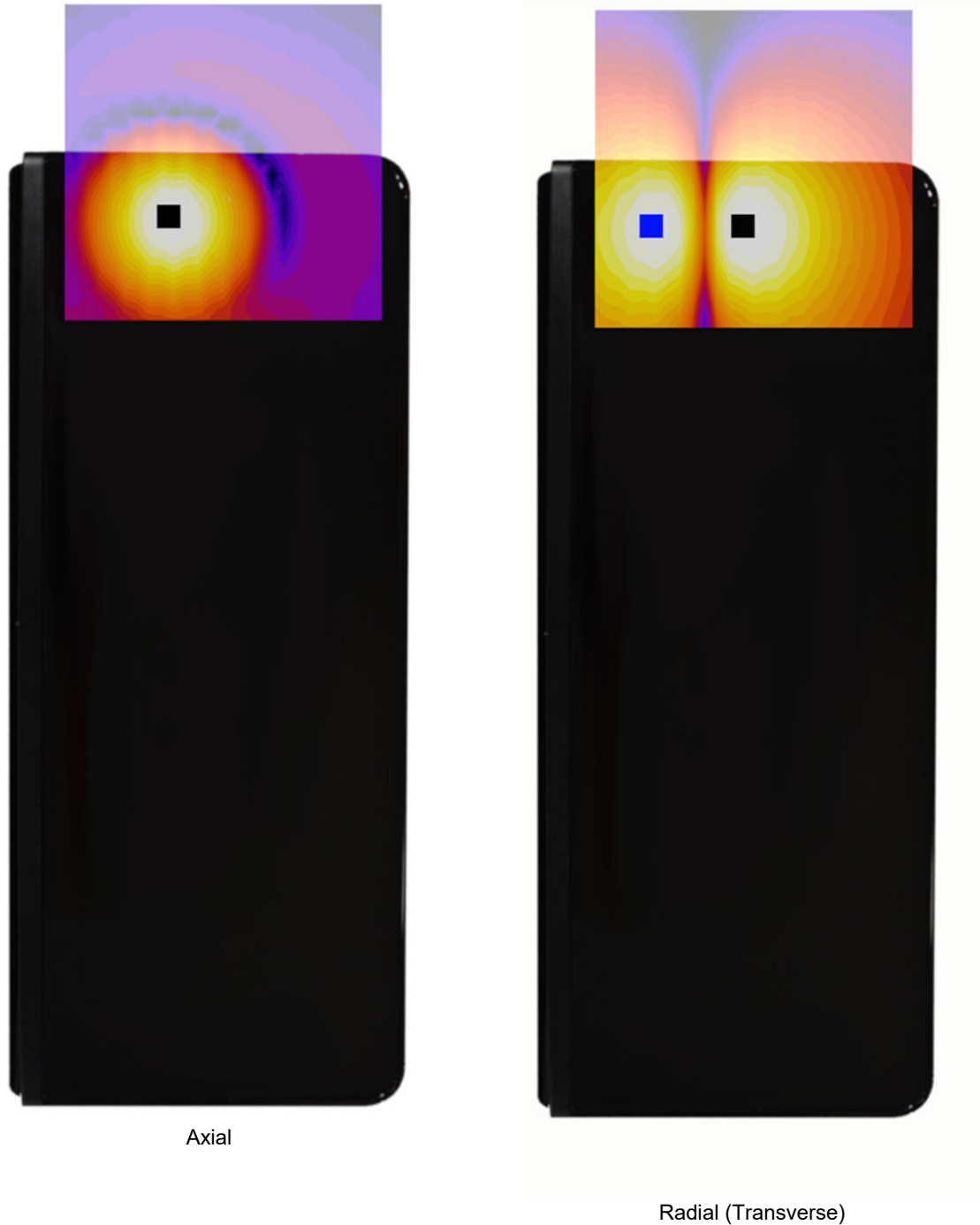
Figure 15-3 T-Coil Scan Overlay Magnetic Field Distributions
