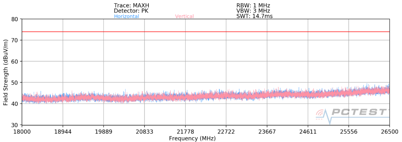
Plot 7-361. Radiated Spurious Plot above 18GHz - 26.5GHz MIMO (802.11ax) – OPEN
