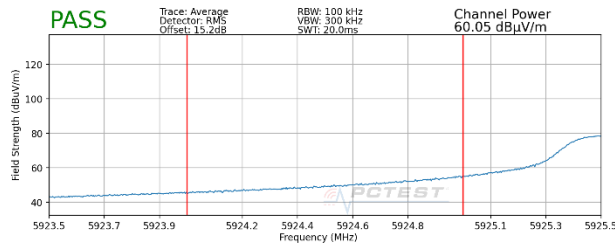
Plot 7-371. Radiated Lower Band Edge Plot MIMO (Average – UNII Band 5)
