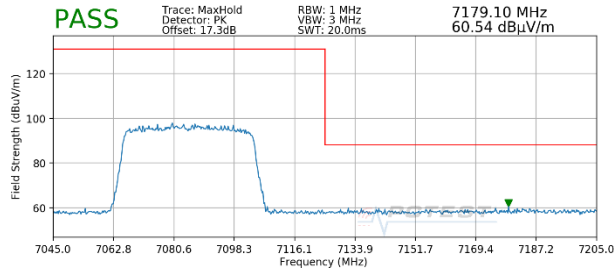
Plot 7-376. Radiated Upper Band Edge Plot MIMO (Peak – UNII Band 8)
