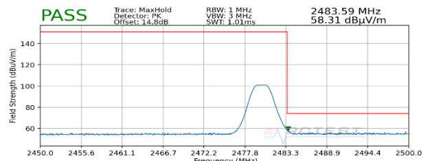
Plot 7-54. Radiated Restricted Upper Band Edge Measurement (Peak) - CLOSE
