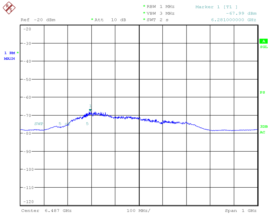
Plot 7-69. UWB Peak Power Measurement - ANT 1 - CH.5 - SP0 – HPRF
