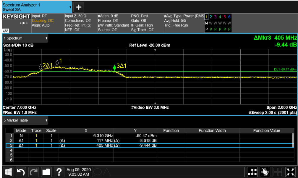
Plot 7-25. BANDWIDTH Plot – ANT1 - CH.5 – SP1 – Preamble 27
