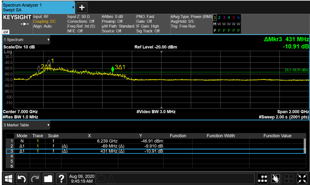
Plot 7-27. BANDWIDTH Plot – ANT2 - CH.5 - SP0 – Preamble 27
