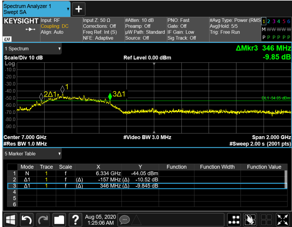
Plot 7-7. BANDWIDTH Plot - ANT1 - CH.5 - SP0 - Preamble 10
