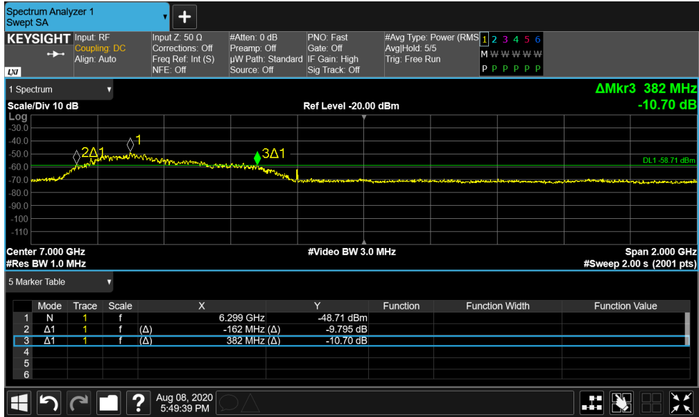
Plot 7-21. BANDWIDTH Plot – ANT2 - CH.5 - SP0 – Preamble 12
