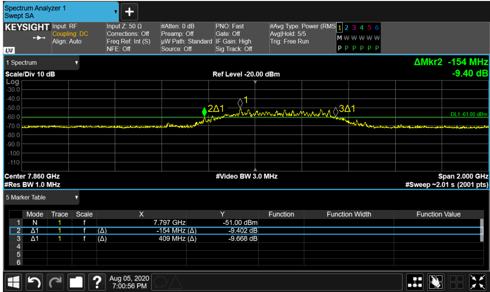
Plot 7-37. BANDWIDTH Plot - ANT1 - CH.9 – SP1 – Preamble 10
