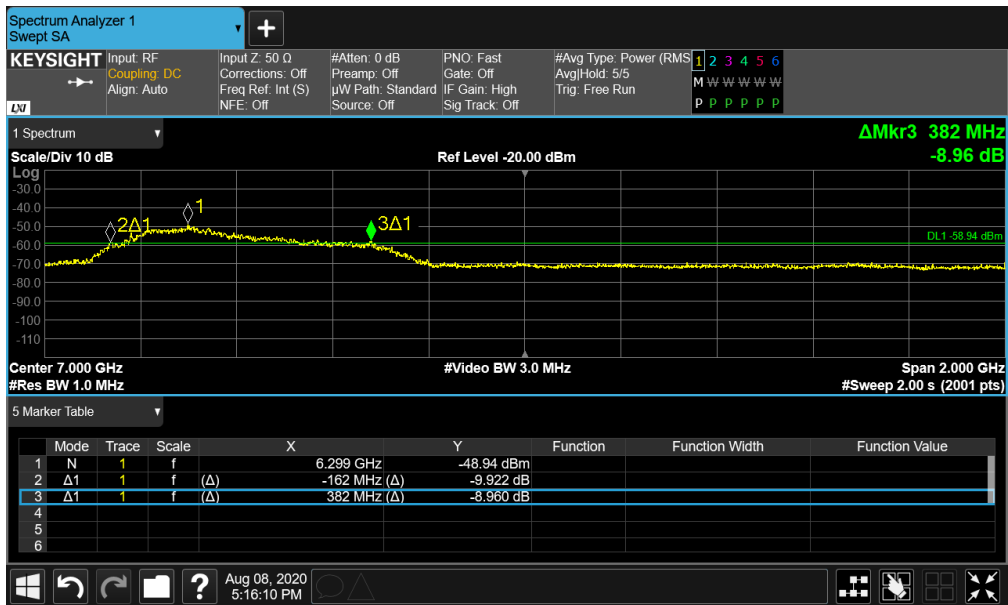
Plot 7-22. BANDWIDTH Plot – ANT2 - CH.5 – SP1 – Preamble 12
