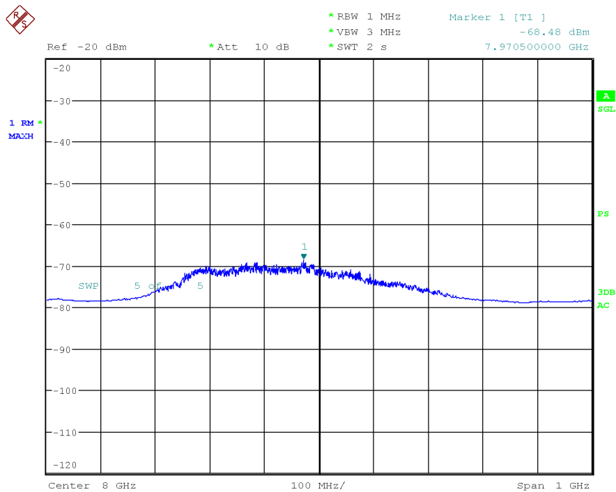
Plot 7-75. UWB Peak Power Measurement - ANT 2 - CH.9 – SP3 – HPRF
