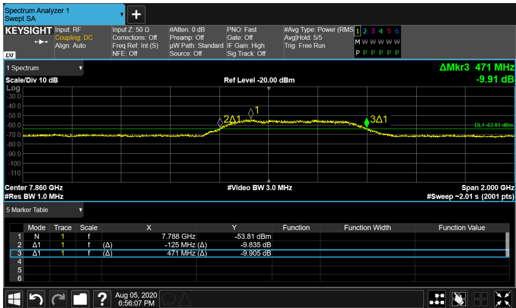
Plot 7-38. BANDWIDTH Plot - ANT1 - CH.9 – SP3 – Preamble 10
