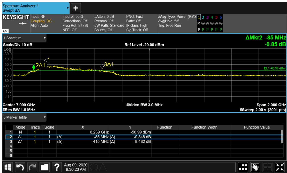
Plot 7-28. BANDWIDTH Plot – ANT2 - CH.5 – SP1 – Preamble 27
