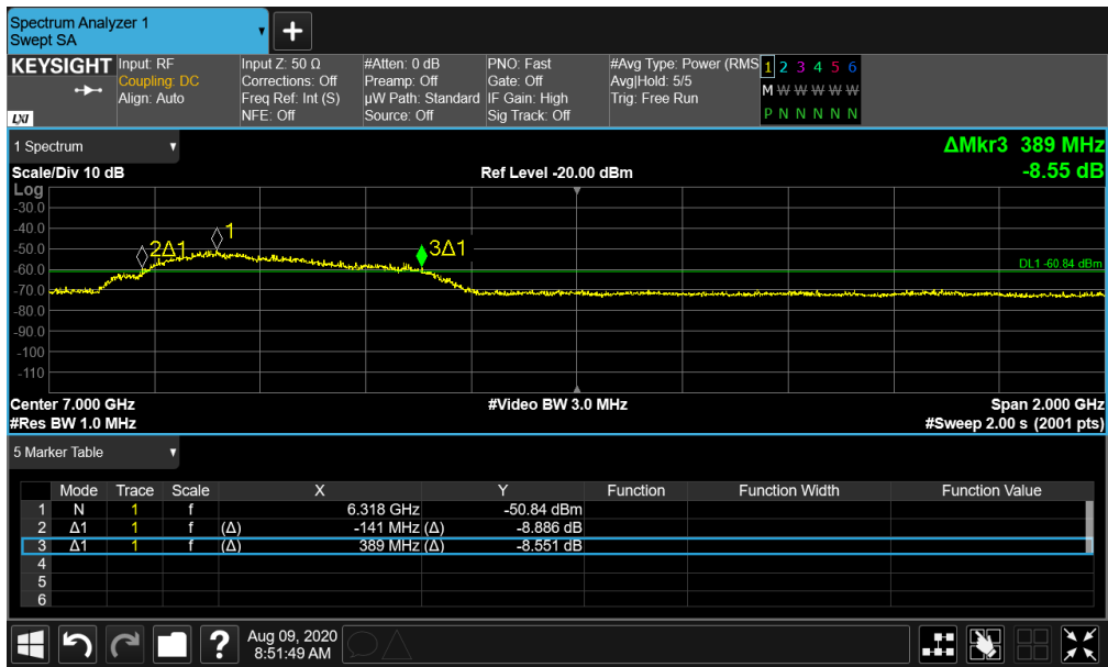
Plot 7-26. BANDWIDTH Plot – ANT1 - CH.5 – SP3 – Preamble 27
