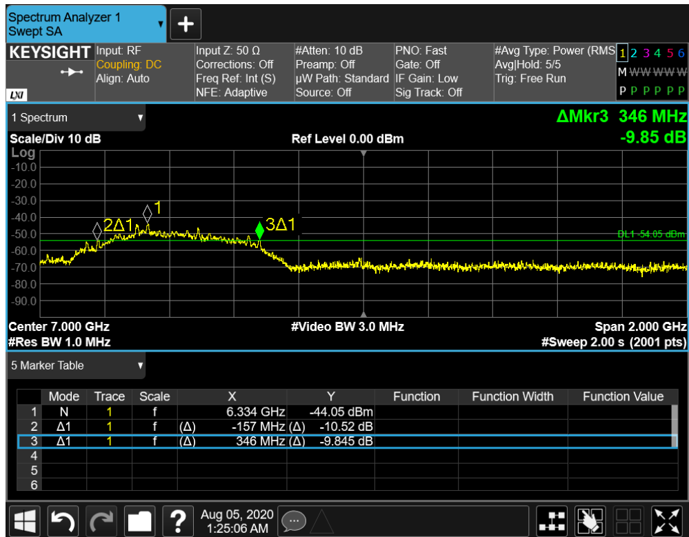
Plot 7-8. BANDWIDTH Plot - ANT1 - CH.5 - SP1 - Preamble 10
