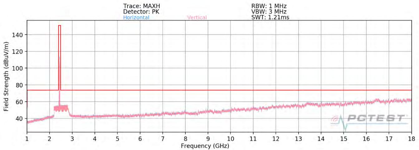
Plot 7-74. Radiated Spurious Plot above 1GHz MIMO (802.11ax OFDMA – 26 Tones – Ch. 6)
