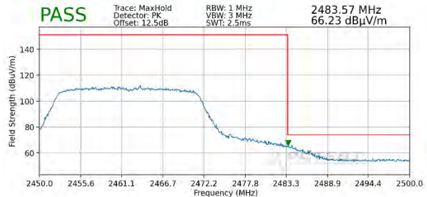
Plot 7-104. Radiated Restricted Upper Band Edge Measurement MIMO (Peak – 242 Tones)
