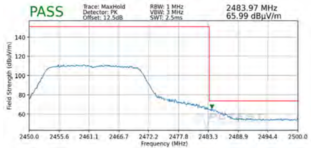
Plot 7-104. Radiated Restricted Upper Band Edge Measurement MIMO (Peak)
