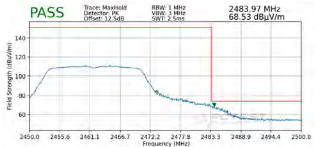
Plot 7-96. Radiated Restricted Upper Band Edge Measurement SISO ANT2 (Peak)
