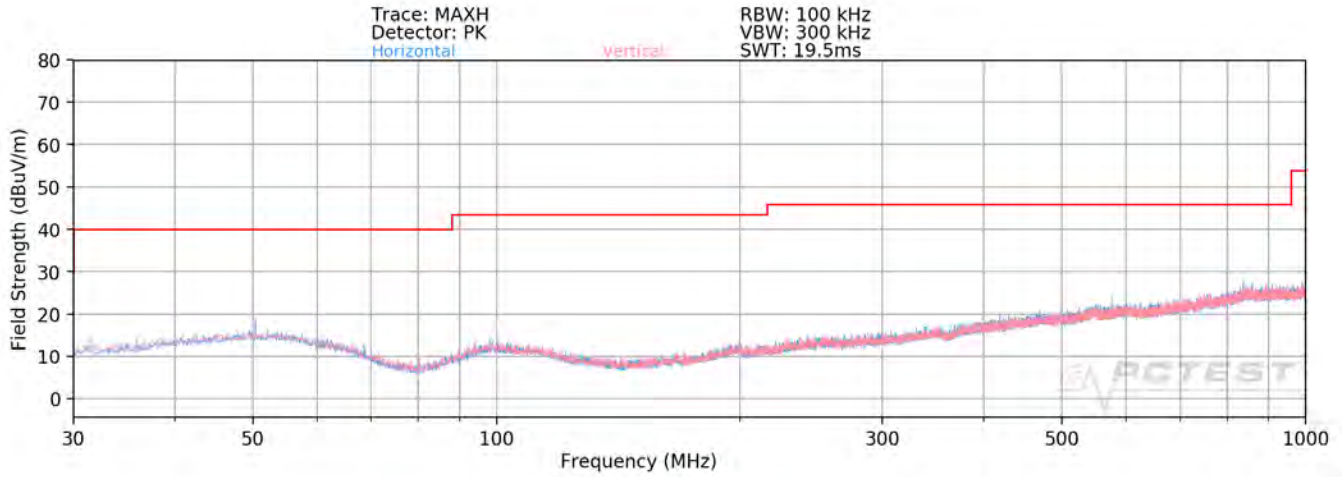
Plot 7-107. Radiated Spurious Plot below 1GHz
