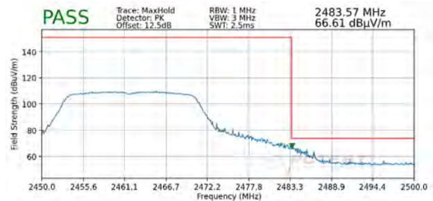
Plot 7-92. Radiated Restricted Upper Band Edge Measurement SISO ANT1 (Peak)
