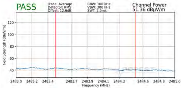
Plot 7-103. Radiated Restricted Upper Band Edge Measurement MIMO (Average)
