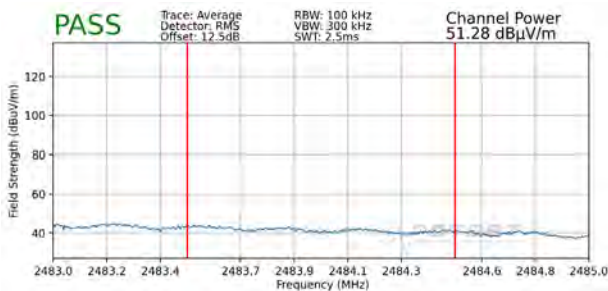
Plot 7-95. Radiated Restricted Upper Band Edge Measurement SISO ANT2 (Average)
