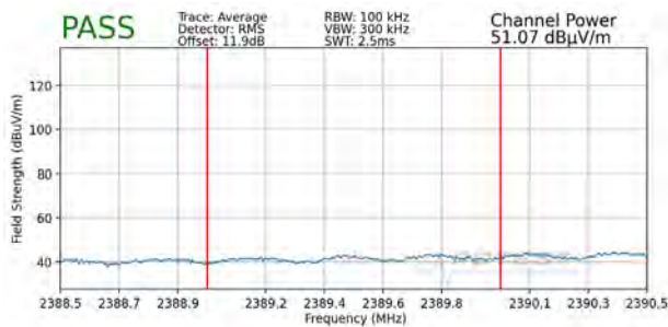
Plot 7-97. Radiated Restricted Lower Band Edge Measurement MIMO (Average)
