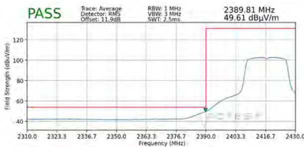
Plot 7-99. Radiated Restricted Lower Band Edge Measurement MIMO (Average)
