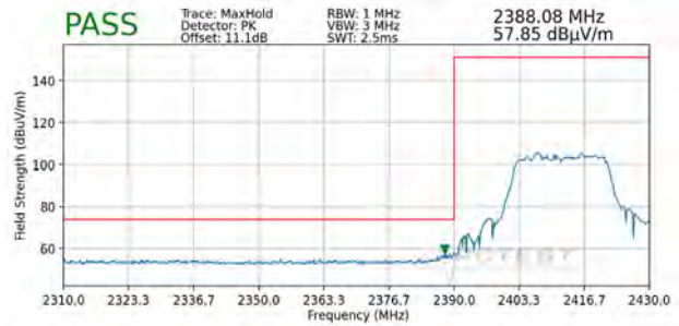
Plot 7-106. Radiated Restricted Band Edge Measurement MIMO with WCP (Peak)
