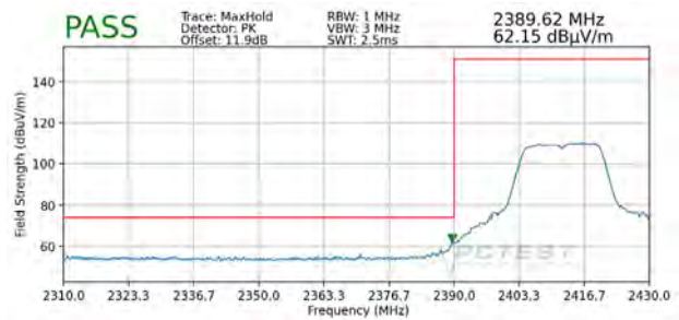
Plot 7-94. Radiated Restricted Lower Band Edge Measurement SISO ANT2 (Peak)
