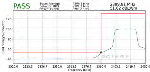
Plot 7-93. Radiated Restricted Lower Band Edge Measurement SISO ANT2 (Average)
