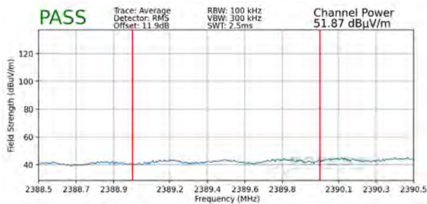
Plot 7-89. Radiated Restricted Lower Band Edge Measurement SISO ANT1 (Average)
