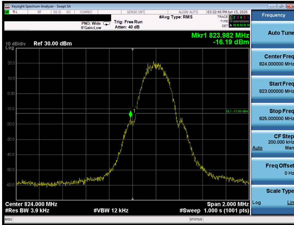
Plot 7-73. Band Edge Plot (Cellular GPRS Mode - Low Channel)
